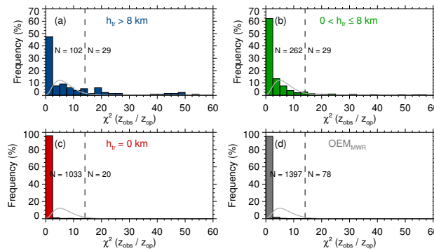
Figure 16. Histograms of the \chi^2 test for four situation given in Tab. 2. The dotted lines indicate the theoretical \chi^2 distribution with m_y degree of freedom. Dashed lines indicate the 5% threshold value of 14. The absolute number of cases below and above the threshold value is given to the left and to the right side of the dashed line, respectively.
