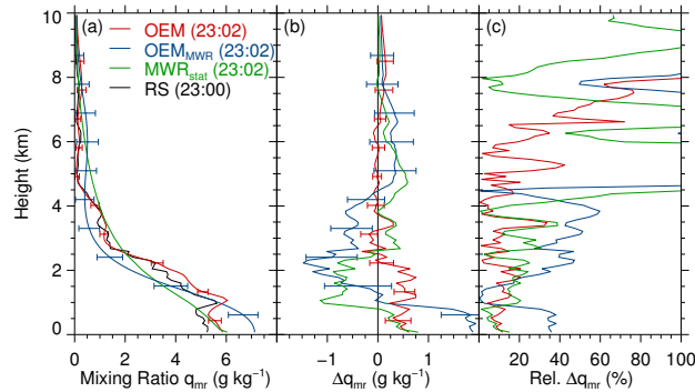
Figure 8. (a) Comparison of mixing ratio profiles on 5 May 2013 around 23:00 UTC: retrieved profile (OEM, red), retrieved profile with RS climatology as a priori ( OEM_{MWR} , blue), profile from the MWR statistical retrieval ( MWR_{stat} , green) and RS (black) as reference. Error bars are added to the optimally estimated profiles (red, blue). Absolute (b) and relative (c) difference from the reference RS.
