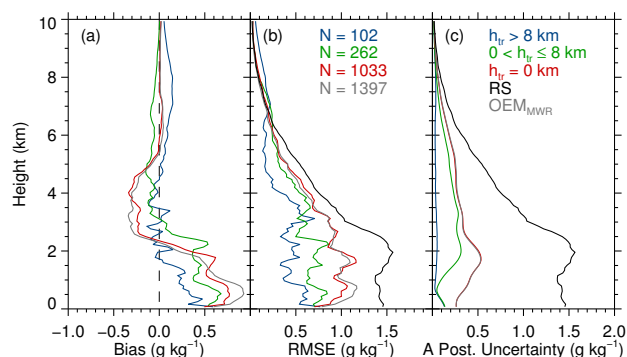
Figure 13. Statistical analysis of the synergy improvement: bias to RS (a), root mean square error (RMSE) to RS (b) and a posteriori uncertainty (c). It distinguishes four situations according to Tab. 2. The sample size is given by the numbers in the middle panel. Only profiles between RS launch time and one hour after are considered.
