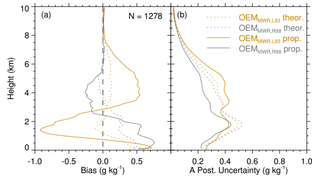
Figure 14. Bias to RS (a) and a posteriori uncertainty (b) for two different absorption codes, Rosenkranz, (R98, grey) and Liebe (L93, orange). The shown retrievals are only based on MWR but with different a priori states. On the one hand, both a priori profile and a priori uncertainty are taken from the RS climatology (theor.) and on the other hand the a priori profile is propagated (prop.) from the previous step while the uncertainty is taken from the RS climatology (red cases in the figures above). The sample size is given by the numbers. Only profiles between RS launch time and one hour after launch time are considered.
