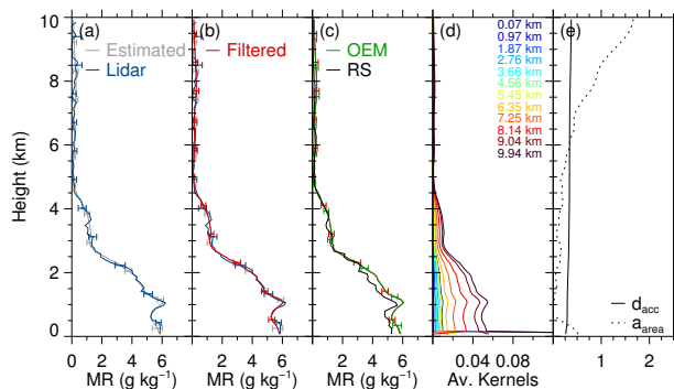
Figure 7. Overview of cloud free scene on 5 May 2013, 23:02 UTC. Mixing ratio (MR) profiles from the Raman lidar and the estimated (a), the Kalman filtered (b) and the optimally estimated state (c). Additionally, the mixing ratio of the radiosonde (RS) is shown (c). Error bars are added to the profiles at the different states of the processing. (d) Averaging kernel for a subset of ten levels indicated by the coloured numbers. (e) Accumulated degree of freedom d_{acc} (solid) and the area of the averaging kernel A_{area} (dotted).
