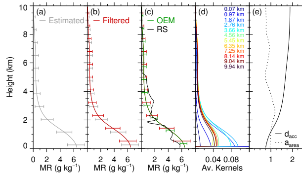
Figure 9. As Figure 7, but on 5 May 2013 07:02 UTC.
