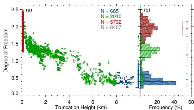
Figure 17. (a): Degree of freedom as function of truncation height for different situations introduced in Tab. 2. (b): Frequency distribution of the degree of freedom. The symbols and error bars correspond to the according mean and standard deviation, respectively. The numbers indicate the sample size of the considered profiles, full height (blue), truncated (green), no lidar (red) and OEM MWR (grey).
