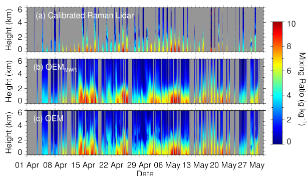
Figure 12. Three different Height-time displays of mixing ratio profiles during HOPE: (a) calibrated Raman lidar profiles, (b) optimal estimated profiles only based on MWR (and surface humidity) without any Raman lidar mixing ratio profile ( OEM_{MWR} ) and (c) optimal estimated profiles based on Kalman filtered Raman lidar mixing ratio a priori profiles (OEM).
