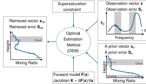
Figure 5. Illustration of the optimal estimation method. Details are given in the text.
