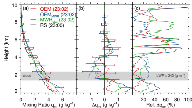
Figure 11. As Figure 8 but on 21 April 2013. The grey area indicates the cloud with an LWP of 242 \text{ g m}^{-2} .
