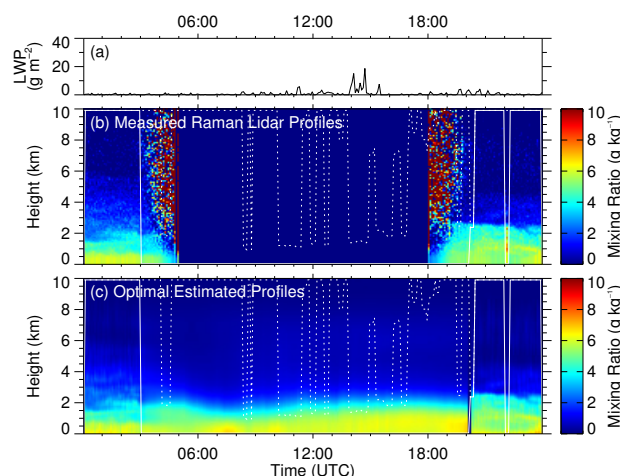
Figure 6. Overview of a mostly cloud free case on 5 May 2013. (a) liquid water path (LWP). (b) Height-time display of the mixing ratio measured by the Raman lidar. (c) Height-time display of the retrieved optimal estimated mixing ratio. The solid line indicates the height where the Raman lidar profiles are truncated. The dotted line defines the cloud base height determined by the lidar.
