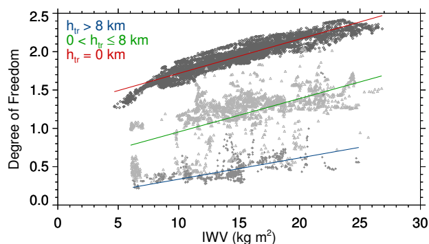
Figure 18. Degree of freedom as function of IWV for the situations introduced in Tab. 2. The lines indicate the according regression lines.
