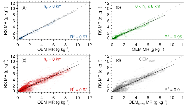
Figure 15. Comparison of optimal estimated (OEM) and radiosonde (RS) mixing ratio profiles for four situations given in Tab. 2. The black solid line indicates the regression line.
