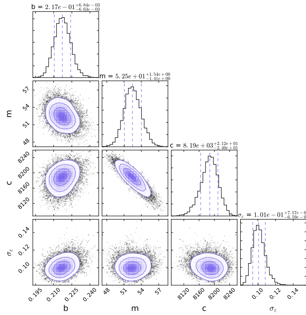
Figure A1. PCASP (low gain stage) calibration results following the new method. Shown is the resulting model parameter ensemble by analogy with Fig. 9.
