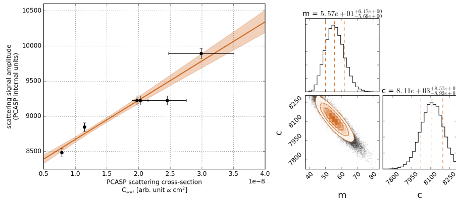
Figure A2. PCASP (low gain stage) calibration results for the approach of Rosenberg et al. (2012). The black markers in the left hand plot represent the midpoints of the scattering signal amplitude histogram modes measured for the PSL standards and the corresponding calculated mean scattering cross-sections. The error bars represent the histogram modes' half widths and scattering cross-section standard deviations respectively. The red brown solid line shows the best fit, the shaded area the range between the 16 and 84th percentiles of the fit function PDFs. To allow for direct comparison with the results of the new method the right hand plot shows the parameter solution ensemble in the same way as in Fig. A1.
