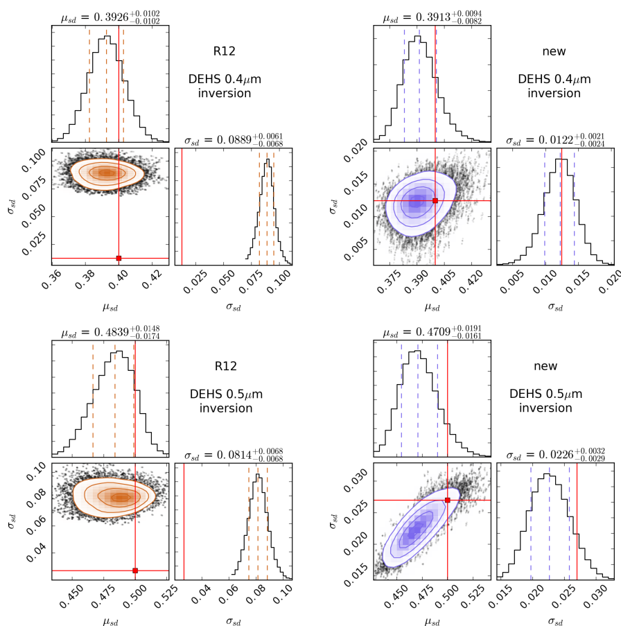
Figure 9. Parametrized size distribution retrieval results for two DEHS samples with mean diameters of 0.4 (upper row) and 0.5 \mu\text{m} (lower row) using the different approaches (columns). The theoretical (true) values for the Gaussian aerosol distributions' means and standard deviations are indicated by the red lines and markers. The dashed lines in the 1D parameter solution histograms represent the median, 16 and 84th percentiles (in \mu\text{m} ). The median values and their distances to the percentiles are noted on top of each histogram. The 2D plots show the solution scatter (black points) superposed with color-coded 2D histograms and smoothed Gaussian contours at 0.5, 1., 1.5 and 2 sigma.
