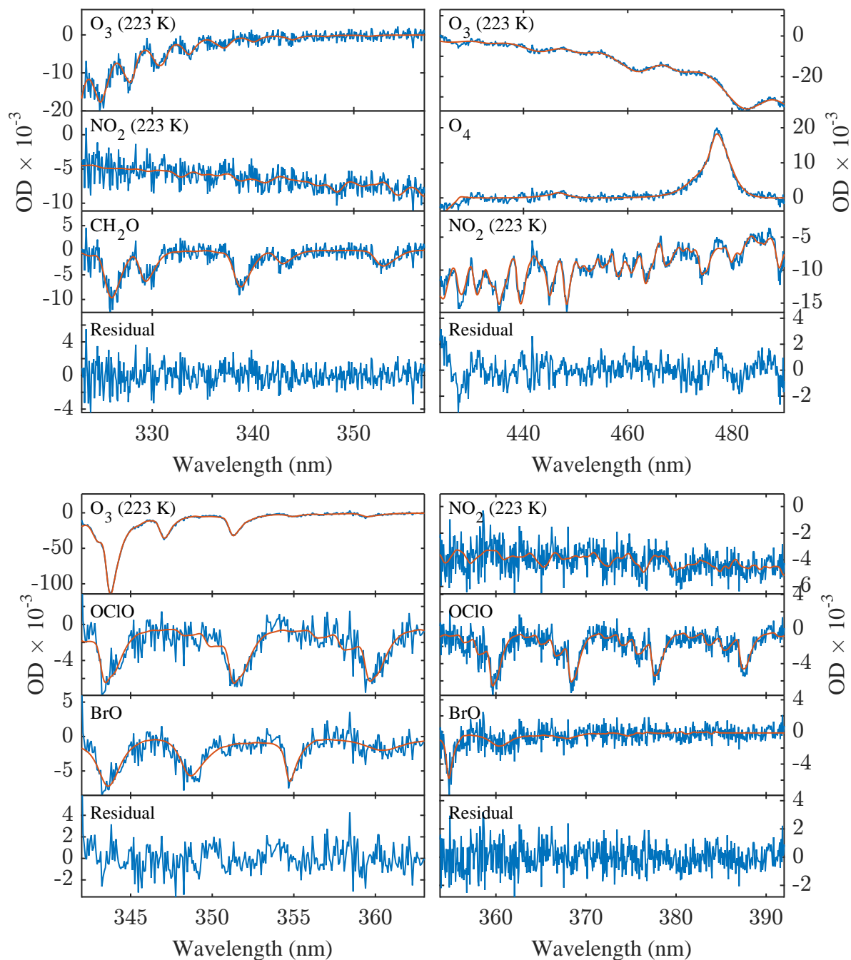
Figure 2. Sample spectral retrievals as described in section 3.1. Top left: CH 2 O ( 1.4 \times 10^{17} molec./cm 2 ) retrieval in the UV spectral range (ACRIDICON, 16 September 2014). Top right: NO 2 ( 2 \times 10^{16} molec./cm 2 ) retrieval in the visible spectral range (ESMVal, 13 September 2012). Bottom left: BrO ( 8 \times 10^{14} molec./cm 2 ) retrieval in the UV. Bottom right: OCIO ( 5.6 \times 10^{14} molec./cm 2 ) in the UV (both POLSTRACC, 31 January 2016). Fitted reference absorption cross sections are shown in red and the residual structures are shown in blue.
