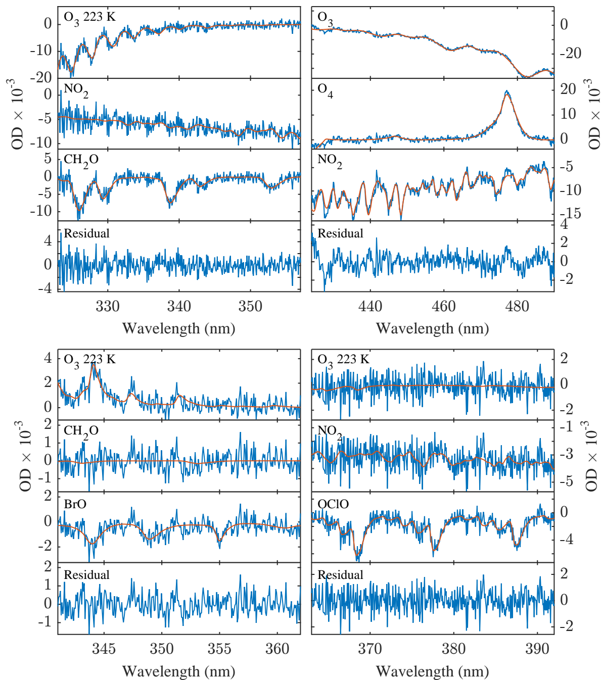
Figure 2. Sample spectral retrievals as described in section 3.1. Top left: CH 2 O retrieval in the UV spectral range. Top right: NO 2 retrieval in the visible spectral range. Bottom left: BrO retrieval in the UV. Bottom right: OCIO in the UV. Fitted reference absorption cross sections are shown in red and the residual structures are shown in blue.
