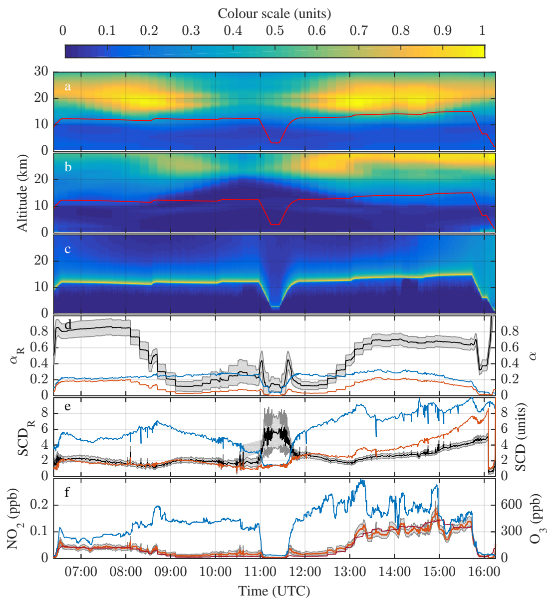
Figure 7. Illustration of NO_2 mixing ratio retrieval for the ESMVal flight on 13 September 2012 using the CCM EMAC. Panel a: EMAC predicted [O_3] curtain (colour scale \times 7.9 \cdot 10^{12} \text{ cm}^{-3} ) and aircraft altitude (red line). Panel b: EMAC predicted NO_2 curtain (colour scale \times 2.9 \cdot 10^9 \text{ cm}^{-3} ) and aircraft altitude (red line). Panel c: Box-AMFs calculated by the RTM McArtim (colour scale \times \log(217) ). Panel d: Calculated \alpha_{O_3} (blue) and \alpha_{NO_2} (red) as well as \alpha_R (black line) and its uncertainty range (grey shaded area). Panel e: Retrieved SCD_{O_3} (blue, scale divided by 9.0 \times 10^{20} ) and SCD_{NO_2} (red, scale divided by 3.4 \times 10^{17} ) as well as SCD_R (black line, scale multiplied by 10^4 ) and its uncertainty range (grey shaded area). Panel f: Retrieved [NO_2]_{O_3} (light red line) and its uncertainty range (grey shaded area) together with in situ measured O_3 (blue line). The dark red line shows the NO_2 mixing ratio predicted by the EMAC model.
