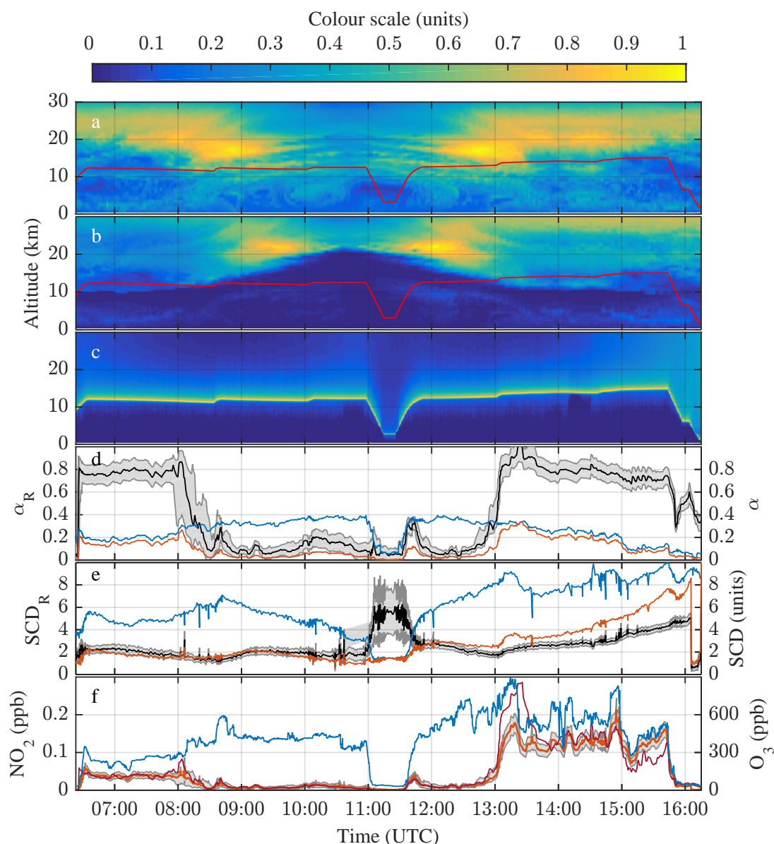
Figure 3. Illustration of NO_2 mixing ratio retrieval for the ESMVal flight on 13 September 2012 using the CTM CLaMS. Panel a: CLaMS predicted [O_3] curtain (colour scale \times 7.9 \cdot 10^{12} \text{ cm}^{-3} ) and aircraft altitude (red line). Panel b: CLaMS predicted [NO_2] curtain (colour scale \times 2.9 \cdot 10^9 \text{ cm}^{-3} ) and aircraft altitude (red line). Panel c: BoxAMFs calculated by the RTM McArtim (colour scale \times \log(217) ). Panel d: Calculated \alpha_{O_3} (blue) and \alpha_{NO_2} (red) as well as \alpha_R (black line) and its uncertainty range (grey shaded area). Panel e: Retrieved SCD_{O_3} (blue, scale divided by 9.0 \times 10^{20} ) and SCD_{NO_2} (red, scale divided by 3.4 \times 10^{17} ) as well as SCD_R (black line, scale multiplied by 10^4 ) and its uncertainty range (grey shaded area). Panel f: Retrieved [NO_2]_{O_3} (light red line) and its uncertainty range (grey shaded area) together with in situ measured O_3 (blue line). The dark red line shows the NO_2 mixing ratios predicted by the CLaMS model.
