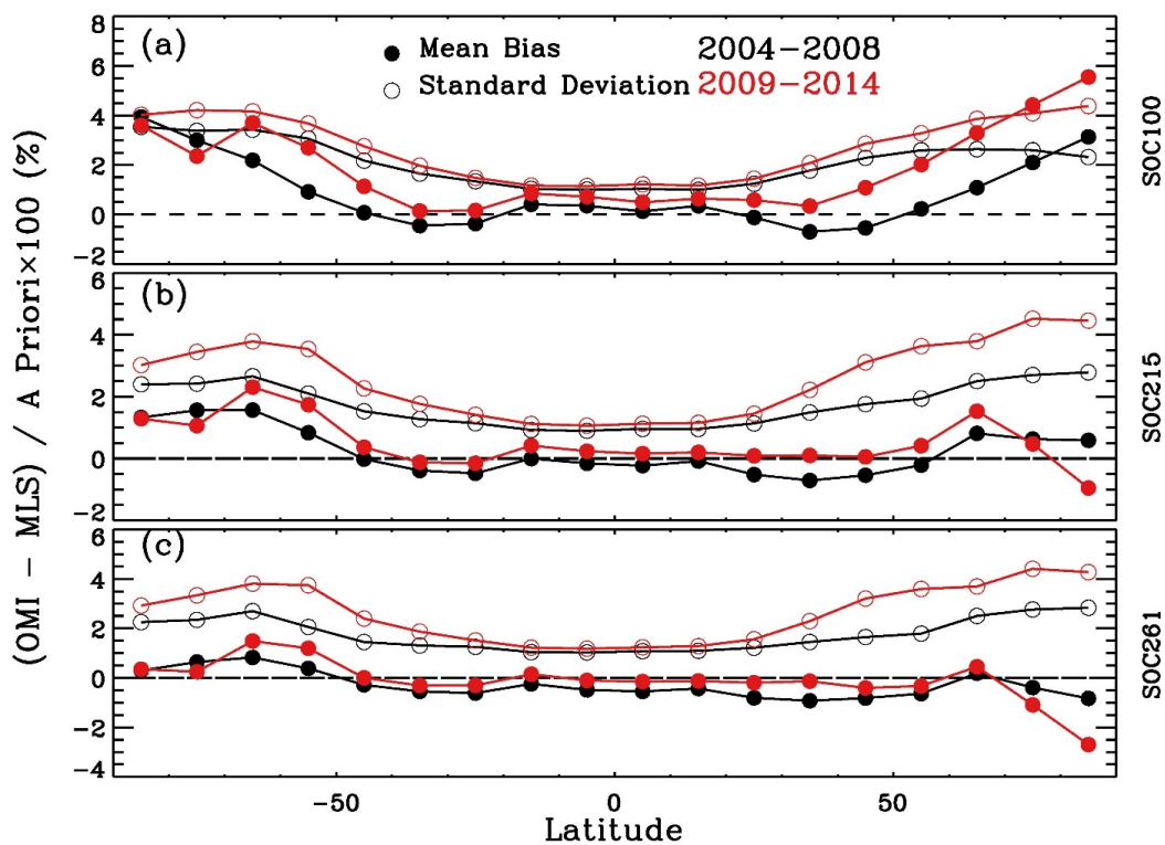
Figure 7. Mean biases (solid circles) and standard deviations (open circles) of the differences between OMI and MLS stratospheric ozone columns (SOCs) above 100 hPa (top), 215 hPa (middle) and 261 hPa (bottom) as a function of latitude, during 2004-2008 (black) and 2009-2014 (red).
