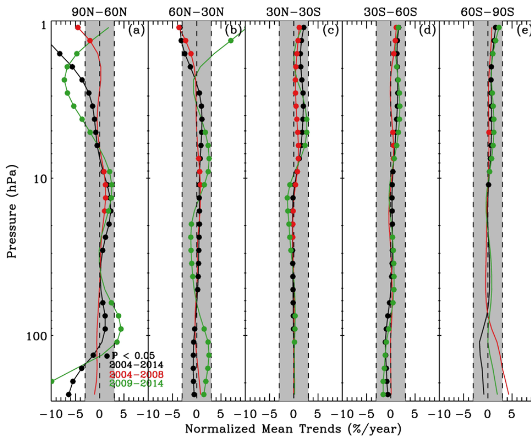
Figure 9. Linear regression trends of relative OMI-MLS biases as a function of altitude for five latitudes bands during three time periods: 2004-2014 (black), 2004-2008 (red) and 2009-2014 (green). Solid circles indicate significant trends (with P value less than 0.05).
