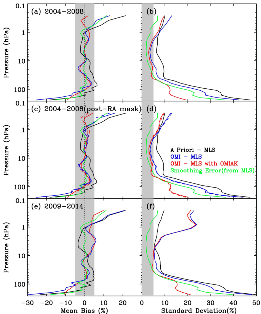
Figure 3. (left) Global mean biases at each MLS layer and (right) corresponding standard deviations of the differences between OMI and MLS profiles from 0.22 -261 hPa in (top) 2004-2008, (middle) 2004-2008 with post-RA mask and (bottom) 2009-2014, respectively. The black/blue lines compare a priori/OMI retrievals with original MLS profiles. The red lines compare OMI retrievals with MLS profiles after applying OMI Averaging Kernels (AKs). The green lines represent OMI smoothing errors estimated by assuming MLS data as the truth. For contrast, the comparisons of OMI and MLS data based on the ideal collocation criteria in 2004-2008 are plotted in blue and red dashed lines in the middle panels.
