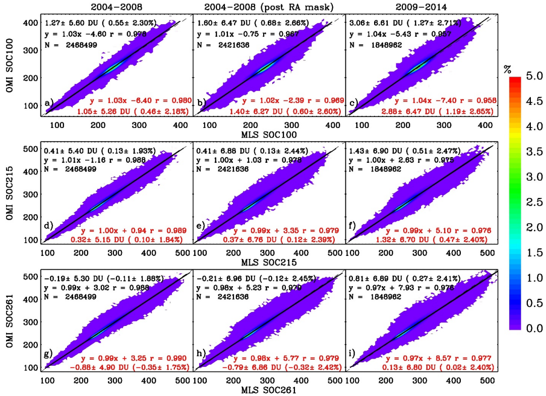
5 Figure 6. Scattering density plots of OMI and MLS stratospheric ozone columns above 100, 215 and 261 hPa (i.e., SOC100, SOC 215 and SOC261), respectively, from the top to bottom panels, during 2004-2008 (left), 2004-2008 with post-RA mask (middle column), and 2009-2014 (right). OMI averaging kernels (AKs) are not applied to MLS data. The comparison statistics of OMI-MLS SOC are shown in black including mean biases, standard deviations, relative mean biases and standard deviations, correlation coefficients, linear regressions and the number of OMI-MLS pairs. Comparison statistics with OMI AKs applied to MLS data are also provided in red.
