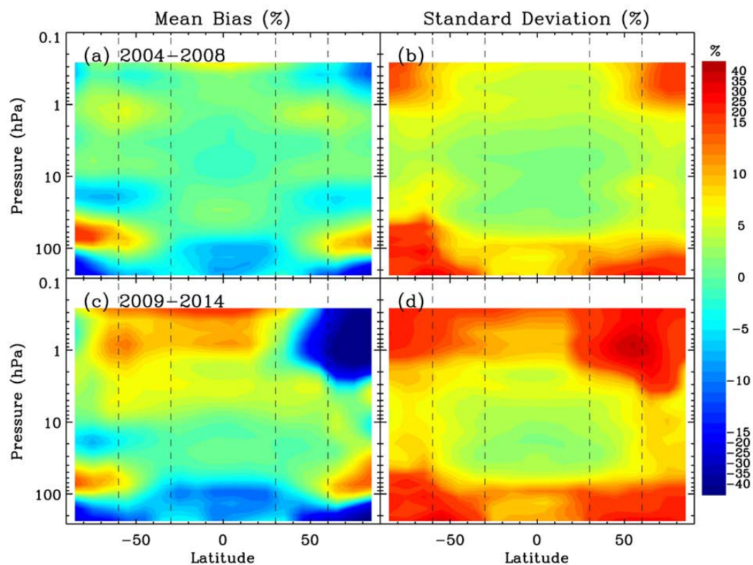
Figure 4. (left) Mean OMI/MLS ozone profile biases and (right) corresponding standard deviations as a function of latitudes in (top) 2004-2008 and (bottom) 2009-2014, respectively. OMI averaging kernels are applied to MLS data.
