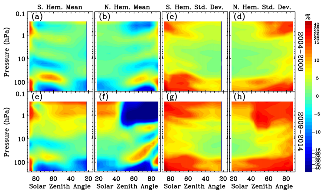
Figure 5. Similar to Figure 4, but as a function of solar zenith angles for South and North Hemispheres, respectively.
