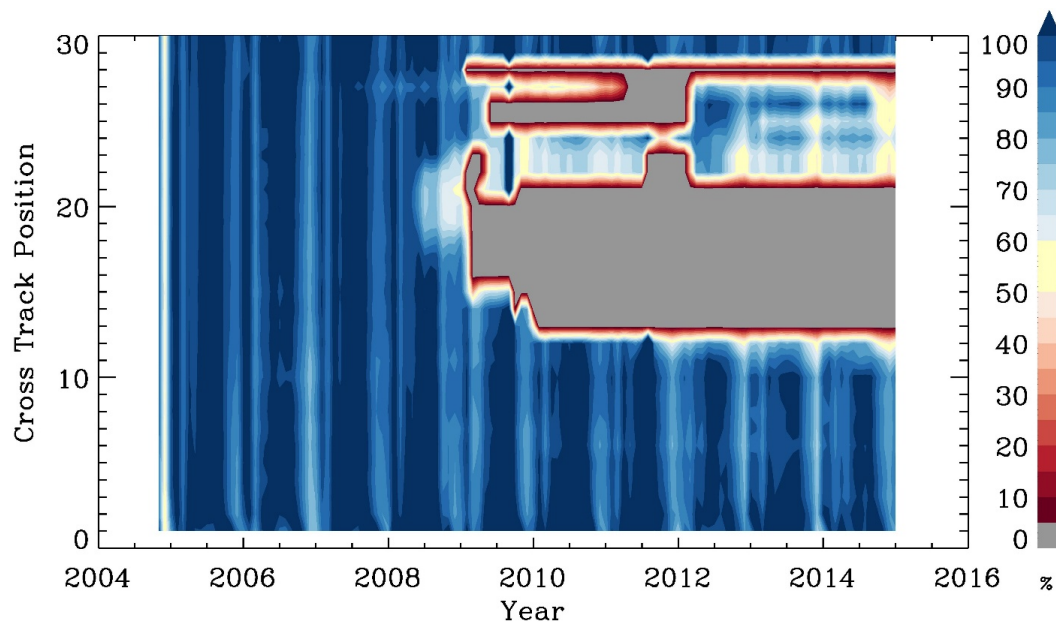
Figure 1. The monthly mean number of OMI retrievals at each cross-track position from October 2004 through December 2014, relative to the corresponding monthly mean number of OMI retrievals in January 2005, i.e. at the beginning of OMI operation.
