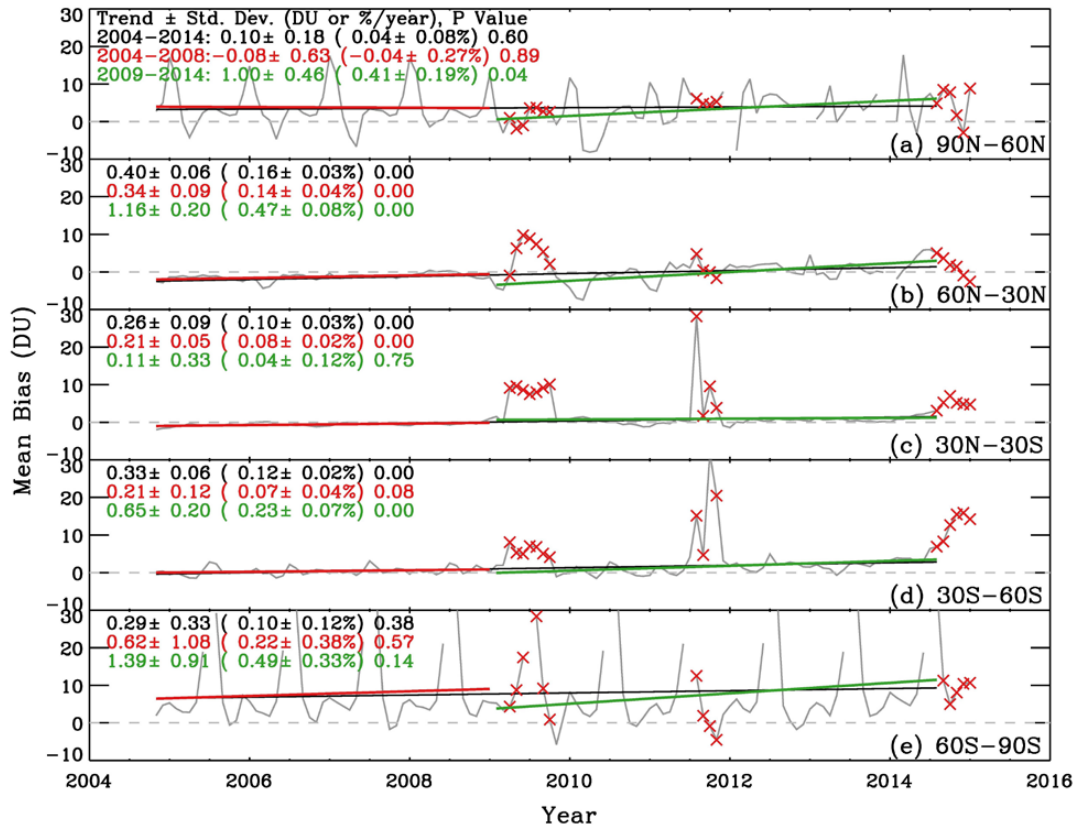
5 Figure 10. Monthly mean biases of OMI-MLS stratospheric ozone columns with pressure less than 215 hPa are plotted in solid gray lines for five different latitude ranges. The corresponding linear trends in 2004-2014, 2004-2008 and 2009-2014 are shown in black, red and green lines, respectively. The red cross signs indicate the periods when OMI has unusually large SOC errors likely due to row anomaly or other unknown issues; the values during these periods are not included in our trend calculations. The legends show linear trends in both DU/year and %/year and the corresponding P values.
