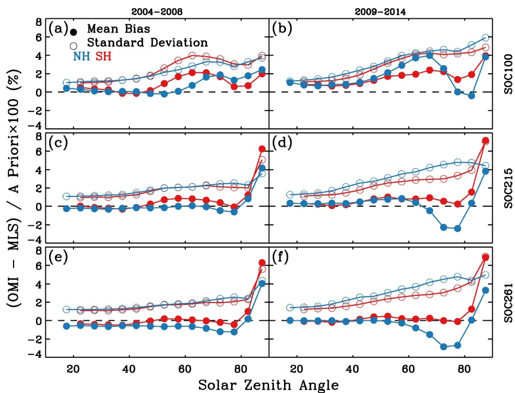
Figure 8. Mean biases (solid circles) and standard deviations (open circles) of the differences between OMI and MLS stratospheric ozone columns (SOCs) above 100 hPa (top), 215 hPa (middle) and 261 hPa (bottom) as a function of solar zenith angle for Northern Hemisphere (blue) and Southern Hemisphere (red) during 2004-2008 (left) and 2009-2014 (right).
