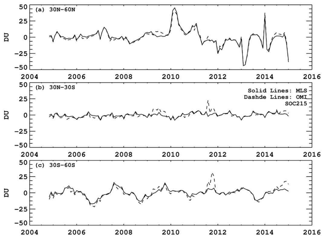
Figure 2. Deseasonalized time series of monthly mean MLS (solid lines) and OMI (dashed lines) Stratospheric Ozone Columns down to 215 hPa (SOC215s) in (a) 30°N-60°N, (b) 30°N-30°S and (c) 60°S-30°S, respectively.
