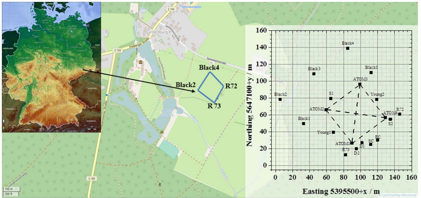
5 Figure 1. Map of Grillenburg (middle), meadow in light green, Tharandt Forest in dark green, area under investigation is marked by the blue rectangle (map Germany, 2017; map Grillenburg, 2017; see References) and scheme of area under investigation with location of several devices and auxiliary equipment: ATOM1-4 (4 masts for travel-time tomography A-TOM), dashed lines mark acoustic paths, R72/73 (2 Bruker Rapid, passive OP-FTIR), D1/2 and S1/2 (2 Bruker EM27, active OP-FTIR with source and detector), Young1/2 (2 masts, each equipped with 2 ultrasonic anemometers), Black1-5 (5 black screens for passive OP-FTIR), EC tower, SC soil respiration chamber measurements.
