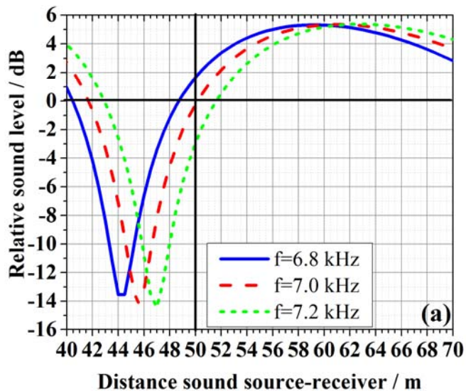
Figure 8. Relative sound level depending on the distance and on the sound frequency for a grassland surface. The height of the acoustic devices above ground is 1.5 m (a) and 3.0 m (b), respectively.
