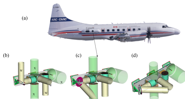
Figure 2. The NRC Airborne W- and X-band (NAWX) radar installation inside the starboard blister radome mounted on the Convair 580. The aft antenna beam can be redirected from nadir and up to 50^\circ forward along the flight direction.
