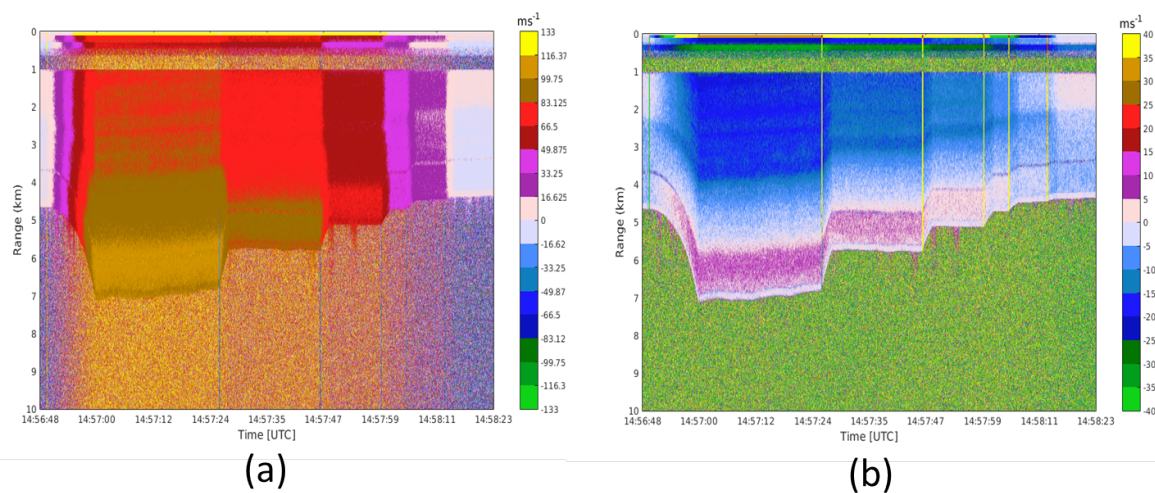
Figure 16. Velocity fields for the case study in Fig. 15: (a) measured PDPP velocity and (b) estimated velocity of the precipitation along the direction of the antenna beam.
