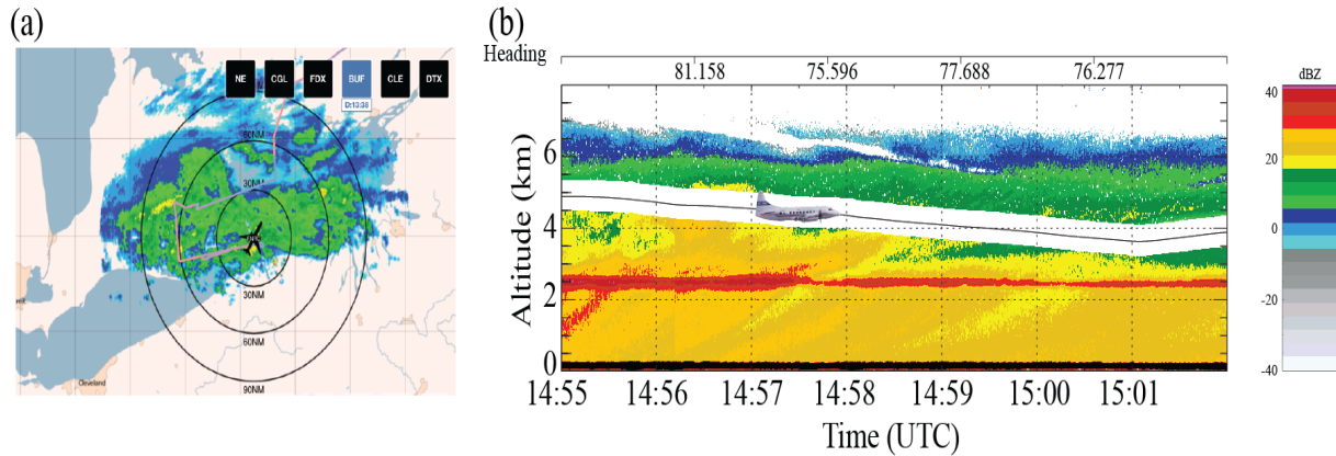
Figure 13. Same as Fig. 8 except during the PDPP data collection inside a winter storm on 25-Mar-2017.
