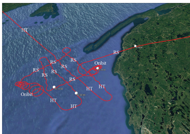
Figure 3. Typical PDPP flight track showing where the aircraft performed a series of horizontal transects (HT), roll sweeps (RS) and orbits of various roll angles.
