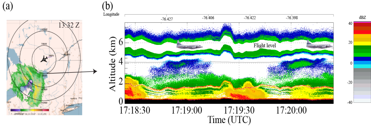
Figure 8. (a) Screen capture of NexRad Buffalo S-band Radar received at the aircraft as it leaves Ottawa, ON, Canada on 10-Jan-2017. (b) Vertical cross-section of Z_e obtained by the NRC Airborne X-band (NAX) radar while the aircraft is sampling a cloud system over Lake Ontario.
