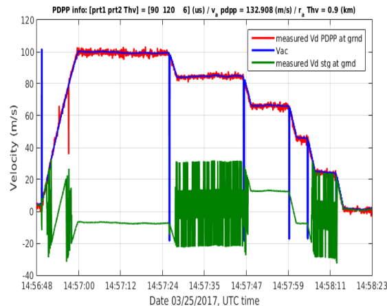
Figure 17. PDPP measured velocity (red line), the aircraft contribution computed from the aircraft INS data (blue line) and velocity estimates using staggered PRT pulses (green) at ground gates for the study case in Fig. 13.
