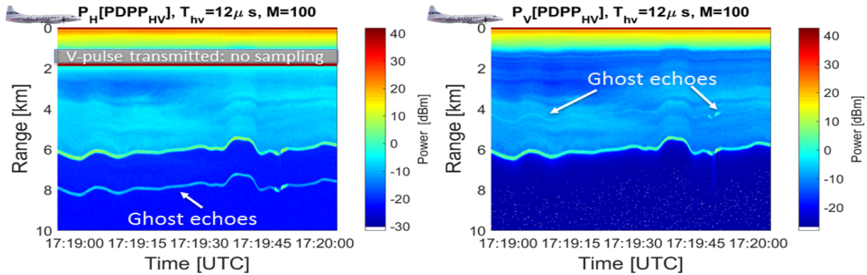
Figure 9. Example of power as recorded when operating in PDPP mode with H-pulse followed by an V-pulse after 12 \mu\text{s} . Left panel: power received in the H-channel; right panel: power received in the V-channel. The mechanism for producing ghost echoes is explained in the upper part of the panel.
