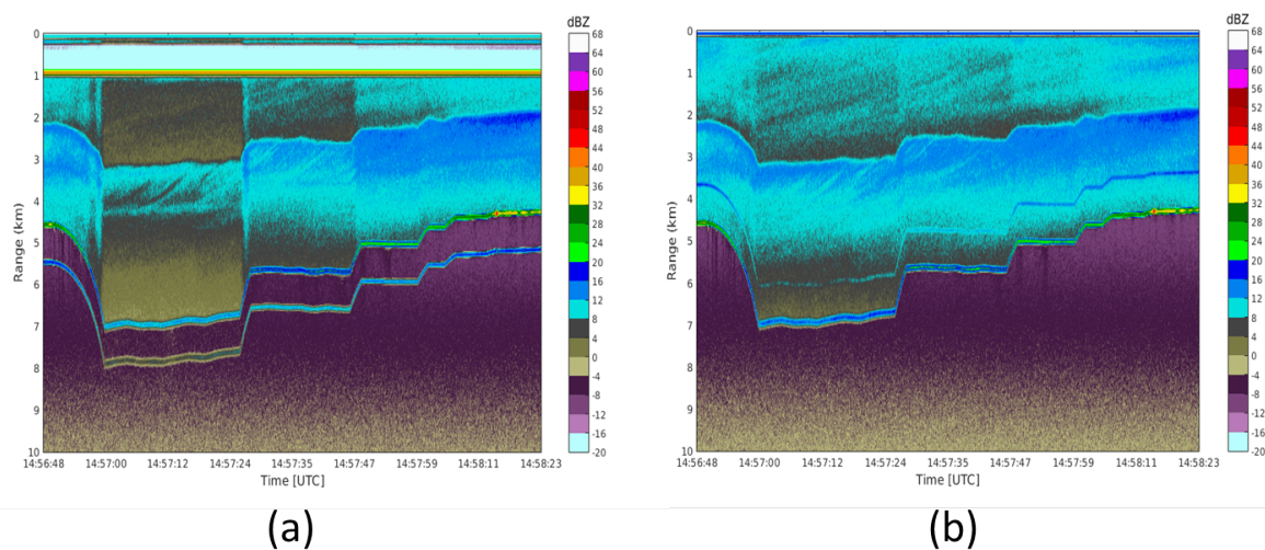
Figure 15. Similar to Fig. 9 but for March 25 flight and in reflectivity space. The PDPP spacing in this case is 6 \mu\text{s} .
