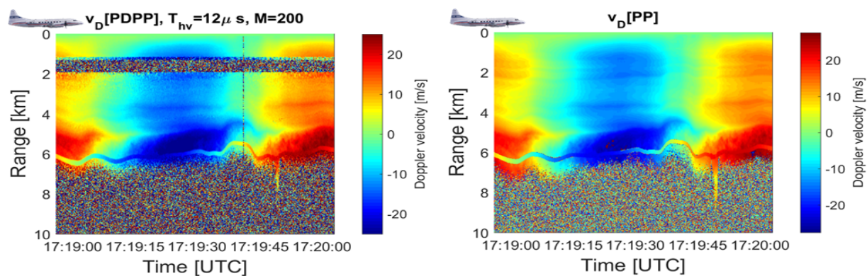
Figure 11. Velocity as measured by the PDPP technique with T_{hv} = 12 \mu s (left) and by the pulse-pair with two staggered pulse repetition times of 90 and 120 \mu s (right).
