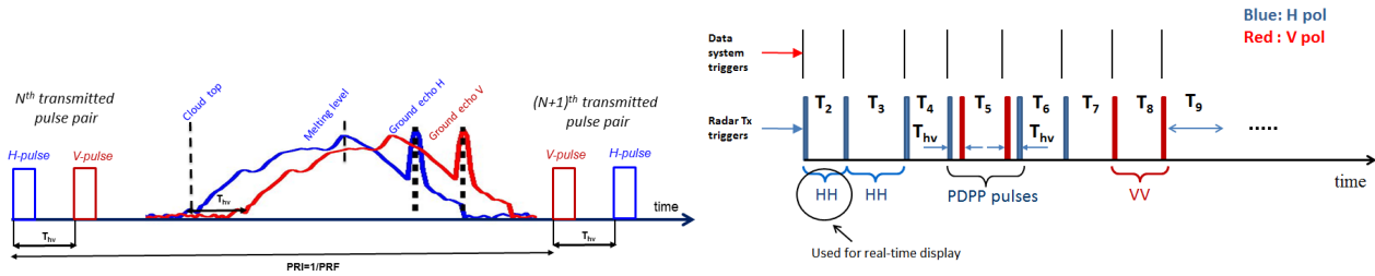
Figure 1. Top panel: schematic for the polarization diversity pulse mode. The terms H- and V- refer to the polarization state of the outgoing pulses. Pairs of H and V pulses are transmitted with a pulse-pair interval T_{hv} and with a pair repetition interval PRI . Each V-H pair is followed by an H-V pair. Between transmitted pulses, the H (blue) and V (red) receivers sample the backscattered power. Bottom panel: PDPP waveform implemented in the NRC airborne W-band radar system.
