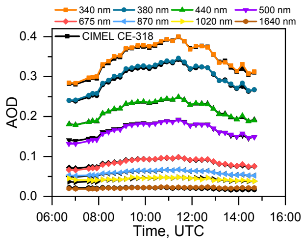
Figure 4. Comparison of the spectral extinction AOD from PLASMA (colored lines) and CIMEL CE-318 (black lines) sun photometers measurements on 12 June 2017 at Carpentras, France.
