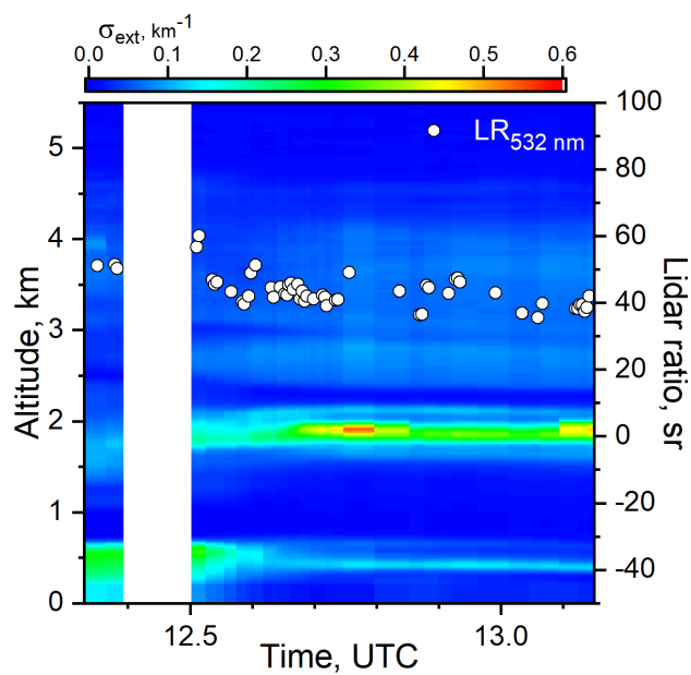
Figure 9. Spatio-temporal variability of extinction coefficient (colormap) and extinction-to-backscatter ratio (white dots) at 532 nm from on-road mobile measurements along Lille-Dunkerque transect on 26 August 2016 (12:18-13:10 UTC).
