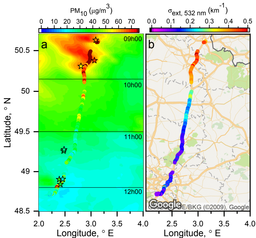
Figure 12. Spatial variability of (a) modelled PM_{10} concentrations and PM_{10} measured by mini-WRAS during mobile observations along Lille-Palaiseau transect on 28 August 2017. Air quality stations along the road are marked with colormapped stars. The colormap is the same for both the measured and the modelled PM_{10} concentrations. (b) extinction coefficient at 532 nm at ground level computed using Mie calculations on aerosol spectrometer data.
