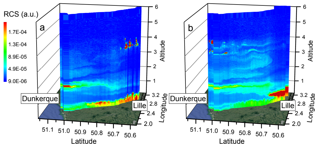
Figure 6. Three-dimensional view on the spatio-temporal variability of the LiDAR range-corrected signals measured along (a) Lille-Dunkerque and (b) Dunkerque-Lille transects on 26 August 2016. Observed structures: PBL up to 1 km altitude, elevated aerosol layers between 2 and 5 km and scattered clouds at 4 km near Lille and Dunkerque represented with red color.
