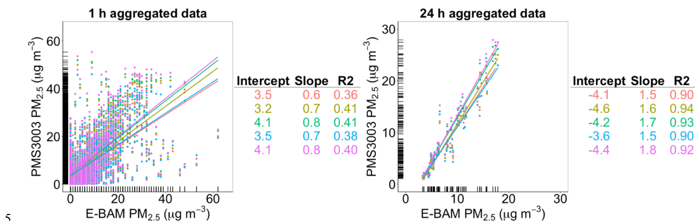
Figure 4: Linear regressions between aggregated PM_{2.5} mass concentrations ( \mu g m^{-3} ) of the E-BAM and the five uncalibrated PMS3003s at 1 h and 24 h time intervals from February 1, 2017 to March 31, 2017 at Duke University (6 h and 12 h results not shown). Marginal rugs were added to better visualize the distribution of data on each axis.
