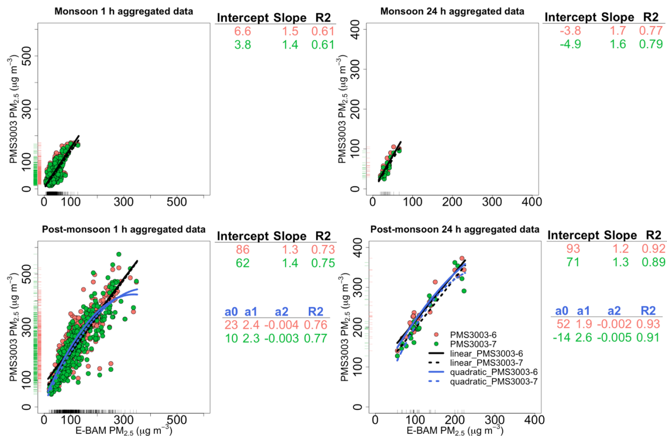
5 Figure 10: Linear regressions between aggregated PM 2.5 mass concentrations ( \mu\text{g m}^{-3} ) of the E-BAM and the two uncalibrated PMS3003s at 1 h and 24 h time intervals during the monsoon season (from June 8, 2017 to June 29, 2017), and the post-monsoon season (from Oct 23, 2017 to Nov 16, 2017) at IIT Kanpur (6 h and 12 h results are shown in Fig. S9). The fit coefficients for the calibration models are provided. Marginal rugs were added to better visualize the distribution of data on each axis.
