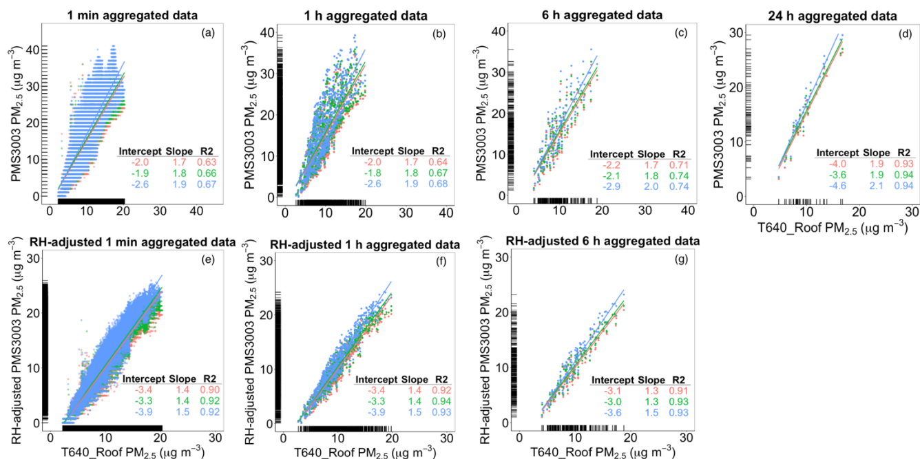
Figure 7: Linear regressions between aggregated \text{PM}_{2.5} mass concentrations ( \mu\text{g m}^{-3} ) of the T640 sitting on the roof (T640_Roof) and the three PMS3003s from June 30, 2017 to July 31, 2017 at US EPA RTP. In a–d, the PMS3003 readings are raw values at 1 min, 1 h, 6 h, and 24 h, respectively (12 h results are not shown). In e–g, the PMS3003 readings are RH-adjusted values at 1 min, 1 h, and 6 h, respectively. Marginal rugs were added to better visualize the distribution of data on each axis. Note the rug on the y axis in a is sparse because 1 min raw PMS3003 \text{PM}_{2.5} measurements are recorded as integers.
