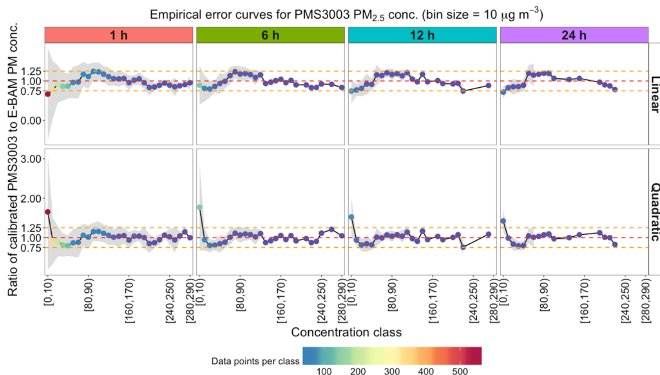
Figure 12: Empirical error curves for the E-BAM calibrated Plantower PMS3003 \text{PM}_{2.5} measurements at 1 h, 6 h, 12 h, and 24 h time intervals by two different calibration methods (i.e., simple linear and quadratic equations). The curves were generated from the combination of the Duke University and IIT Kanpur data sets. The points and lines represent the means of ratios of E-BAM-calibrated-PMS3003 to E-BAM \text{PM}_{2.5} measurements in different concentration classes, each of which spans a 10 \mu\text{g m}^{-3} interval. The shaded region represents the corresponding magnitudes of errors of PMS3003 \text{PM}_{2.5} measurements after the E-BAM calibration. The concentration classes are color coded by the number of data points in each class. Note the shaded region is generally absent from near the upper end of the \text{PM}_{2.5} ranges due to insufficient observations for the error evaluation. The red dashed line indicates ratio of 1, while the two orange dashed lines indicate ratio of 0.75 and 1.25, respectively.
