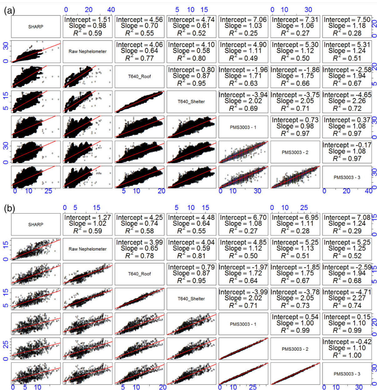
5 Figure 6: Pairwise correlations between (a) 1 min aggregated PM 2.5 mass concentrations (µg m -3 ) (b) 1 h aggregated PM 2.5 mass concentrations (µg m -3 ) of the SHARP, the SHARP's nephelometer, the two T640s, and the three uncalibrated PMS3003 sensor packages between June 30, 2017 and July 31, 2017 at US EPA RTP. In both (a) and (b), the upper-right set of panels includes the intercept, slope, and R 2 of linear regression models using the ordinary least squares (OLS) method; the lower-left set of panels shows the linear regression lines superimposed on pairwise plots.
