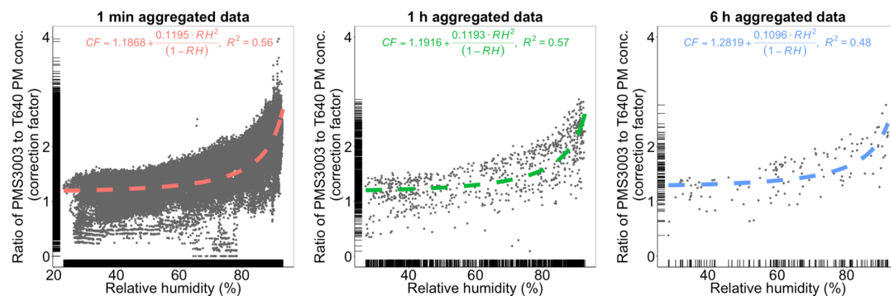
Figure 8: Fractional increase in \text{PM}_{2.5} weight measured by the uncalibrated PMS3003 sensors with respect to RH at 1 min, 1 h, and 6 h time intervals from June 30, 2017 to July 31, 2017 at US EPA RTP. RH (%) and PMS3003 \text{PM}_{2.5} concentrations ( \mu\text{g m}^{-3} ) are arithmetic means averaged across all the three PMS3003 sensor packages at each point in time. The fitted RH adjustment equations and curves were superimposed on the plots. Marginal rugs were added to better visualize the distribution of data on each axis. The results of 12 h and 24 h aggregated data are not shown as their patterns are relatively indistinct.
