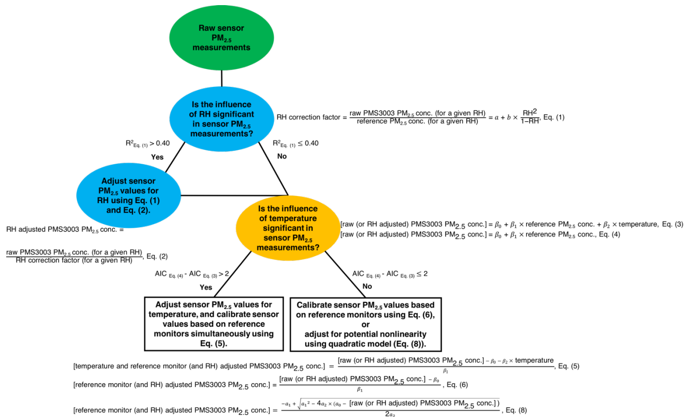
Figure 2: Flow path for sensor calibrations.
