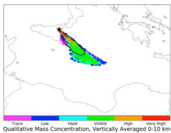
b) Nominal HYSPLIT
