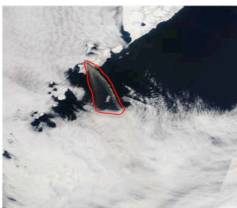
d) Terra MODIS Truecolor Scene
