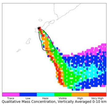
a) MISR-Initialized HYSPLIT
