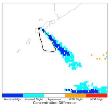
c) MISR - Nominal Difference
