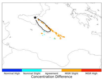
c) MISR - Nominal Difference
