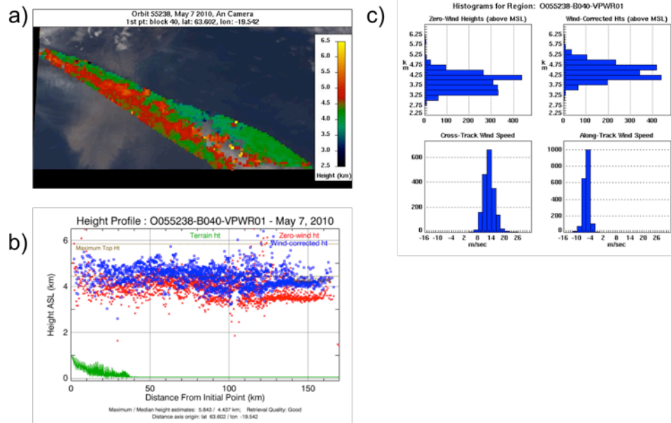
Figure 1. MINX Height Retrievals, measured from the geoid, for the Eyjafjallajokull volcano eruption plume, May 7, 2010. (a) Elevation map for the main plume. Each box represents a 0.55 km area where the height is displayed with darker colors on the low end and warmer colors on the high end. (b) MINX Height Profile, as a function of distance from the source. Terrain elevation is indicated by the green line. The injection height is ~ 5.8 km directly above the source, and remains at similar elevation downwind. (c) MINX Height Histogram, provides distribution of height retrievals without a wind correction, with the wind correction, and the cross/along track wind speeds.
