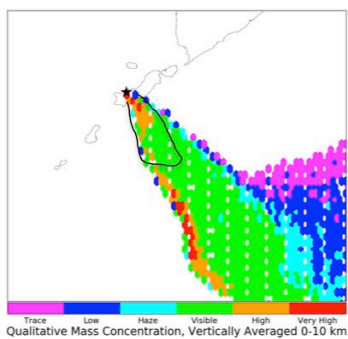
b) Nominal HYSPLIT
