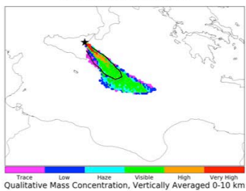
a) MISR-Initialized HYSPLIT
