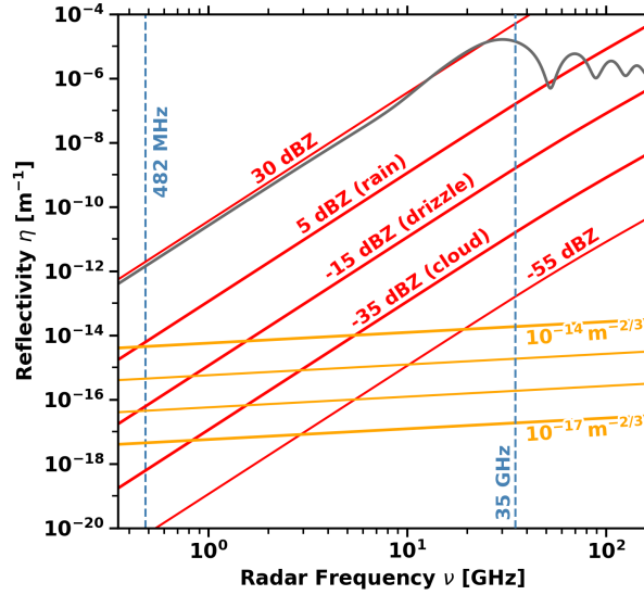
Figure 2. Reflectivity of different scattering processes. Red lines indicate typical values of hydrometeor reflectivity with the sensitivity threshold of the cloud radar at -55 dBZ (Görsdorf et al., 2015). Orange lines indicate the reflectivity for C_n^2 typically observed in the atmosphere (e.g. Clifford et al., 1994). The grey line shows the reflectivity of one liquid drop ( N = 1 \text{ m}^{-3} ) with a diameter of d = 3 \text{ mm} as derived from Mie theory.
