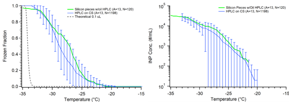
Figure 6. Comparison of freezing on silicon wafer chips (green) against hydrophobic cover slips (blue), following Figure 5. The freezing temperature spectrum is on the left, and the retrieved c_{IN} is on the right. Both datasets use 0.1 \mu\text{L} droplets. The data from all replicate arrays using silicon (green) are combined into one series and thus no error bars can be determined. The parentheses next to each legend entry contains the number of arrays of droplets (A) and the total number of droplets across all arrays (N). The gray dashed line indicates the theoretical homogeneous freezing curve of 0.1 \mu\text{L} droplets, using the parameterization of Koop and Murray (2016).
