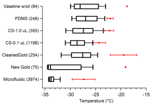
Figure 11. Summary of pure water droplet freezing spectra for different substrates tested. Boxes show the 25% and 75% frozen quartiles and the median, N_{50} , is indicated by the line inside each box. Red markers are the temperatures of the first onset freezing droplets with error bars showing variability between different replicate droplet arrays. No error bars for the onset freezing for Vaseline and gold wafer are shown because
