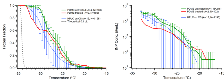
Figure 9. Measurements of HPLC pure water droplet freezing on PDMS are shown in red and green, following Figure 5. The data from small droplets on a silanized coverslip are displayed for comparison in blue (Fig. 5, blue). The PDMS data was obtained using treated (red) and untreated (green) PDMS polymer with small droplets. The parentheses next to each legend entry contains the number of arrays of droplets (A) and the total number of droplets across all arrays (N). Error bars on green data show standard deviation from replicate arrays, while the red data are combined into one series as explained in section 2. The gray dashed line indicates the theoretical homogeneous freezing curve of 0.1 uL droplets, using the parameterization of Koop and Murray (2016).
