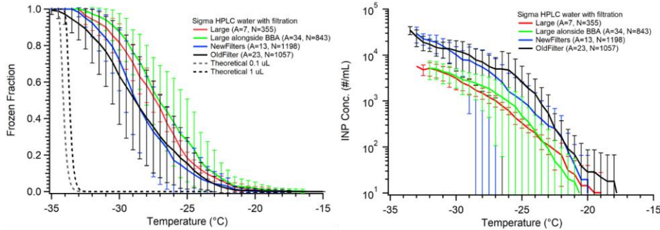
Figure 5. Droplet freezing temperature spectra (left) and apparent ice nuclei concentration, c_{\text{IN}} , (right) for pure water droplet freezing measurements on a hydrophobic cover slip. In all experiments HPLC water that was filtered using an Anotop 0.02\ \mu\text{m} syringe filter was used. Each data series has been binned into 0.5^{\circ}\text{C} temperature increments. The red data series is from large ( 1.0\ \mu\text{L} ) droplets, green is from large ( 1.0\ \mu\text{L} )
