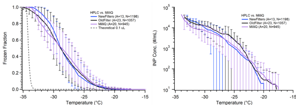
Figure 3. Comparison of pure water freezing using filtered MilliQ produced water and filtered purchased HPLC water. Shown are the measured droplet freezing temperature spectra (left) and the derived INP concentration (right). HPLC water was filtered using a new Anotop 0.02 \mu\text{m} filter for each bottle of water (blue), or the same filter for multiple stock bottles of water (black). The results from typical MilliQ water arrays are shown in purple. The parentheses next to each legend entry contains the number of arrays of droplets (A) and the total number of droplets across all arrays (N). The gray dashed line indicates the theoretical homogeneous freezing curve of 0.1 \mu\text{L} droplets, using the parameterization of Koop and Murray (2016).
