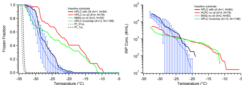
Figure 7. Pure water droplet experiments on a Vaseline coated substrate, following Figure 5. The HPLC water using a silanized coverslip data in blue are displayed for comparison and is the data from the hydrophobic cover slip using small droplets (Fig. 5, blue). The data from replicate arrays for Vaseline is combined as described in Section 2 and thus no error bars are determined for these. Three sets of experiments on Vaseline are shown: black is small droplets (0.1 \mu L) of HPLC filtered water in oil, red is large droplets (1.0 \mu L) without oil, and green is large droplets of MilliQ water without oil. The parentheses next to each legend entry contains the number of arrays of droplets (A) and the total number of droplets across all arrays (N). The gray and black dashed lines indicate the theoretical homogeneous freezing curve of 0.1 \mu L and 1 \mu L droplets, respectively, using the parameterization of Koop and Murray (2016).
