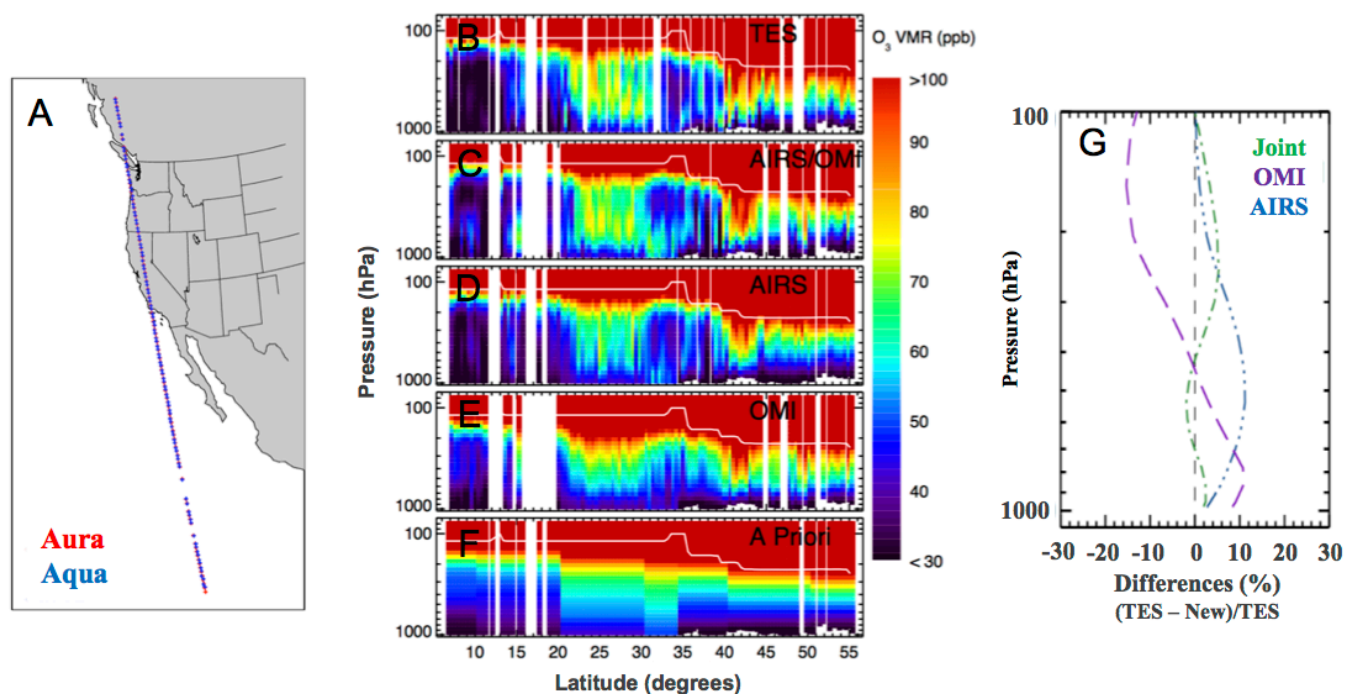
10 Figure 2: Collocated ozone (O 3 ) measurements from A-Train nadir viewing spectrometers over the western United States on August 23, 2006. (A) geolocation of 110 TES-AIRS-OMI triads (spatial-temporal differences ~8 km; ~16 minutes); (B) vertical profile of TES O 3 volume mixing ratio (VMR) data (version 6) with a unit of parts per billion (ppb); (C) joint AIRS+OMI retrievals; (D) AIRS alone; (E) OMI alone; (F) a priori used in retrievals; (G) averaged percentage differences of retrieved O 3 profiles in comparison to TES O 3 data (version 6): TES vs. joint AIRS+OMI (green dash-dot), TES vs. AIRS alone (blue), and TES vs. OMI alone (purple dash). The white curves in the panels of B–F indicate the tropopause pressure taken from the Goddard Earth Observing System Model, Version 5. 15
