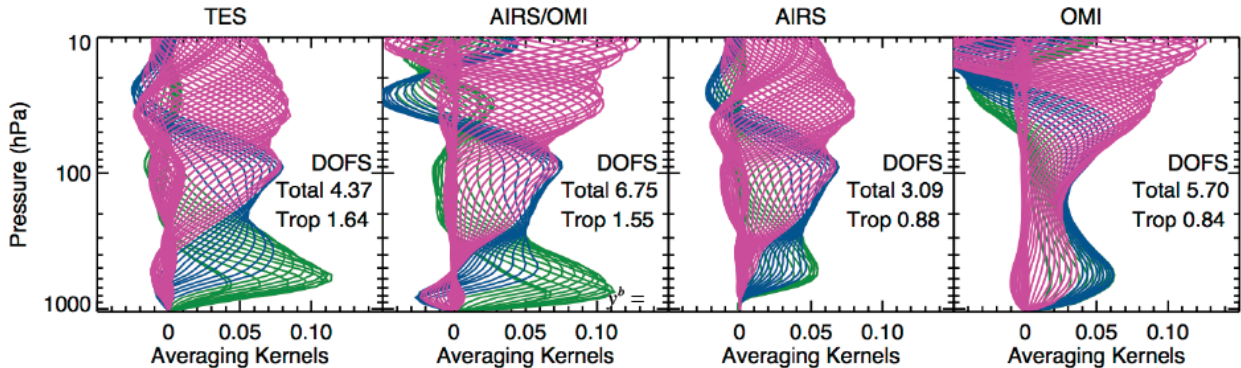
Figure 1: Averaging kernels of collocated measurements of TES (version 6), joint AIRS+OMI, AIRS alone, and OMI alone over California, USA on August 23, 2006. The green, blue, and magenta curves in four panels indicate the averaging kernels in the pressure range of surface-400 hPa, 400 to 100 hPa, and above 100 hPa, accordingly.
