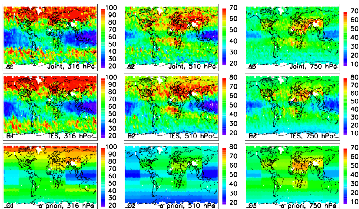
Figure 3: Global maps of monthly averaged ozone (O 3 ) volume mixing ratio (VMR) with a unit of ppb. The A-Train measurements in August 2006 were used in creating these global maps. Comparison of Joint AIRS+OMI (top row, A), TES (middle row, B), and a priori (bottom row C) ozone VMR for the pressure level of 316, 510 and 750 hPa (columns left, middle, right), respectively. All data have been gridded to 2.5° × 2.5° cells. Results for the remaining months of 2006 are available in supplement Figures S1–S11.
