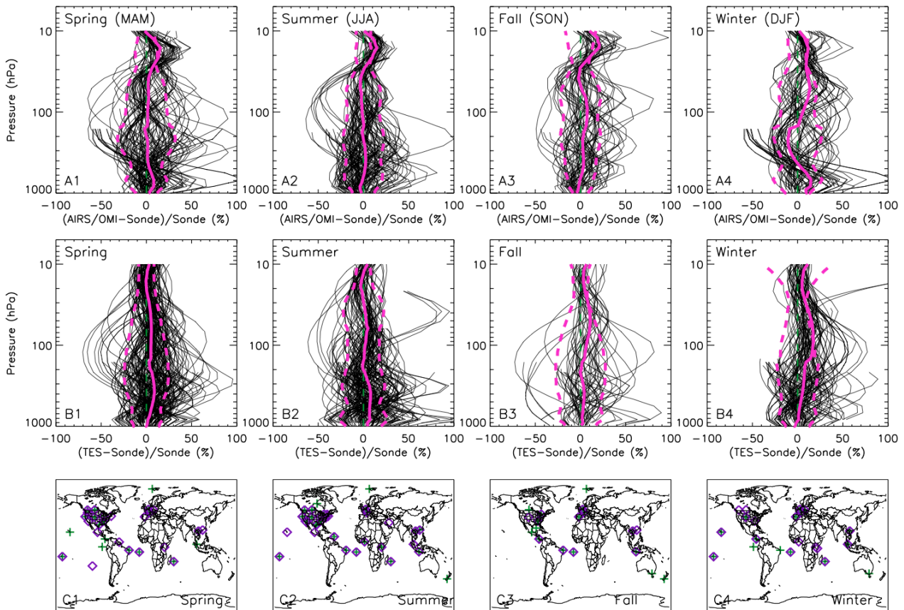
15 Figure 6: Joint AIRS+OMI-sonde (A1–A4) and TES-sonde (B1–B4) percentage differences of measured ozone concentration for the four seasons (months abbreviated in parentheses) over global. Individual profiles are shown in black, and the mean and 1 sigma standard deviation range are overlaid in solid magenta (mean) and dashed magenta lines. The profiles were plotted after removing cloudy scenes and flagged satellite (joint AIRS+OMI and TES) data. (A1–A4) joint AIRS+OMI vs. ozonesonde; (B1–B4) TES data
