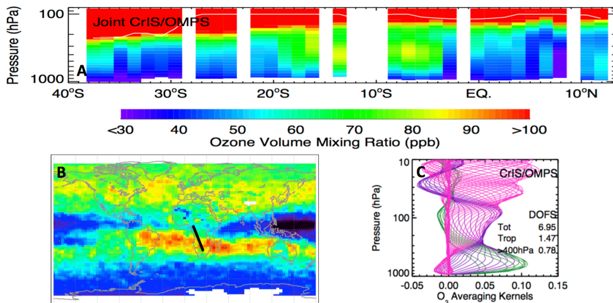
Figure 7: Joint CrIS+OMPS ozone profile retrievals over Africa on October 21, 2013. The elevated ozone concentrations between 2–20°S are associated with biomass burning. (A) The retrieved ozone concentration profiles along the transect measurements. The white curve indicates the tropopause pressure reported by GEOS-5. (B) TES monthly mean ozone concentration at 510 hPa. The black line indicates the joint CrIS+OMPS measurements location. (C) The averaging kernels of joint CrIS+OMPS measurements.
