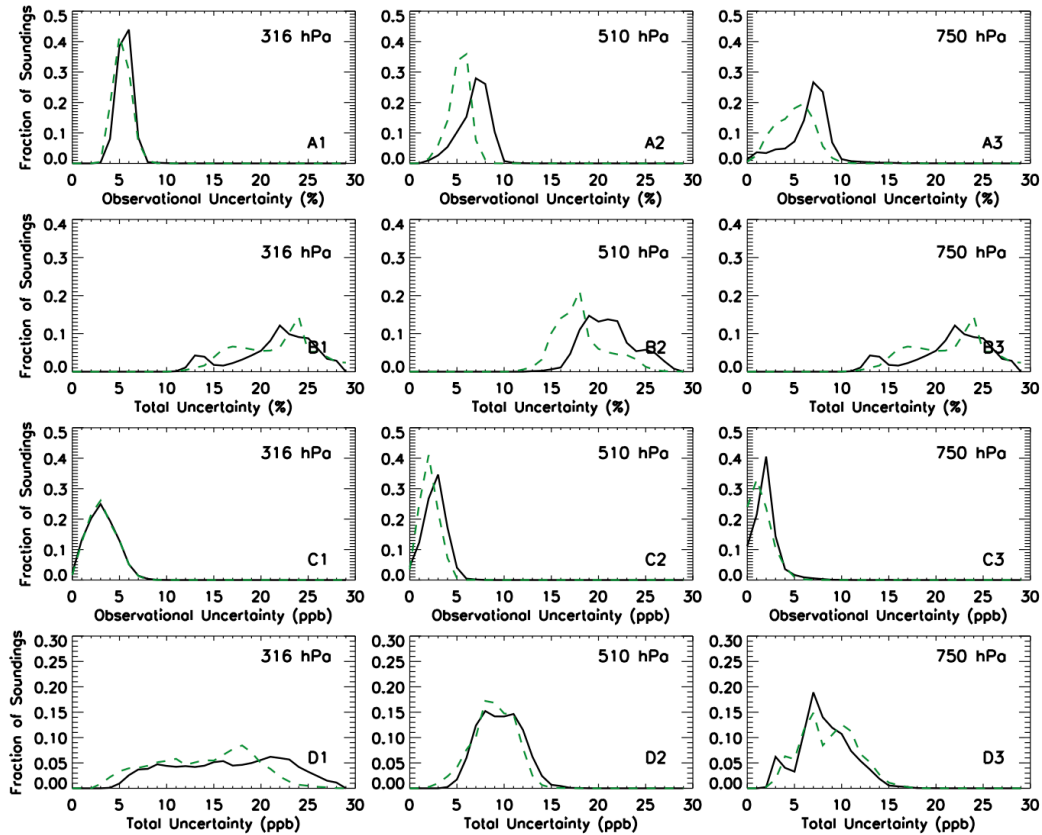
Figure 5: Estimated (predicted) uncertainty of retrieved global O 3 concentration shown in Fig. 3. Here, we used the A-Train measurements from August 2006. Results for the remaining months of 2006 are available in supplement Figures S23–S33. (A1–A3) observational uncertainty; (B1–B3) total uncertainty; (C1–C3) observational uncertainty in ppb; and (D1–D3) total uncertainty in ppb. Joint AIRS+OMI data are shown in black line, and TES version 6 data are shown in green dash.
