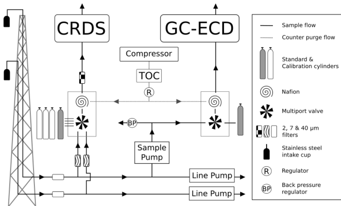
Figure 2: A generalised schematic showing the initial Bilsdale and Heathfield site setup of the cavity ringdown spectrometer (CRDS) and the Gas Chromatograph – Electron Capture Detector (GC-ECD) including the dry gas generator (TOC) and back pressure regulator (BP). Note that Bilsdale has three inlets, while Heathfield has only two as shown here. The Nafion® drying system located downstream of the CRDS multiport valve was removed at both sites in 2015. Black arrows and lines show the direction of sample, standard and calibration gas flow. Grey dashed lines and arrows show the flow path of the Nafion® counter purge gas.
