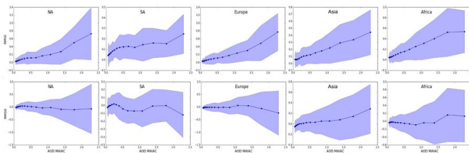
Figure 8. Absolute error ( mse , top row) and bias ( rmsd , bottom row) of MAIAC AOD for different world regions as a function of retrieved AOD. NA and SA stand for the North and South America, respectively.
