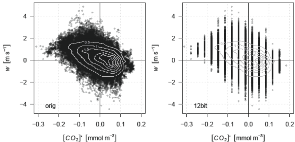
10 Figure 2: Quadrant (hole) analysis of all data points (20 Hz sampling rate) of the vertical wind velocity and the carbon dioxide concentration for one hour (summer at noon) with 16-bit-digitalization (left) and reduced to 12-bit-digitalization (right). A normalized density distribution in form of isopleths is included in both figures.
