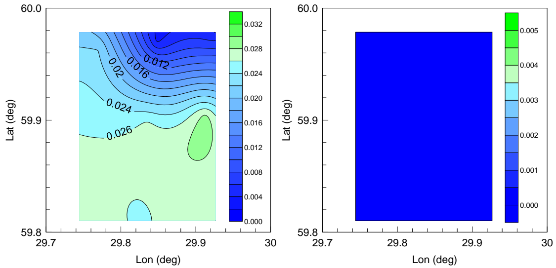
Figure 5: The map of the mean (left) and median (right) LWP values ( \text{kg m}^{-2} , colour scale) calculated for the small terrain (9 pixels, see Fig. 1) and for the CD dataset (measurements by the SEVIRI instrument).
