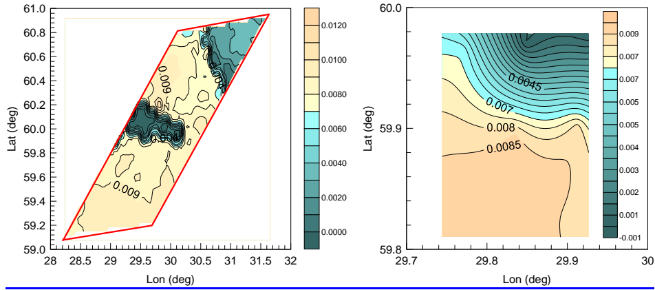
Figure A1.1: The maps of the median LWP values ( \text{kg m}^{-2} , colour scale) calculated for the large terrain (left) and small terrain (right) and for the 2-year period 1 Dec 2012 – 30 Nov 2014 (measurements by the SEVIRI instrument).
