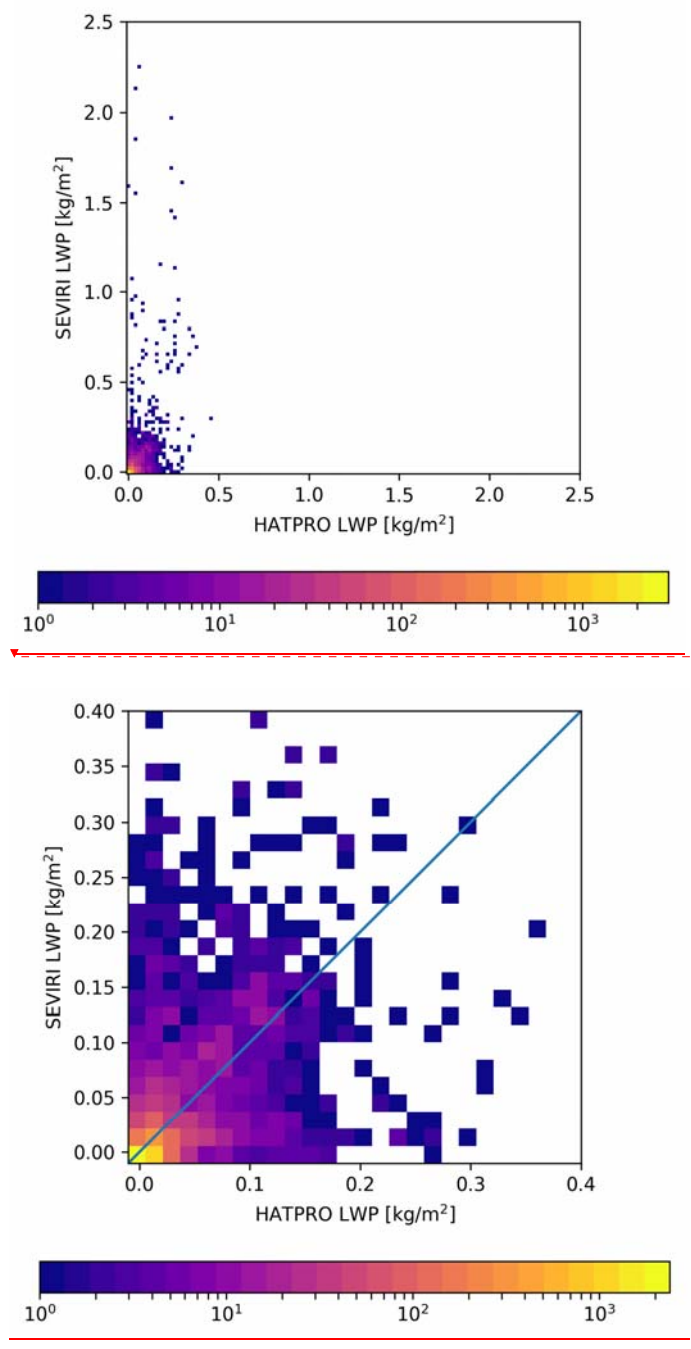
Figure 9: Comparison of the HATPRO and SEVIRI instantaneous measurements by means of two-dimensional histogram with number of occurrence colour scale. Upper panel: extra high LWP values are shown, lower panel: only LWP < 0.4 \text{ kg m}^{-2} are shown.
