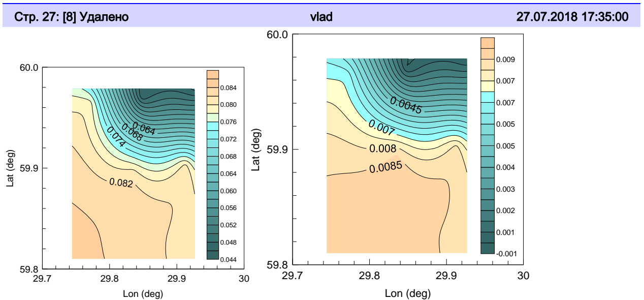
Figure 3: The map of the mean (left) and median (right) LWP values ( \text{kg m}^{-2} , colour scale) calculated for the small terrain (9 pixels, see Fig. 1) and for the 2-year period 1 Dec 2012 – 30 Nov 2014 (measurements by the SEVIRI instrument).
