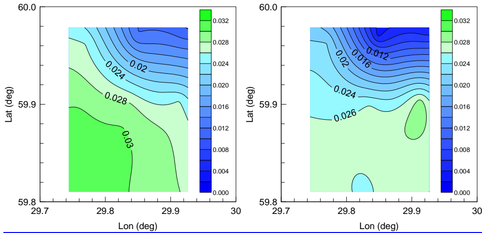
Figure 3: The map of the mean LWP values ( \text{kg m}^{-2} , colour scale) calculated for the small terrain and for the WH (left) and CD (right) datasets (measurements by the SEVIRI instrument).
