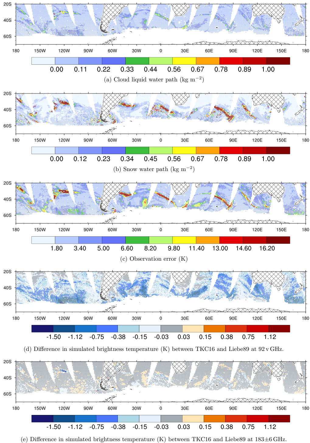
Figure 7. Maps for a) cloud liquid water path from corresponding FG field, b) snow water path from corresponding FG field, c) observation error with Liebe89, d) difference in FG at 92 v between TKC16 and Liebe89 and e) difference in FG at 183 \pm 6 GHz between TKC16 and Liebe89 for areas of the southern mid- to high latitudes excluding land and sea ice for a 12-hour window centred at 3 UTC on 30 August 2016, co-located to SSMIS-F17 observations. Cross-hatched areas represent land and white areas have no data due to e.g. screening or quality control (see section 2.2)
