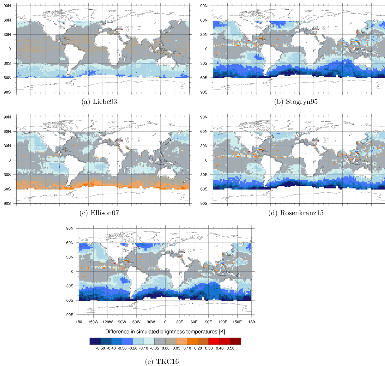
Figure 4. As Fig. 3 but for channel 92 v.
