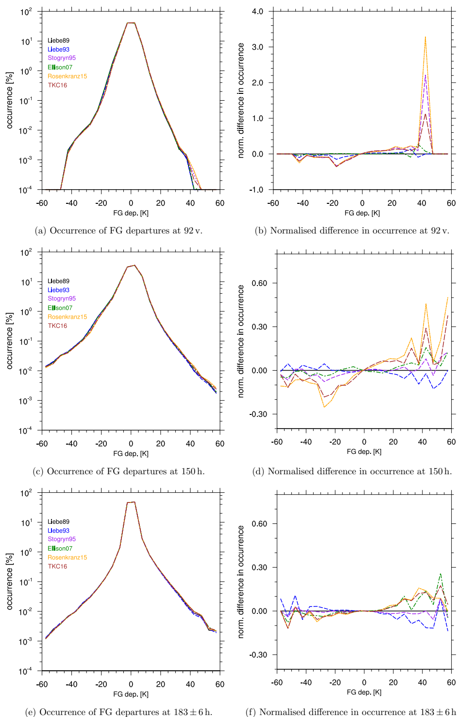
Figure 10. Histograms of FG departures [K] using different liquid water permittivity models with the right panel showing the normalised difference for the newer permittivity models relative to Liebe89. Bin size is 5 K. Results cover the time period from 1 to 31 August 2016 for the southern hemisphere ( 20^{\circ}\text{S} to 90^{\circ}\text{S} ). Different colours refer to different permittivity models, as shown in the figure.
