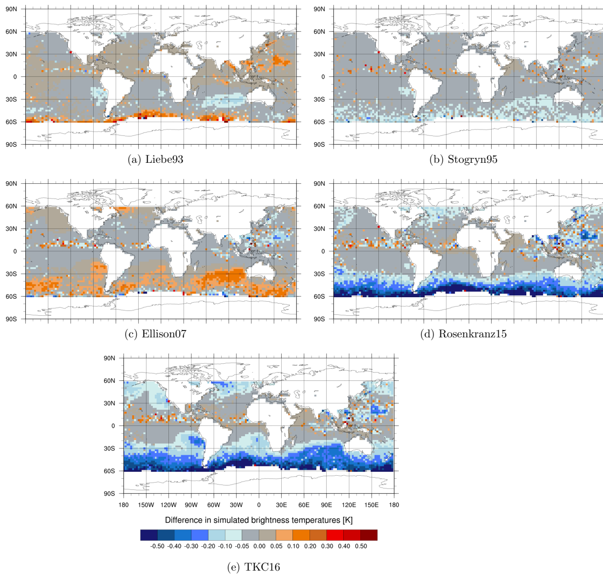
Figure 5. As Fig. 3 but for channel 150 h.
