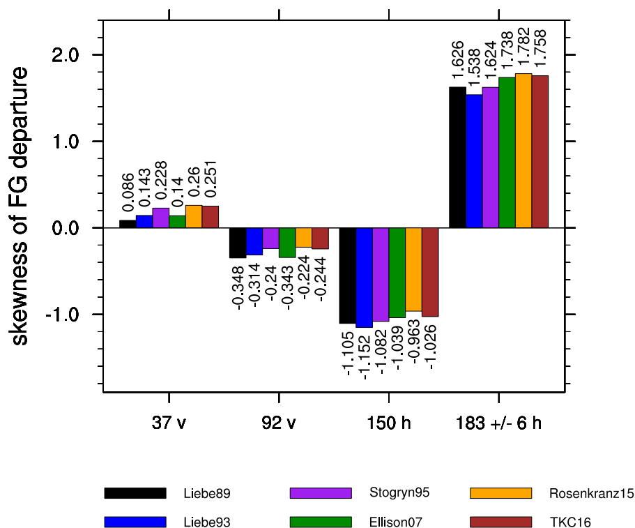
Figure 11. Skewness in FG departure distribution for the different liquid water permittivity models at 37 v, 92 v, 150 h and 183 ± 6 h collocated to SSMIS-F17 observations over the time period 1 to 31 August 2016 for the southern hemisphere (SH: 20° S to 90° S).
