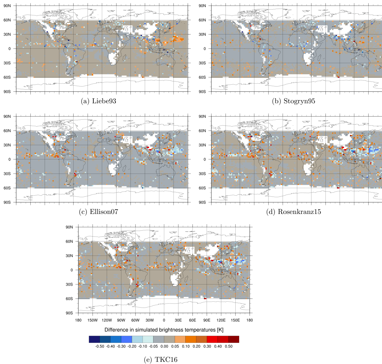
Figure 6. As Fig. 3 but for channel 183 \pm 6 h.
