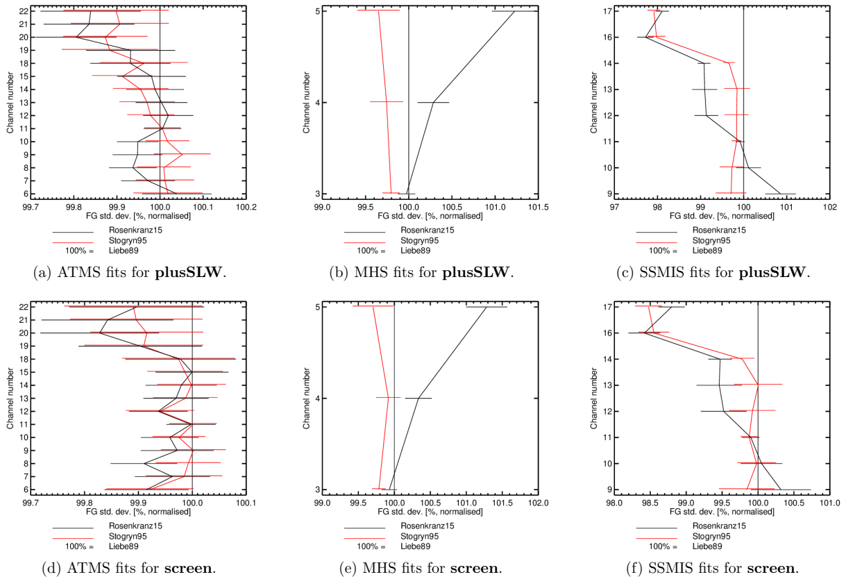
Figure 13. Standard deviation in FG departures in the southern hemisphere of ATMS, MHS and SSMIS for Rosenkranz15 and Stogryn95 normalised by Liebe89 for plusSLW and for screen . Different colours refer to different liquid water permittivity models, as shown in the figure. The horizontal bars indicate 95% confidence range. Results cover the time period from 1 June to 30 September 2016.
