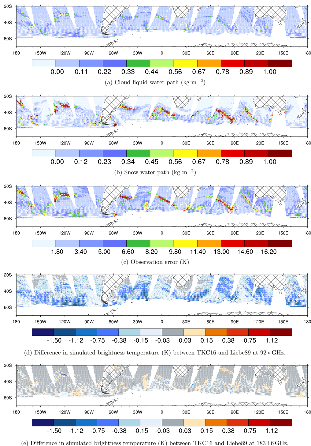
Figure 7. Maps for a) cloud liquid water path, b) snow water path, c) observation error with Liebe89, d) difference in FG at 92 v between TKC16 and Liebe89 and e) difference in FG at 183 \pm 6 GHz between TKC16 and Liebe89 for areas of the southern mid- to high latitudes excluding land and sea ice for a 12-hour window centred at 3 UTC on 30 August 2016, co-located to SSMIS-F17 observations. Cross-hatched areas represent land and white areas have no data due to e.g. screening or quality control (see section 2.2)
