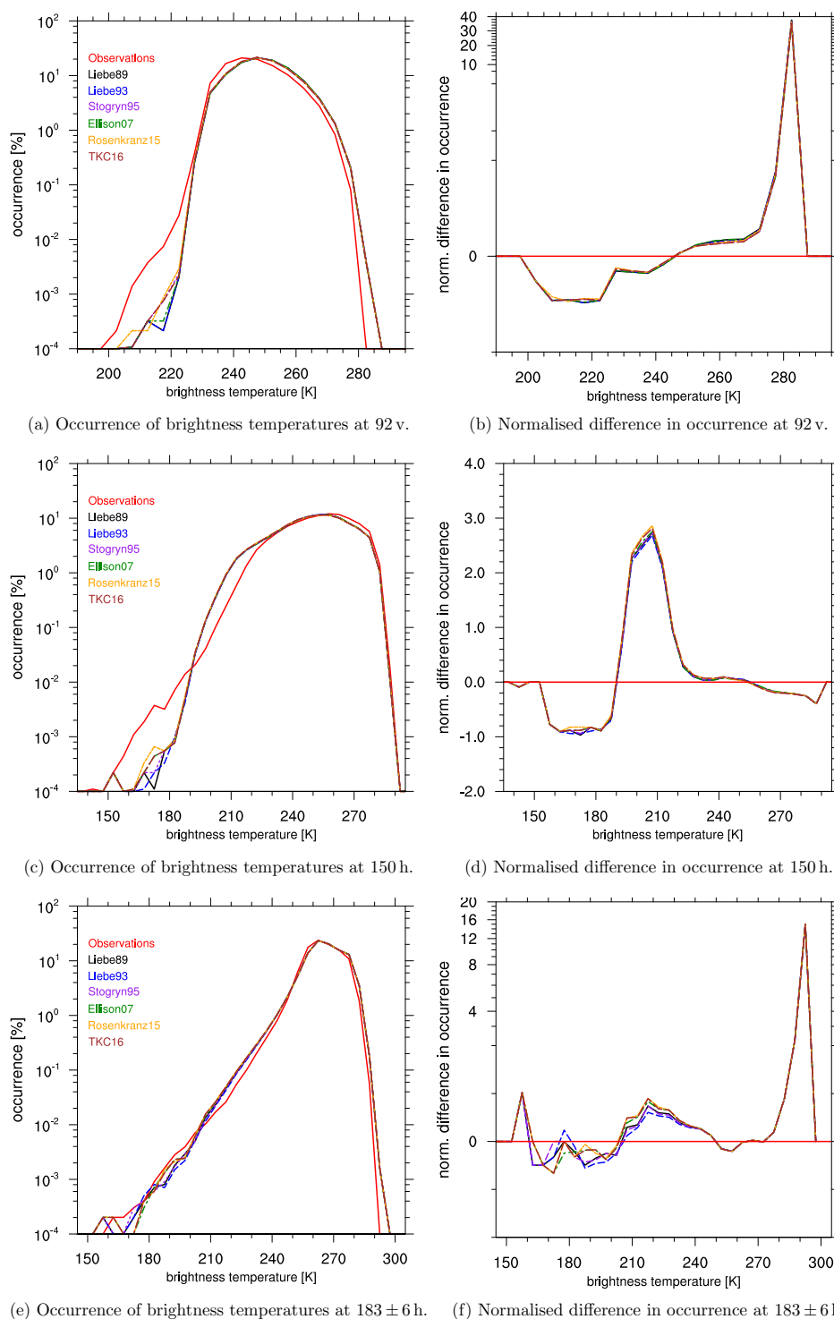
Figure 9. Histograms of simulated and observed brightness temperatures [K] using different liquid water permittivity models with the right panel showing the normalised difference in occurrence of simulated brightness temperatures relative to observations. Bin size is 5 K. Results cover the time period from 1 to 31 August 2016 for the southern hemisphere ( 20^{\circ}\text{S} to 90^{\circ}\text{S} ). Different colours refer to different permittivity models, as shown in the figure.
