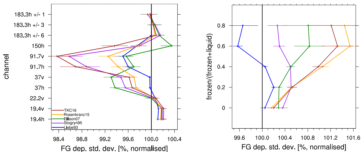
(a) Standard deviation in FG departures for samples with no frozen hydrometeors. (b) Standard deviation in FG departures at 183 ± 6 GHz.
