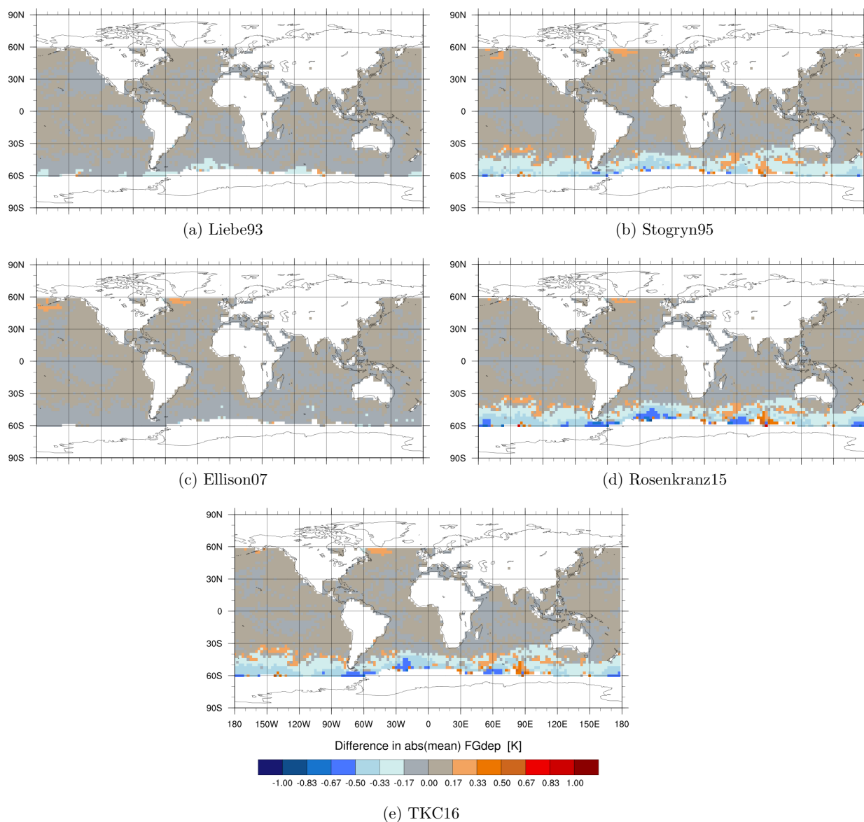
Figure A1. Maps of difference in observed minus simulated brightness temperatures [K] between the newer liquid water permittivity models and the current Liebe89 for 37 v brightness temperatures co-located to corresponding SSMIS-F17 observations. Means are computed in each 2.5^\circ lat x 2.5^\circ lon bin and over the time period 1 to 31 August 2016. White coloured areas correspond to areas where data is not assimilated, as mentioned in section 2.2.
