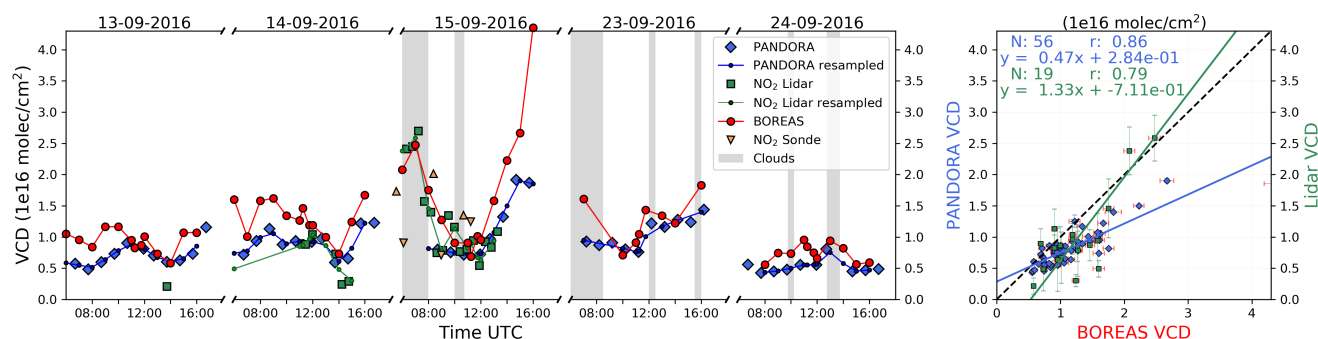
Figure 17. Left: time series of Pandora, LIDAR and BOREAS \text{NO}_2 -VCD. Blue diamonds show the original Pandora measurements, green squares the LIDAR datapoints. Small dots with connecting lines depict the resampled datasets of Pandora and LIDAR. BOREAS is shown as red circles. Grey areas indicate clouds. The plot includes orange triangles as the representation of the integrated \text{NO}_2 sondes measurements with the ascend and descend separated in different triangles with the edge to the top or to the bottom respectively. Right: scatter plot of the datasets including parameters of the orthogonal regression and Pearson's correlation coefficients.
