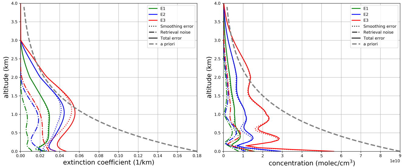
Figure 8. Retrieval errors for E1-E3 of the synthetic aerosol (left) and \text{NO}_2 study (right). Aerosol results are shown for SNR = 3000 and Tikhonov parameter \gamma = 2 . Trace gas errors are depicted without additional regularization ( g = 1 ). Pre-scaling was used.
