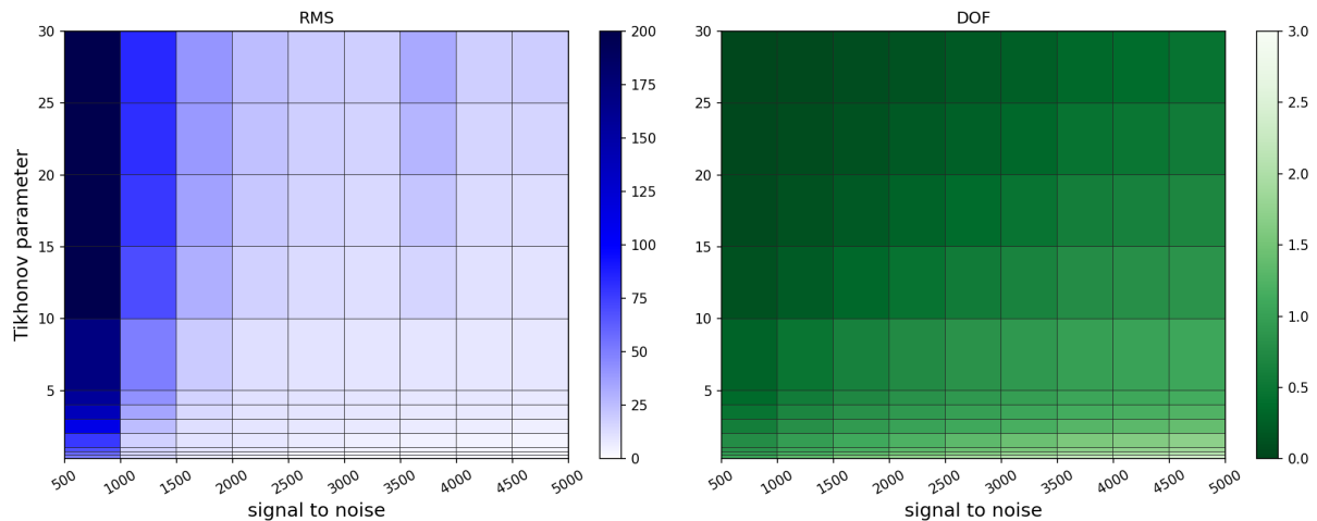
Figure 10. RMS between measured and simulated O_4 \Delta S and the matching degrees of freedom (DOF) for the specific retrievals for different SNR and \gamma values.
