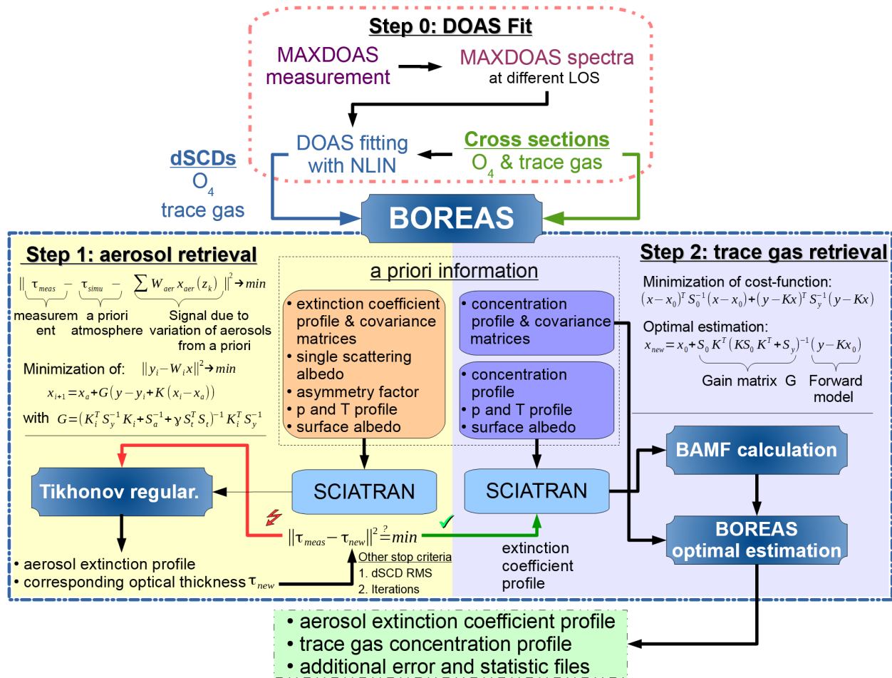
Figure 2. BOREAS analysis flow chart. The algorithm is separated into two steps. Step 1: Aerosol retrieval within a Tikhonov-Regularization. Step 2: Optimal estimation based trace gas retrieval.
