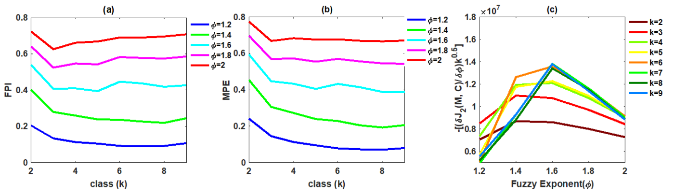
Figure 3: Determination of the number of classes, k , and the fuzzy exponent, \phi , for the FKM cloud-aerosol discrimination
