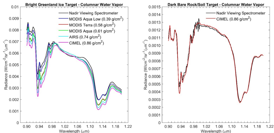
Figure 11 The airborne nadir viewing spectrometer's measurement sensitivities to columnar water vapor for bright Greenland ice (panel a) and dark bare rock/soil (panel b) targets. A variety of satellite columnar water vapor data products were evaluated for the bright Greenland ice target due to the remoteness of the flight line segment and its proximity to the Thule Air Base CIMEL.
