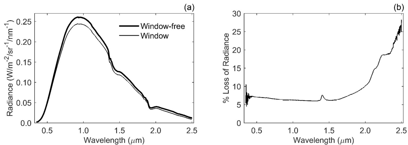
Figure 3. A measure of light transmission through the BK7 optical window mounted within the OrangeCan. Panel (a) shows the NIST traceable source output with and without the optical window. Panel (b) summarizes wavelength-dependent radiance loss due to window transmissivity.
