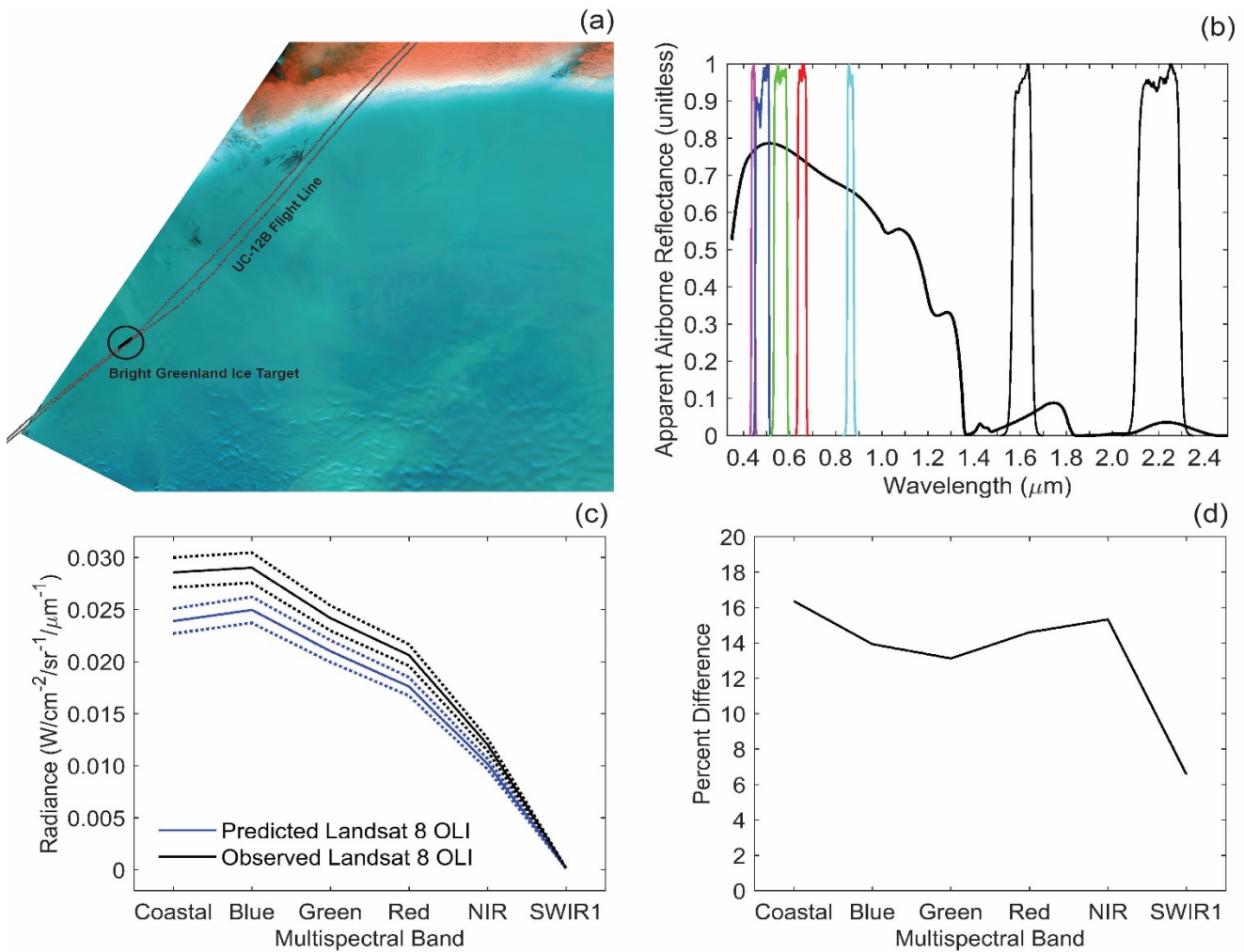
Figure 13. MODTRAN predicted radiance for coincident Landsat 8 OLI imaging of the bright Greenland ice target using the nadir viewing spectrometer apparent reflectance spectrum. Panel (a) shows the Landsat 8 OLI image acquisition on 29 July 2015 with the bright Greenland ice target (black line within the black circle), and the UC-12B flight line (grey line). Panel (b) shows Landsat 8 OLI's visible, NIR, and SWIR1/2 relative spectral response functions plotted over the bright Greenland ice target apparent reflectance spectrum. Panel (c) is the comparison of convolved predicted and measured Landsat 8 OLI radiance for the bright Greenland ice target using the average of 24 airborne Greenland ice spectra, and the average of 24 closest Landsat pixels. The dotted lines indicate the within 5% measurement requirement for both Landsat 8 OLI (absolute calibration) and the airborne nadir viewing spectrometer (relative calibration). Panel (d) is the percent difference [percent difference = (measured – predicted) / measured] between predicted and measured Landsat 8 OLI radiance. Note, radiance for Landsat 8 OLI was not predicted for the SWIR2 relative spectral response function based on UC-12B BK-7 window transmission uncertainty beyond 2.0 \mu\text{m} .
