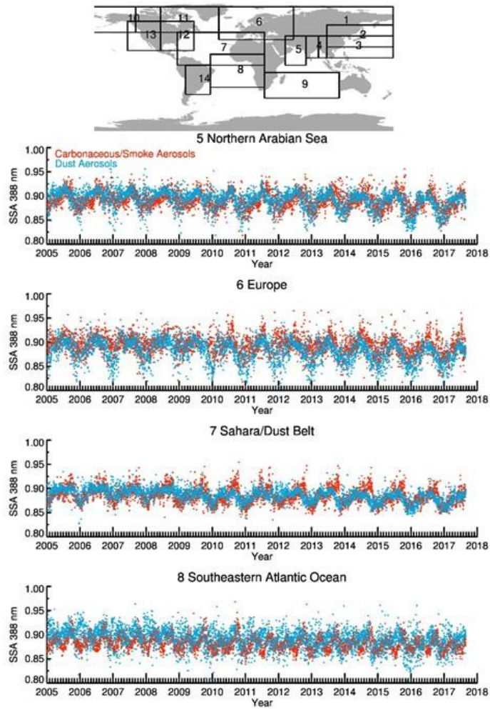
5 Figure 2 (Top) Geographical boundaries of select 14 regions considered for calculating corresponding regional values of SSA (388 nm). (Remaining panels) Regional mean UVA1 weighted cloud-free SSA (388 nm) for carbonaceous, and dust aerosols for the four selected regions (numbered 5, 6, 7, and 8 in the top panel) derived using OMI/OMAERUV operational (version 1.8.9.1) L2 cloud-free SSA retrievals.
