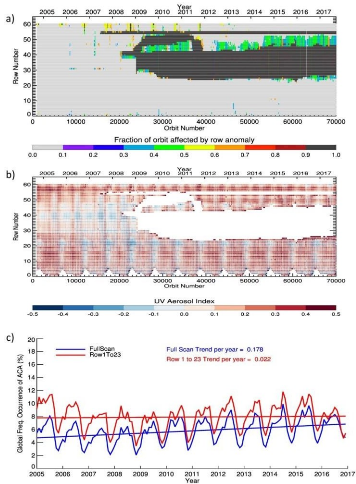
5 Figure 6 (a) Chart showing the time evolution of OMI row anomaly and (b) cloudy-sky (LER388>0.25) UVAI. (c) Monthly time-series of the global, cloudy-sky frequency of occurrence (in % with respect to the total cloudy-sky observations) of absorbing aerosols above cloud derived using OMI full scan (Rows 1 to 60) (blue) and anomaly-free observations (Rows 1 to 23) (red). Solid lines represent the linear regression fits to the respective time-series data.
