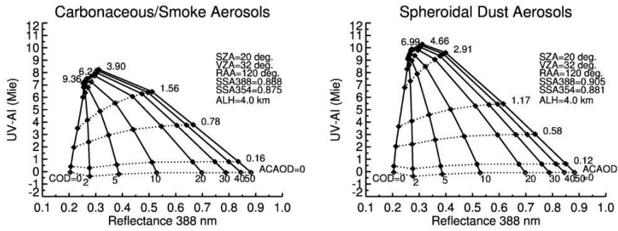
5 Figure 1 Simulation of UVAI (y-axis) versus Reflectance at 388 nm (x-axis) for the different pairs of ACAOD and COD (both at 388 nm) for the carbonaceous (left) and spheroidal shape dust aerosols (right). Values of ACAOD and COD depicted in the figure correspond to the 388 nm wavelength. The shown 2-D diagram forms the retrieval domain in which the observations from OMI are fitted and related to a pair of ACAOD and COD.
