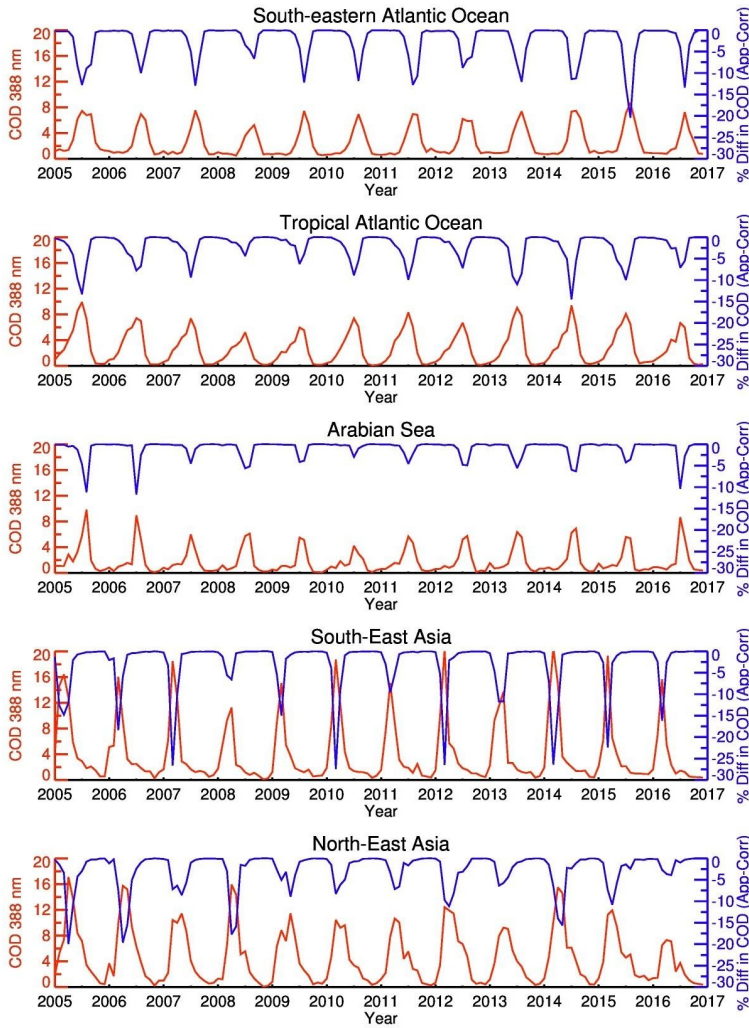
5 Figure 10 Time-series of regional, monthly mean aerosol-corrected (left y-axis, color: red) COD (388 nm) derived using a 12-year long OMACA record. The y-axis on the right side (color: blue) depicts a time-series of the % difference between simultaneous retrievals of apparent/non-corrected and aerosol-corrected COD for the same period and regions. Only anomaly-free observations of OMI (Rows 1 to 23) were used in the calculations.
