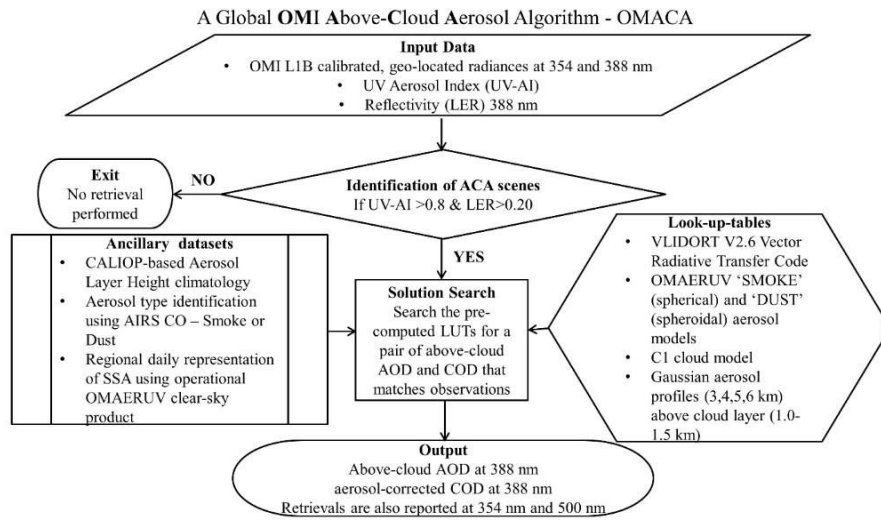
Figure 3 A General flowchart of the OMACA algorithm.
