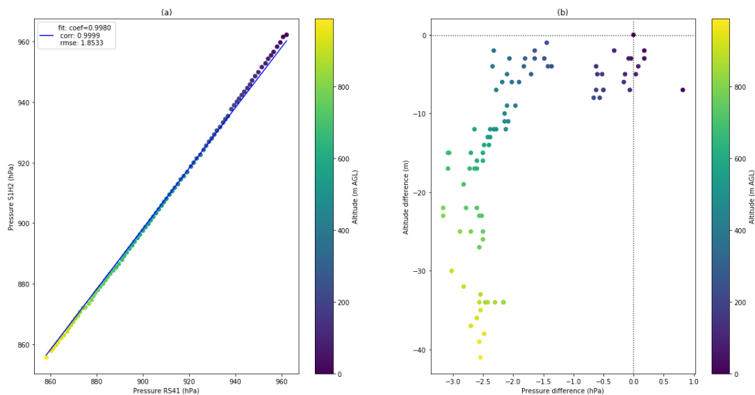
Figure 7 Comparison of pressure recorded by the Windsond S1H2 and calculated by the Vaisala MW41 (a), the pressure difference between the recorded Windsond S1H2 and the Vaisala RS41-SG (b) during the flight of the 28/06/2016 05:44 in Kumasi. The colors are based on the Vaisala RS41-SG measured altitude with the maximum altitude set to 1000 m.
