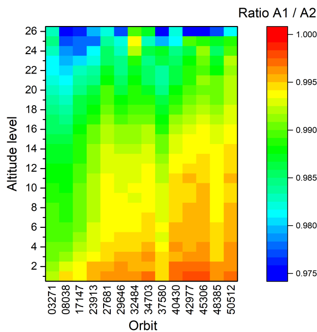
Figure 12. Ratio of calibrated spectra of channel A1 and A2.
