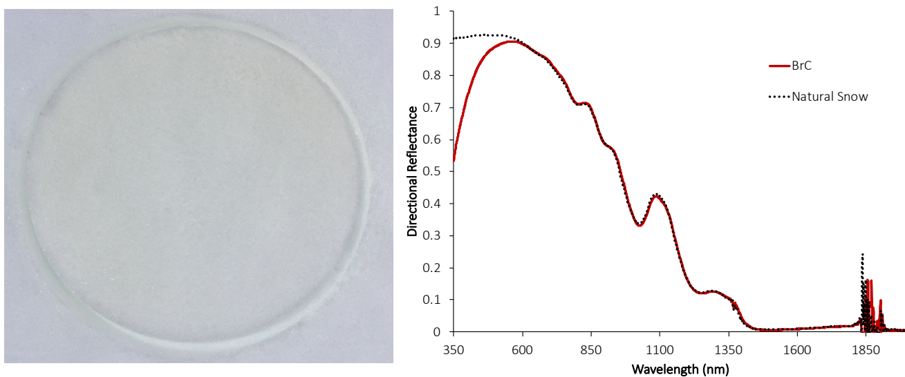
Figure 6: Image and HCRF spectra for a BrC deposition and adjacent natural snow in May of 2017 at the Tamarack Lake site. This BrC deposition drastically reduced the high natural snow reflectivity in the ultraviolet and short-wavelength visible (< 500 nm) spectral regions. Solar zenith: 34.6°; solar azimuth: 235.0°.
