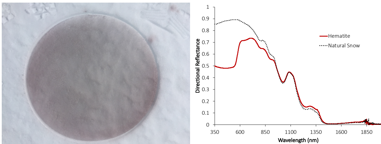
Figure 7: Image and HCRF spectra for a hematite deposition and adjacent natural snow in May of 2016 at the CUES research site. This hematite deposition drastically reduced the high natural snow reflectivity in the ultraviolet and short-wavelength visible ( < 600 nm) spectral regions. Solar zenith: 26.7^\circ ; solar azimuth: 167.6^\circ .
