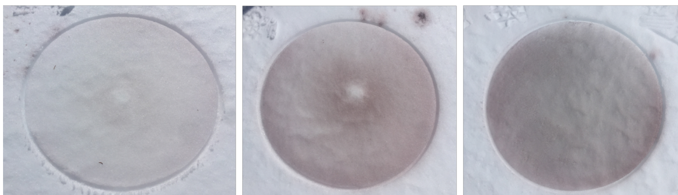
Figure 4: Images of three hematite depositions allow for visual inspection of the deposition uniformity. The left and center panels represent a previous apparatus design which featured a fan mounted inside the deposition chamber, which created less-uniform depositions. The right panel represents a hematite deposition using the final configuration of the apparatus.
