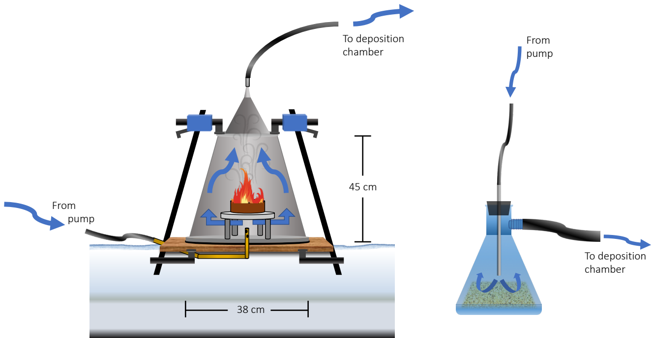
Figure 1: A battery-powered pump provided combustion and transport air into the aerosol production chamber for combustion aerosol (left), which flows to the deposition chamber at a flow rate of \sim 5.3 LPM. A 1-liter glass Buchner flask was used as the entrainment chamber for dry, pulverized dusts (right), which was provided short, quick bursts of air from a positive-displacement piston pump. The schematics are not drawn to scale.
