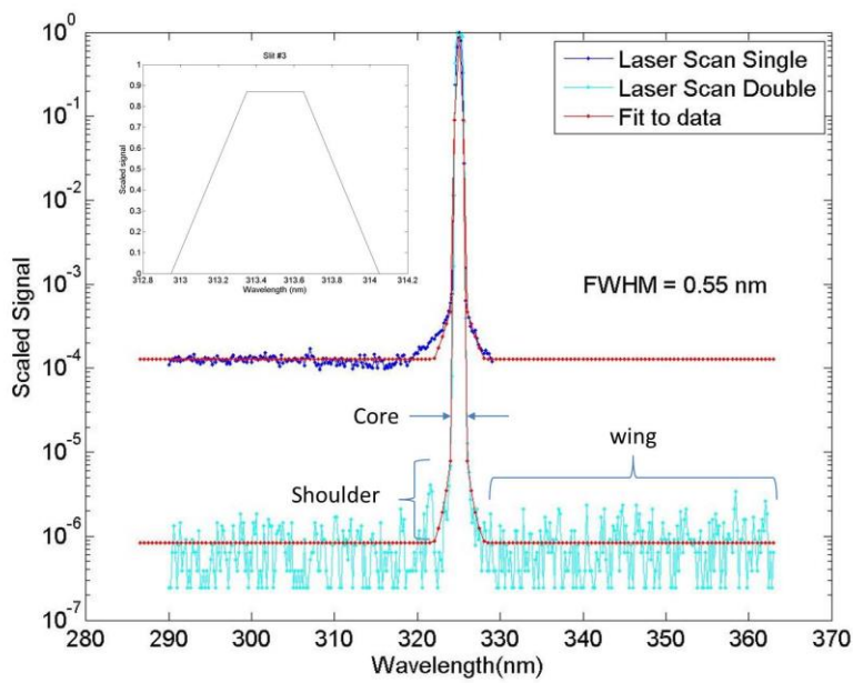
Figure 1: Slit functions measured with a He-Cd laser for single #009 and double #119 Brewers at Mauna Loa as well as fitted models; The ideal slit function is also shown inside the main graph.
