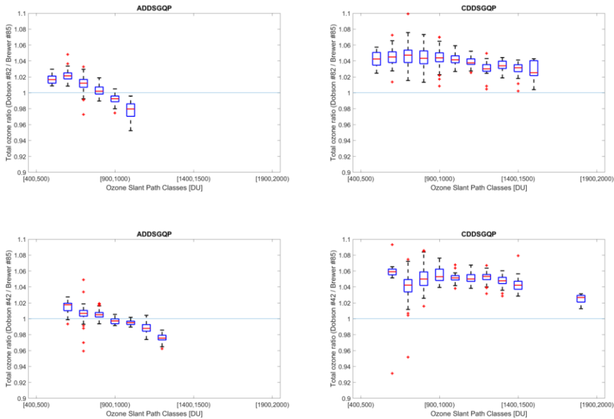
10 Figure 11: The ratio of quasi-simultaneous direct sun observations (within 5 min) by Dobsons #82 and #42, AD and CD wavelengths to data from double Brewer #085 at the South Pole for total ozone values larger than 220 DU . On each box, the central red line is the median, the edges of the box are the 25th and 75th percentiles, the whiskers extend to the most extreme data points not considered outliers, and outliers are plotted individually. In each bin the values with differences larger than three standard deviations from the mean of the bin have been removed from the calculation. Note that only bins with more than 6 simultaneous measurements are 15 depicted. The title of plots is showing the type of measurements. ADDSGQP: AD direct sun measurement using a ground quartz plate, and CDDSGQP: CD direct sun measurement using ground quartz plate.
