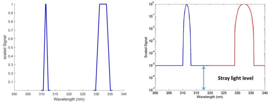
Figure 3: Dobson C-pair ideal slit functions (Left) parameterised from Figure 1 of Komhyr 1993. Dobson Modelled slit functions (right). Two straight lines have been added to the core slit functions in order to account for stray light.
