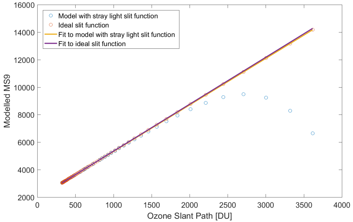
10 Figure 5: Example of Langley plot fitted to a modelled single Brewer data (see text for the details).
