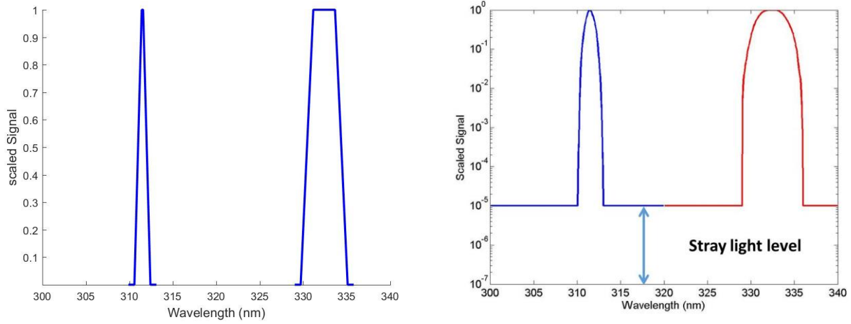
15 Figure 3: Dobson C-pair ideal slit functions (Left) parameterised from Figure 1 of Komhyr 1993. Dobson Modelled slit functions (right). Two straight lines have been added to the core slit functions in order to account for stray light.
