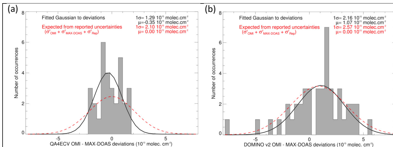
Figure 14. (a) Histogram of differences of QA4ECV OMI vs. MAX-DOAS tropospheric \text{NO}_2 columns for Tai'an (China) in May-June 2006. The black line shows a Gaussian fit to the observed differences, and the red dashed lines shows the Gaussian expected from the uncertainties reported in the QA4ECV and MAX-DOAS data products. (b) Same as (a), but now for differences between DOMINO v2 vs. MAX-DOAS tropospheric \text{NO}_2 .
