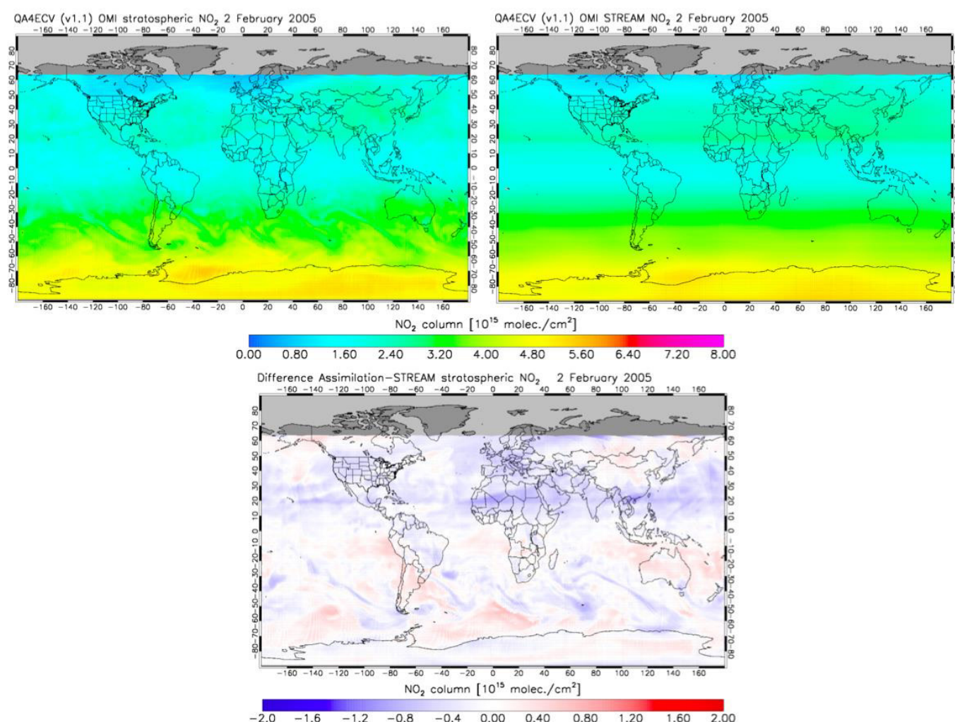
Figure 6. Stratospheric \text{NO}_2 columns from OMI on 2 February 2005, estimated with the data
