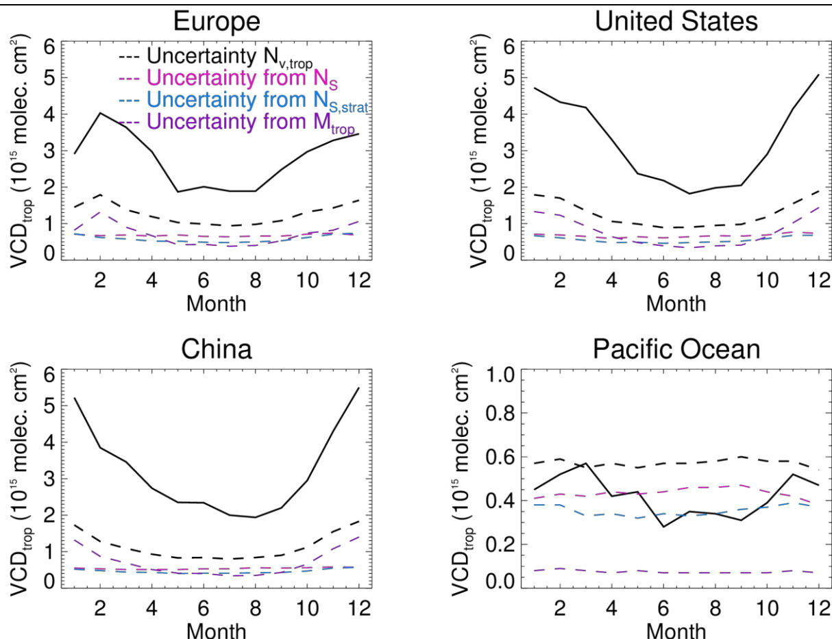
Figure 10. Average (single-pixel equivalent) QA4ECV OMI tropospheric NO 2 columns (solid line) and associated total uncertainties (dashed black line) for Europe (40–50°N, 10°W–15°E), United States (35–45°N, 100–75°W), eastern China (30–45°N, 110–140°E), and the Pacific Ocean (35–45°N, 160–140°W) in 2005. The dashed coloured lined indicate the contributions to the tropospheric NO 2 column uncertainty from SCD (pink, (\frac{\sigma_{N_S}}{M_{tr}}) ), stratospheric correction (light blue, (\frac{\sigma_{N_{S, strat}}}{M_{tr}}) ), and the tropospheric AMF (purple, (\frac{(N_S - N_{S, strat})\sigma_{M_{tr}}}{M_{tr}^2}) ).
