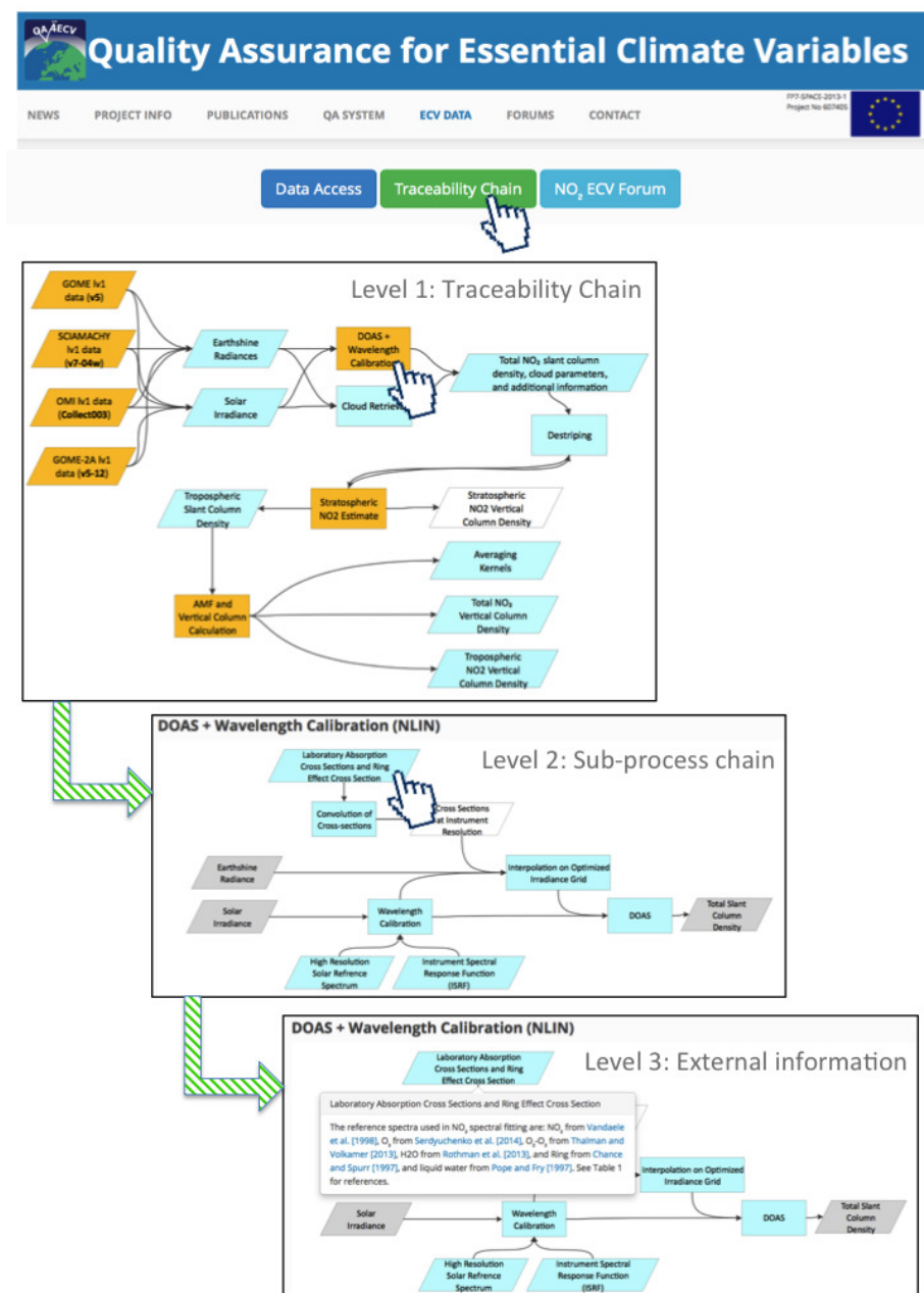
Figure 3. Traceability Chain for the QA4ECV NO 2 retrieval algorithm. The orange blocks (rectangles) are the building blocks of the retrieval, and in the main chain these are clickable to see more details in deeper layers. The light blue blocks are also clickable and will provide more information on that process in a pop-up window. The parallelograms provide information on algorithm choices and input data sets. The interactive traceability chain is available at: http://www.qa4ecv.eu/ecv/no2-pre .
