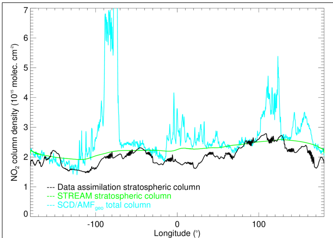
Figure 8. Meridional average QA4ECV OMI NO 2 column averaged over 39-41°N on 2 February 2005. No cloud radiance, albedo, or AMF filtering has been applied. Data assimilation and STREAM stratospheric columns are indicated in the black and green lines, the total slant columns divided by the geometric AMF is light blue. Both data assimilation and STREAM stratospheric column estimates are included in the QA4ECV NO 2 product.
