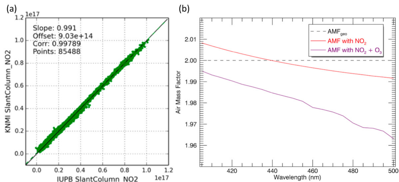
Figure 5. (a) Correlation plots of IUP Bremen (425-497 nm fitting window) and KNMI (405-465 nm) NO 2 slant columns retrieved using preferred fit settings for OMI orbit OMIL2_2005m0202t0339, including only pixels with SZA < 88° and intensity < 1.1×10 14 . (b) Wavelength dependency of the total air mass factor for a scenario with SZA=VZA=0° (geometrical AMF = 2), as calculated with DAK for a mid-latitude standard atmospheric profile with a total NO 2 column of 5.9×10 15 molecules cm -2 (mostly situated in the stratosphere) (red curve), and for the same mid-latitude standard atmospheric profile but now with absorption by both NO 2 and O 3 (total column of 322 DU, purple curve).
