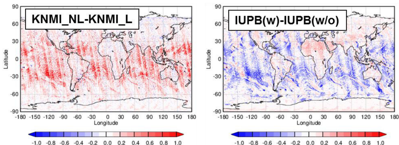
Figure 4. OMI NO 2 slant column differences between KNMI intensity (KNMI_NL) and optical density fit (KNMI_L) and IUPB fit including (IUPB(w)) and excluding the intensity offset (IUPB(w/o))(right). Data from 2 February 2005.
