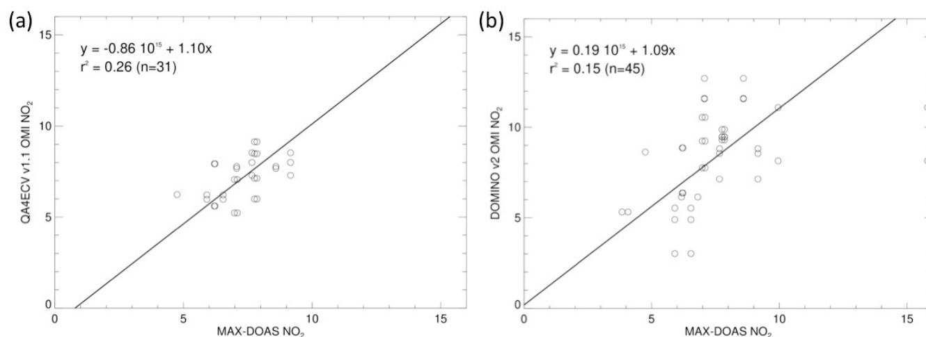
Figure 13. (a) Scatterplot of QA4ECV OMI vs. MAX-DOAS tropospheric \text{NO}_2 columns for Tai'an (China) in May-June 2006. The solid line shows the result of a reduced major axis regression to the data. Only pixels measured a cloud radiance fraction < 0.5 and an effective cloud pressure <850 \text{ hPa} , within 20 km and 30 minutes of a MAX-DOAS measurement have been selected. (b) Same as (a), but now for DOMINO v2 vs. MAX-DOAS tropospheric \text{NO}_2 .
