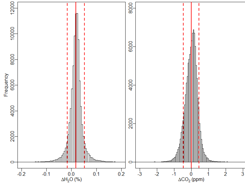
Figure 9. Histogram of difference between H_2O and CO_2 mixing ratios from FCHAOS and the Picarro G2301-f. FCHAOS CO_2 has been calibrated, while H_2O has not. For H_2O , mean of 0.018% or 180 ppm, median of 0.018% or 180 ppm, 1\sigma of 0.034% or 340 ppm, where Picarro G2301-f precision is 100 ppm. For CO_2 , mean of 0 ppm, median of 0.024 ppm, 1\sigma of 0.45 ppm.
