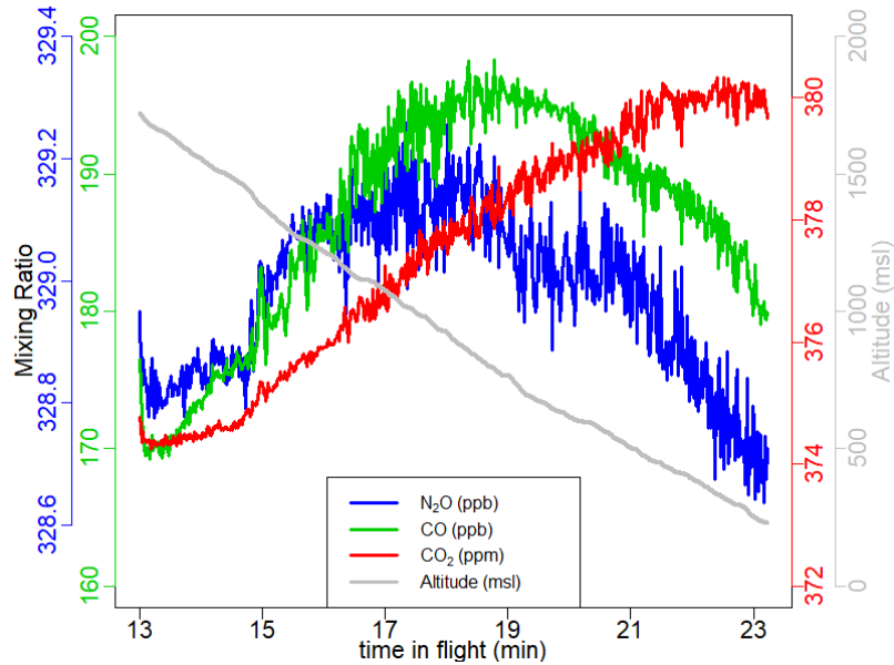
Figure 4. A null test demonstrates artifacts when operating the instrument in an off-the-shelf manner. Drift occurs in \text{N}_2\text{O} , \text{CO}_2 , and CO due to changes in cabin pressure that occur with changing aircraft altitude.
