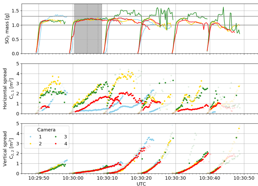
Figure 11. Total mass, horizontal spread and vertical spread (lower panel) of six subsequent puffs. Only data from cameras 1-4 are shown due to significant cloud signals in camera 5 and 6. The background images, and thus cloud cover, were reconstructed from the shaded time period. The shaded data points are discarded because their corresponding mass lies outside the expected range (1.0-1.3 g).
