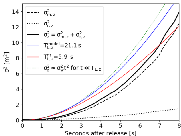
Figure 14. Absolute dispersion in the vertical (solid black line). Relative dispersion and meandering are shown with dotted and dashed black lines, respectively. Two parametrisations of Taylor’s theorem are plotted: 1) modelled from the sonic anemometer data (blue) and fitted to the measured absolute dispersion (red). For dispersion times much smaller than the Lagrangian time scale, the absolute dispersion can be approximated by a t^2 -dependency (green).
