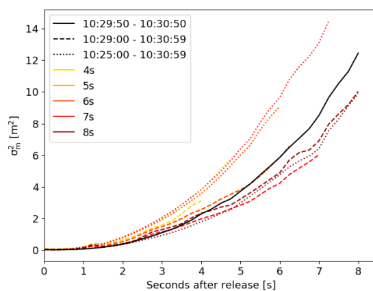
Figure 12. Meandering in the vertical. The black curve shows the ensemble average over the six puffs. The meandering is sensitive to the chosen ensemble. The coloured dashed and dotted curves show the meandering calculated for different numbers of puffs, selected by varying the time interval (line style) and the minimum trajectory lengths (colour).
