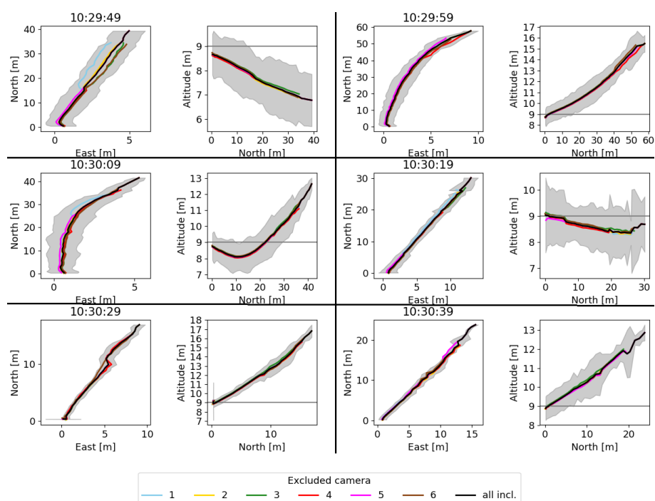
Figure A3. Sensitivity of the reconstructed trajectories to the removal of data from a single camera. The trajectory colour indicates which camera was removed from the calculation, the black trajectory is based on data from all cameras. The time indicates the release time of the puff. In the altitude-north plots, the horizontal line represents the release altitude.
