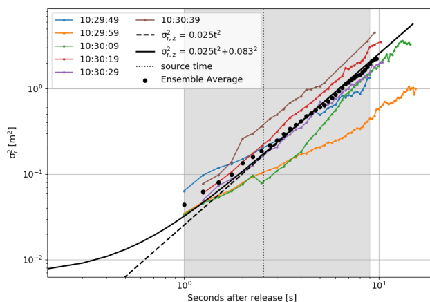
Figure 13. Relative dispersion in the vertical on a log-log-scale. The coloured curves show the dispersion of individual puffs and the black points show the ensemble average over these individual puffs. The source size was estimated by a linear fit to the ensemble average (dashed black line). The resulting source size was used to calculate the predicted curve by Eq. (4) (solid line) and estimate the source time (dotted black line).
