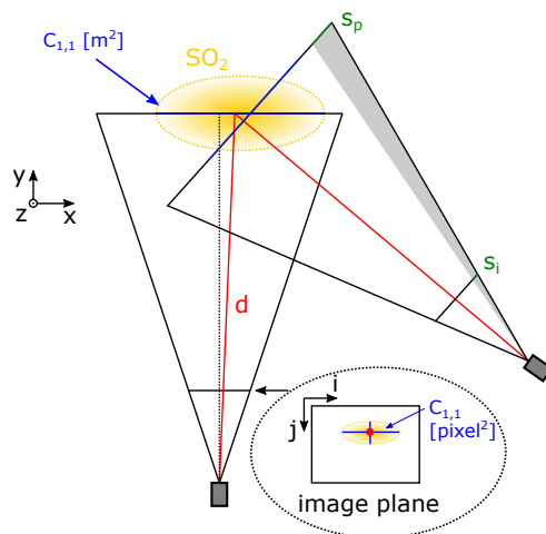
Figure 5. Sketch of the field of view of two cameras from above. The three-dimensional \text{SO}_2 puff (yellow) in the world coordinate system (x,y,z) is projected to the two-dimensional image plane (i,j) . The centre of mass in the image plane corresponds to a solid angle in the world coordinate system (red). The apparent size of a pixel scales with the distance to the object plane (grey area).
