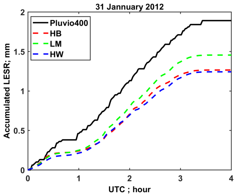
Figure 10: Comparison of liquid equivalent accumulations computed using HB, LM, and HW methods, respectively, based on 2DVD measurements and that directly measured by the collocated Pluvio snow gauge. We used the total accumulation to estimate the PSD adjustment factor for the “LM” and “HW” methods.
