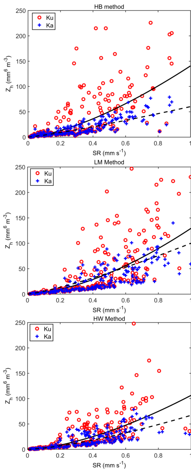
Figure 13: 2DVD derived Z_h versus 2DVD measured SR scatter plots, with Z-SR power-law fits, for Ku- and Ka-bands and “HB” method (top panel), “LM” method (central panel), and “HW” method (bottom panel).
