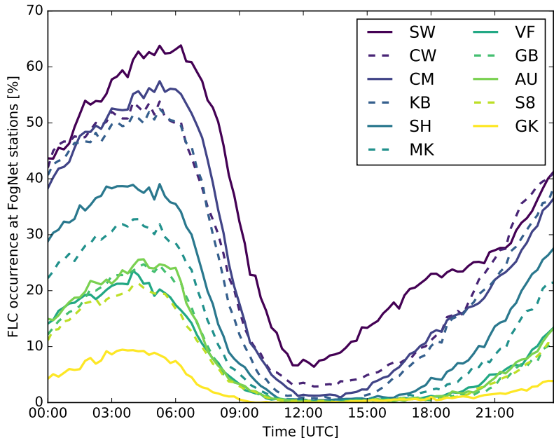
Figure 5. Average diurnal cycle of FLC occurrence at FogNet stations. Lines are colored by the longitudinal rank of each specific station, with coastal stations in dark colors and stations further inland in brighter colors. Every other line is dashed with the only purpose of helping their visual discrimination.
