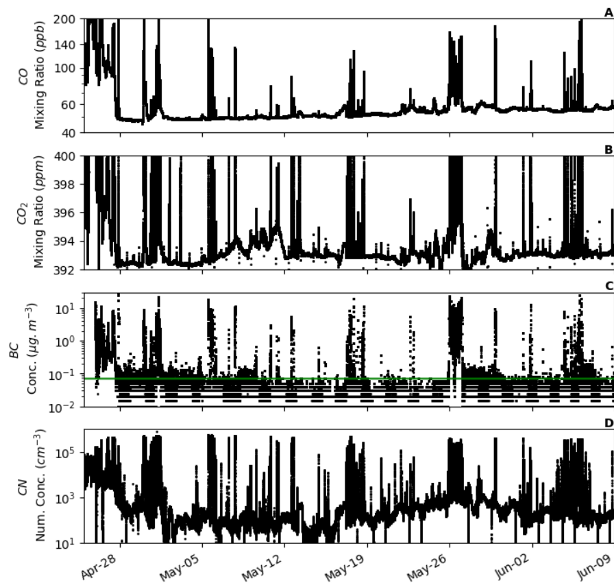
Figure A2. Time series (log scale) of CO, CO 2 , BC and CN for 45 days of voyage IN2016_V03 which traversed from the ice-edge to the equator along the 170°W meridian with a short personnel exchange port period in Wellington, New Zealand on the 26th May, 2016. The green line in Panel C represents the BC limit of 0.07 \mu\text{g}\cdot\text{m}^{-3} utilised. This dataset was utilised for the algorithm development as it exhibits influences from urban and background marine regions, by which differentiation from ship exhaust must be achieved.
