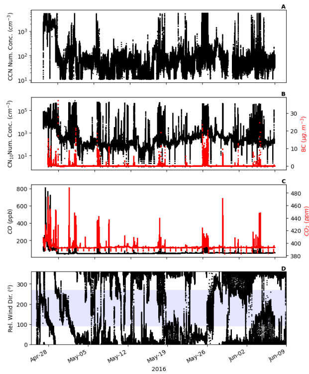
Figure A1. Time series showing that periods of CCN elevated above background values (typically less than 1000\text{ cm}^{-3} ) are associated with elevated concentrations of the other parameters, or wind directions in the exhaust sector. A) CCN B) CN (left) and BC (right) C) CO (left) and \text{CO}_2 (right) and D) relative wind direction with the coloured region signifying those directions exhaust is expected.
