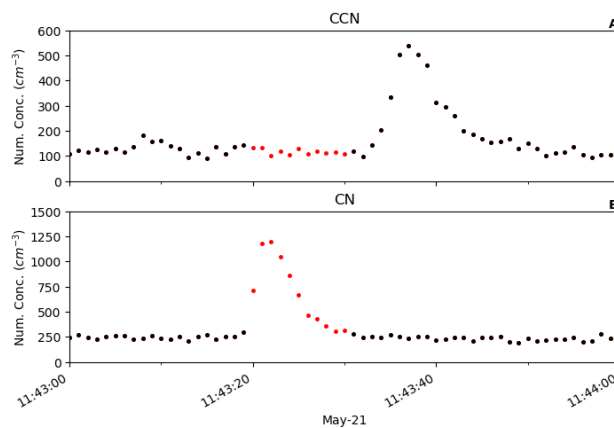
Figure A10. Time series of one minute of time-synchronised aerosol data. Unfiltered data in red, with black markers showing exhaust filtered data. The exhaust is clearly identified in the CN data but due to differences in instrument residence time, the exhaust signal shows up 10 seconds later in the CCN data, in this case, after the exhaust signal has ceased in the CN. While it is possible to align the underlying datasets based on an exhaust event, rather than by time, application of this method is unsuitable for this context because of the range of instrumentation where this exhaust product would be utilised (and thus the range of responses), and because the window filter applied after identification would result in a negligible improvement.
