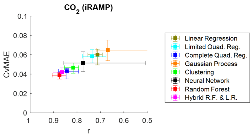
Figure S1. Results corresponding to Fig. 2 for CO 2 .
