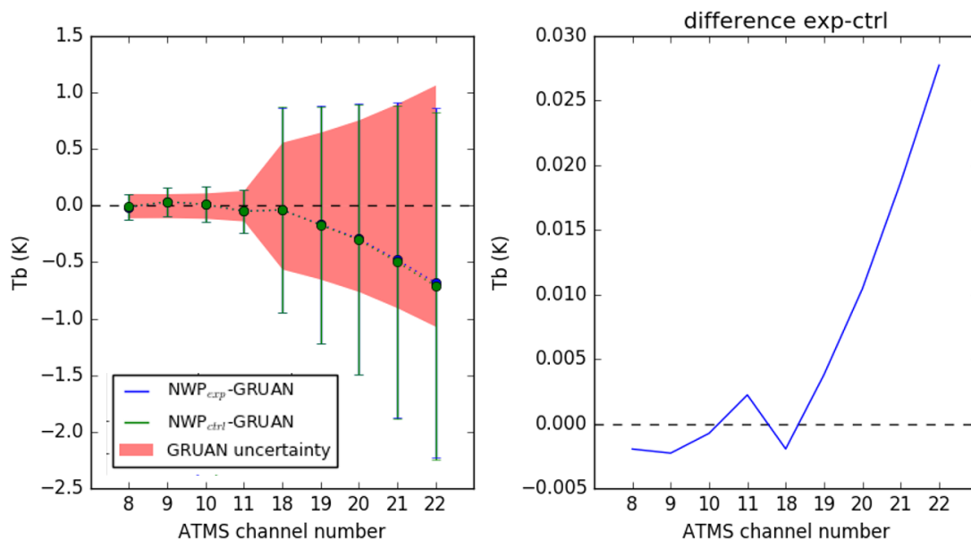
Fig. 1. Figure R1: (left) NWP-GRUAN simulated Tb at ATMS freq. using the MetOffice denial exp. (blue) and from control (green). (Right) difference between exp. and control.
