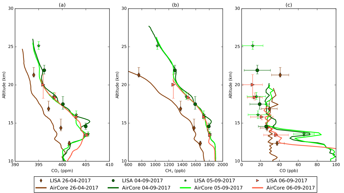
Figure 5: Comparison of AirCore and LISA measurements of (a) \text{CO}_2 , (b) \text{CH}_4 and (c) CO mole fractions. The AirCore CO profiles are averaged in 100 m bins to smooth the relatively large noise of the measurements due to the analytical precision of 7 ppb ( 1 \sigma ) of the CRDS analyser. Different colours and symbols are used to label the samples from different flights shown in the legend.
