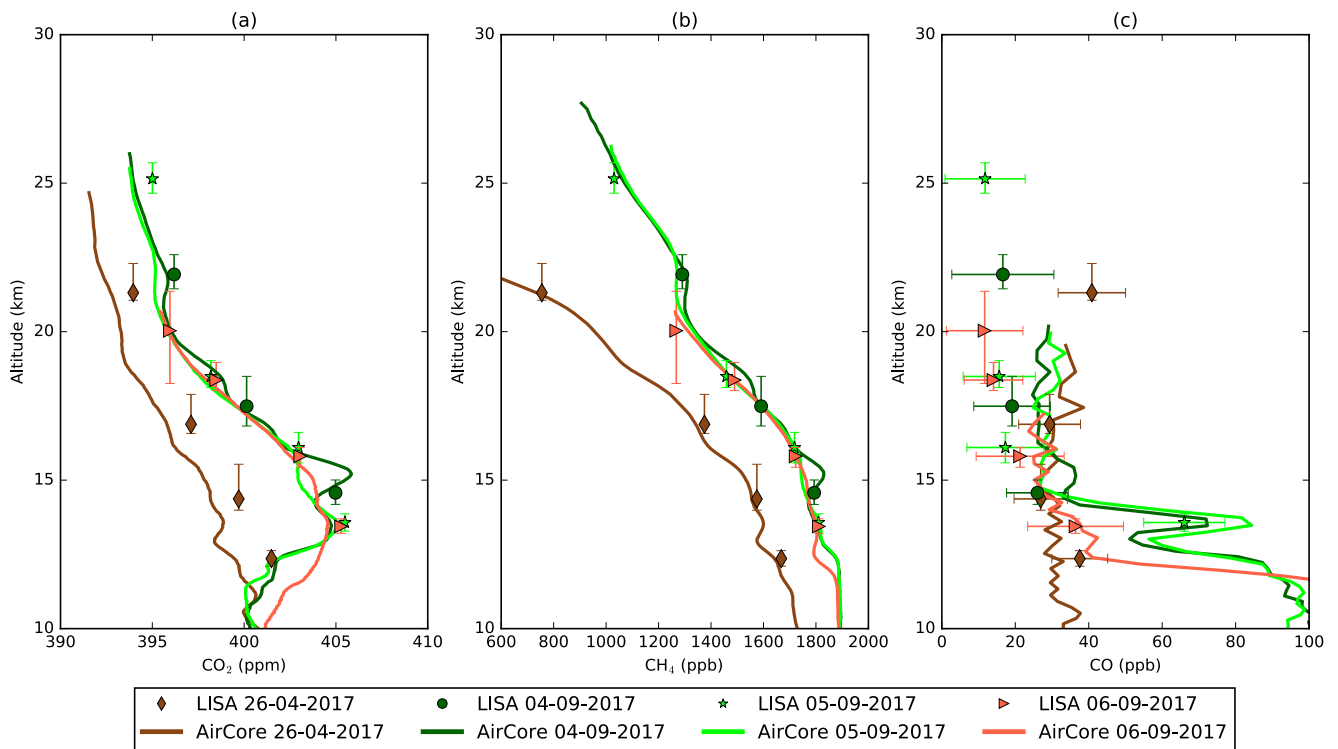
Figure 5: Comparison of AirCore and LISA measurements of (a) CO 2 , (b) CH 4 and (c) CO mole fractions. The AirCore CO profiles are averaged in 100 m bins to smooth the relatively large noise of the measurements due to the analytical precision of 7 ppb (1 \sigma ) of the CRDS analyser. Different colours and symbols are used to label the samples from different flights shown in the legend.
