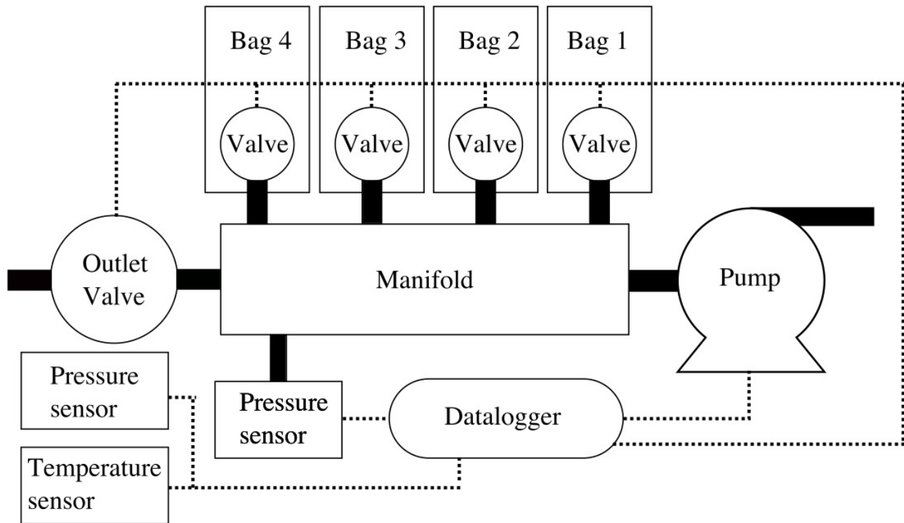
5 Figure 1: A schematic diagram of the sampler. Four bags are connected to a custom-made manifold. A small servomotor operates the screw cap combo valve. The outlet valve is the same as that of the bags, but is normally open when the sampler is idle during flight, allowing air pressure to equilibrate with outside air. Pressure inside the manifold is monitored by a pressure sensor. A datalogger is used to control all of the electronics. Electric connections are shown with dashed lines.
