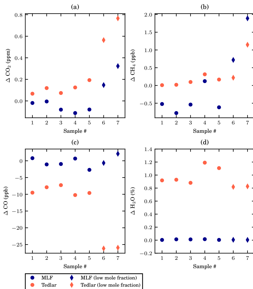
Figure 2. The observed drift of the mole fractions of CO 2 (a), CH 4 (b), CO (c) and H 2 O (d) in each of 7 samples in both Tedlar and MLF bags. The drift is defined as the difference between the measured mole fractions after 4 hours and those measured immediately after filling. For CO 2 , the mole fractions of samples nos. 1 – 5 are representative for stratospheric mole fractions. Samples nos. 6 & 7 contain low mole fractions and represent a typical mole fraction of stratospheric CH 4 .
