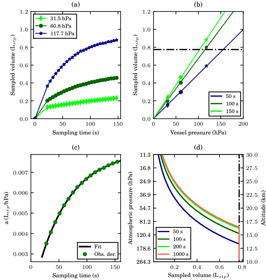
Figure 3. a) Sample volume as a function of the sampling time in seconds. The first 19.7 \pm 0.3 seconds fill the bag up to the pressure in the vessel. The sampled volume in the first 19.7 seconds linearly interpolated starting at zero, e.g. assuming that sampled volume increases linear with time. After the first 19.7 seconds, the bag is not expanding and air needs to be compressed and the flow rate drops. b) Sampled volume in litre at STP as a function of vessel pressure (markers correspond to those presented in 3a). The sampling time of 50 seconds, 100 seconds and 150 seconds are arbitrarily chosen. The lines are a linear fit to the data as in Equation 2. For a given sampling time, the sampled amount at STP decreases linear with vessel pressure. The bags cannot withstand a pressure difference larger than 300 hPa. The practical limit is presented with a black dashed line. c) The slope a(t) (Equation 2) as a function of sampling time. The data points are derived values of t from the pressure data (Obs. der. is observations-derived), and the black line is the applied fit to the data, according to Equation 3, with t_0=19.7 seconds. The fit constants can be found in Table 2. d) Atmospheric pressure on the left and corresponding altitude on the right, as a function of modelled sampled volume. Note that for atmospheric pressure >120 and <30 hPa, as well as for sampling time >150 the depicted model relies on extrapolation of the observations. The International Standard Atmosphere is used to link pressure and altitude. The cut-of at the sample size of 0.77 L_{stp} is due to the practical fill limit of 300 hPa which consequently means that the sampling time is less. The uncertainty in volume presented in a and b is 7.6 \text{ mL}_{stp} .
