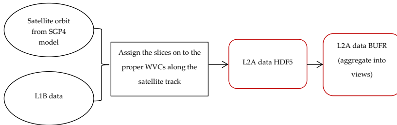
20 Figure 6: The workflow for generating LIB simulation data.
