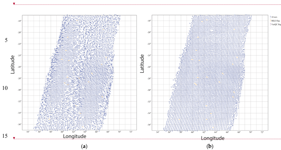
Figure 14: SCAT retrieved wind field. (a) 1 st rank solution; (b) 2DVAR result. The orange flags are artificial QC points and may be ignored.
