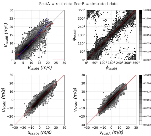
Figure 9: The collocation between SeaWinds (ScatA) and simulated SeaWinds (ScatB) in wind speed (upper left: red points are the average value as a function of wind speed of ScatA; blue points are the average value as a function of wind speed of ScatB), wind direction (upper right), u component (lower left), v component (lower right).
