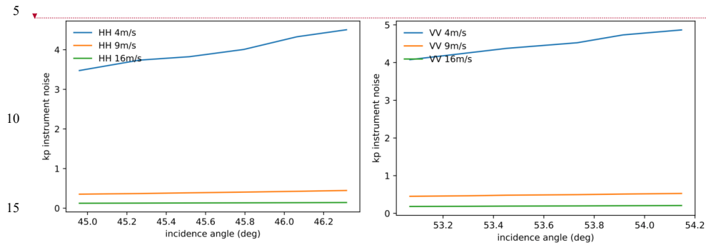
Figure 12: WindRad instrument noise in ratio (1 is 100%) at 4m/s, 9m/s, and 16 m/s on (a) slice level of Ku-band; (b) slice level of C-band (slices with SNR < 0.05 are excluded); (c) WVC mean Kp
