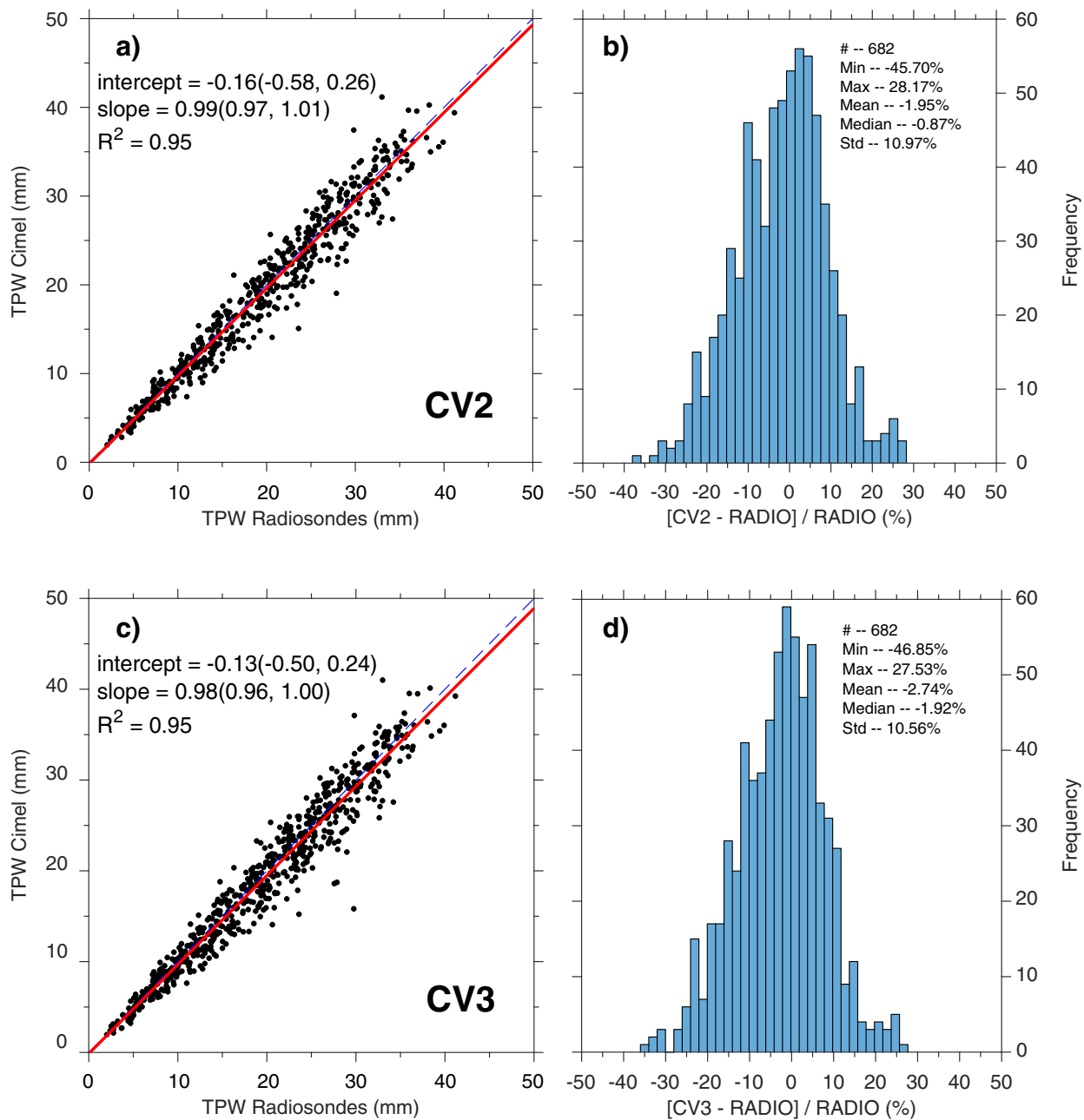
Figure 12. Scatter plot between the TPW from (a) the radiosondes-Ciel V2 and (c) Ciel V3. The red thick line shows the least square regression line and blue dashed line is the identity line. The regression coefficients are displayed along with their 95% confidence interval (in parenthesis). Frequency histogram of the relative difference between (b) the TPW from the radiosondes and CV2 and (d) CV3, respectively. The red line shows the fit of a normal distribution to the data.
