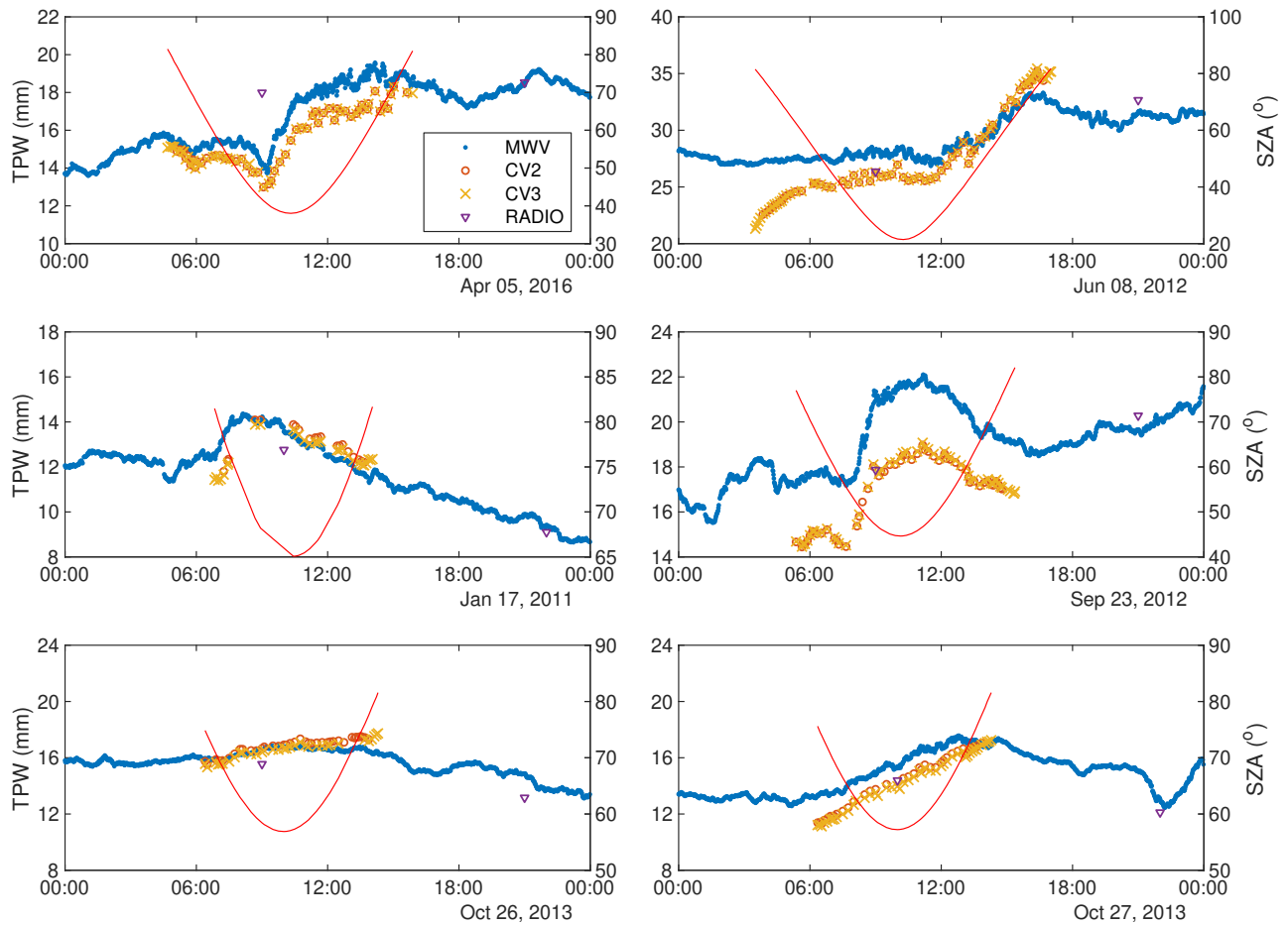
Figure 5. Diurnal variation of total precipitable water from radiosonde (magenta triangle), microwave radiometer (blue dots) and Ciel sun-photometer (V2 and V3 of the algorithm, red circle and orange cross, respectively) for six selected days (i.e., to cover all seasons and have a relative high number of Ciel measurements). The time is in UTC (i.e., local time + 2 hours). The red line indicate the range of the SZAs that Ciel measurements were performed.
