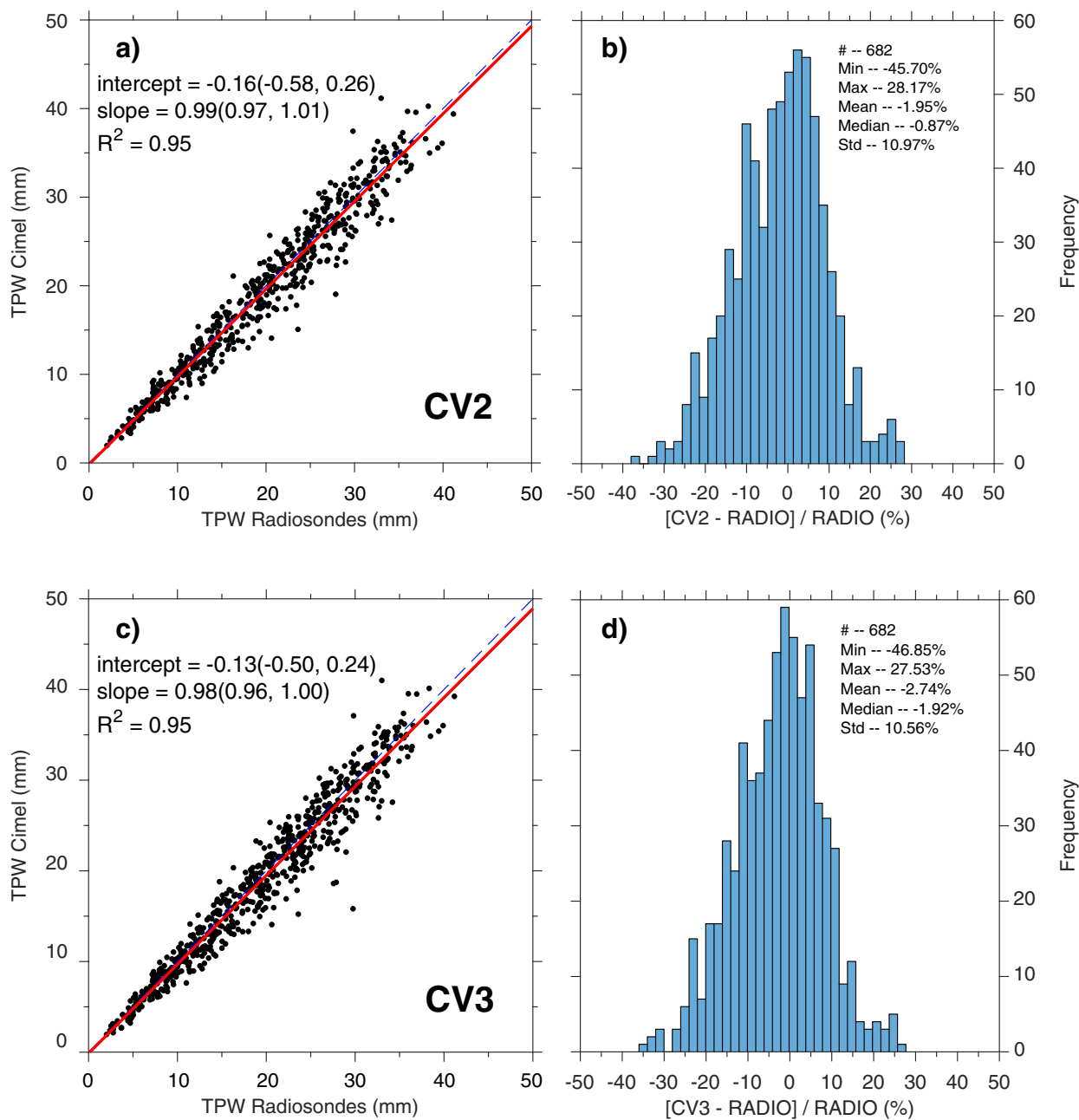
Figure 12. Scatter plot between the TPW from (a) the radiosondes-Cielmex V2 and (c) Cielmex V3. The red thick line shows the least square regression line and blue dashed line is the identity line. The regression coefficients are displayed along with their 95% confidence interval (in parenthesis). Frequency histogram of the relative difference between (b) the TPW from the radiosondes and CV2 and (d) CV3, respectively.
