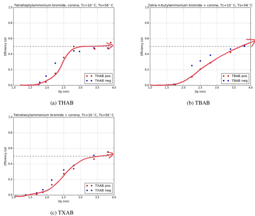
Figure 4. Efficiency curves measured for various laboratory-generated aerosols.
