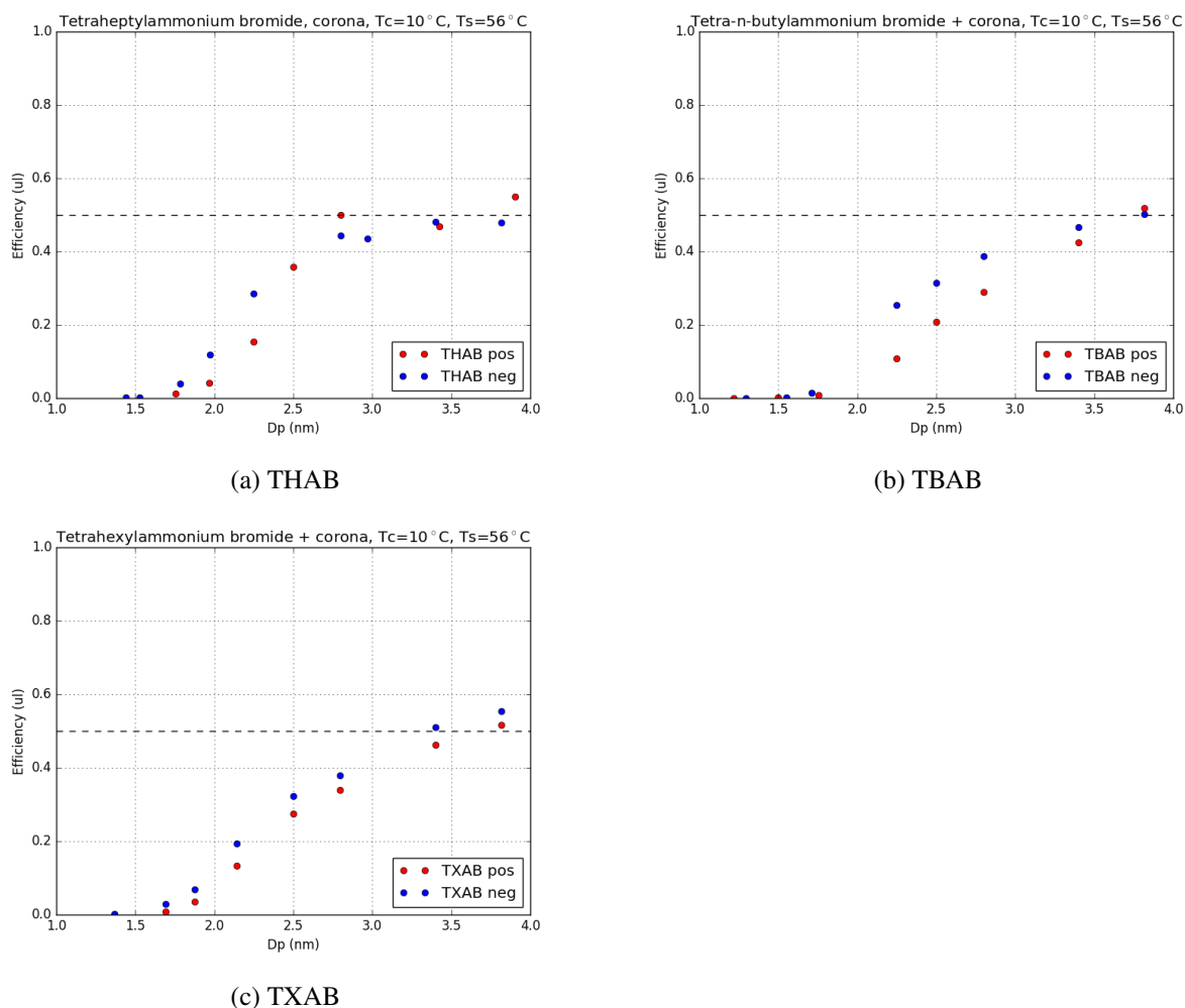
Figure 4. Efficiency curves measured for various laboratory-generated aerosols.
