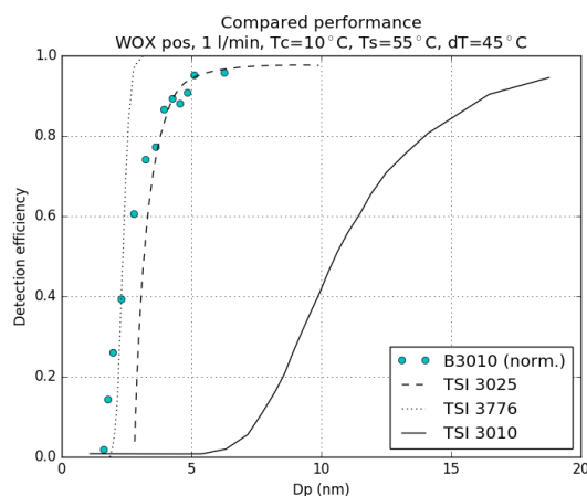
Figure 9. Gain in performance. Tungsten oxide particles. The data from TSI CPCs are taken from product brochures. The data from the B3010 are normalized.
