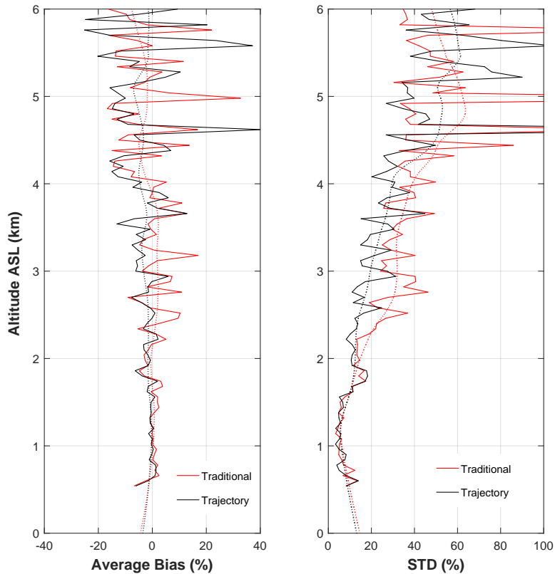
Figure 8. Left panel: The average bias between the radiosonde and the trajectory method calibrated profiles at 25 m vertical resolution for both the trajectory (black) and traditional methods (red). Dotted lines are further smoothed results using a running average of 75 m for both methods. Right panel: The standard deviation of all trajectory percent difference profiles at 25 m resolution for both trajectory (black) and traditional (red) methods. Dashed lines are the further smoothed results by a running average of 75 m for both methods.
