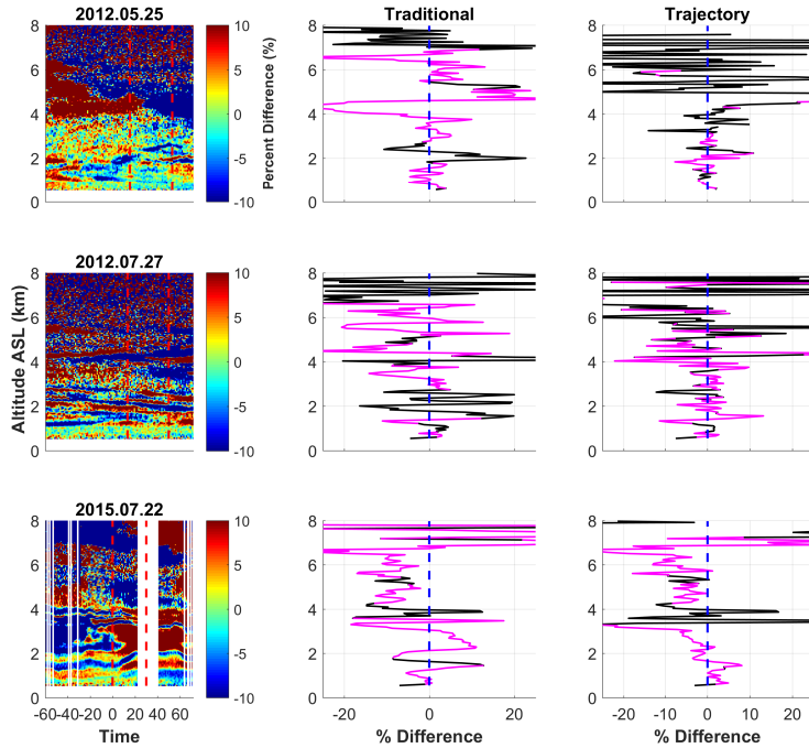
Figure 7. A subset of the dates with largely heterogeneous conditions showing the differences between the traditional and trajectory calibration techniques. This figure follows the same format as Fig. 6 and shows that when the water vapour field changes over the 30 min traditional calibration period, the traditional water vapour profile can look significantly different from the radiosonde. The trajectory method produces a profile with a smaller percent difference with respect to the radiosonde.
