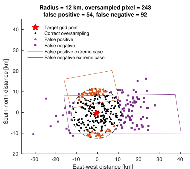
Figure 2. Centers of screened OMI pixels in 2005 over a target grid point (red star) near Denver, CO. OMI pixels are simplified as quadrilaterals provided by the 75FOV pixel edges from the OMPIXCOR product. Pixels that overlap with the target grid point with pixel center falling within the averaging radius (dashed circle) are plotted as black points (correct oversampling). Pixels that overlap with the target grid point with pixel center falling outside the averaging radius are plotted as purple squares (false negative). Pixels that do not overlap with the target grid point with pixel center falling in the averaging radius are plotted as red triangles (false positive). Extreme cases of false positive/negative are illustrated by OMI pixel quadrilaterals.
