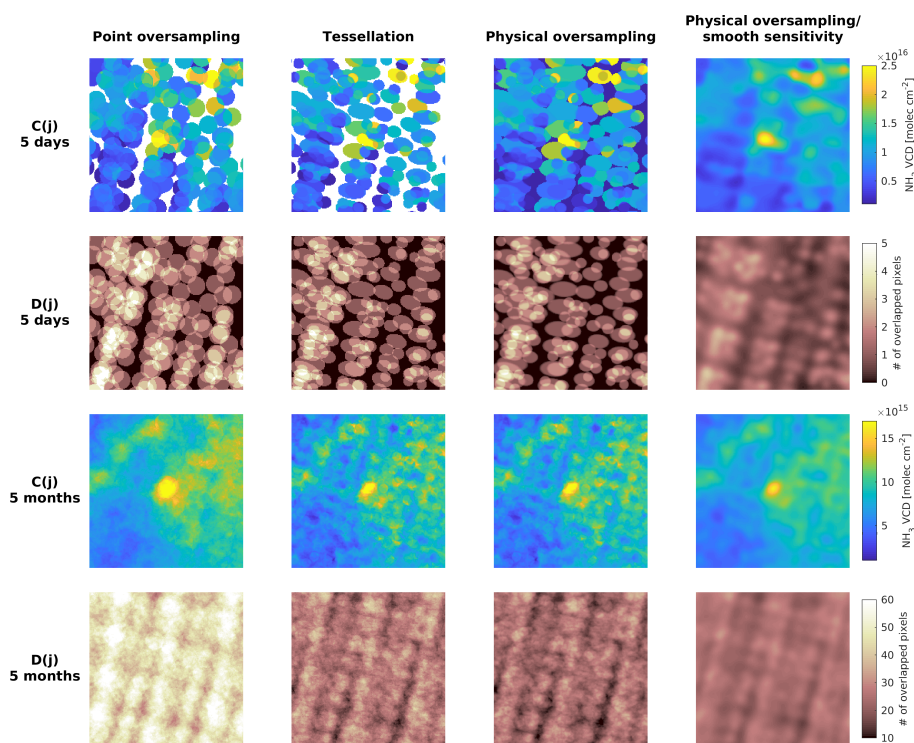
Figure 9. Similar to Fig. 8 using IASI \text{NH}_3 total column product for 2015. The drop-in-the-box approach is not included. Instead, the physical oversampling results using a smoother version of the IASI spatial response function are shown in the fourth column. The true IASI spatial response function has much sharper edges than OMI, such that the physical oversampling results (third column) are very similar to tessellation results (second column).
