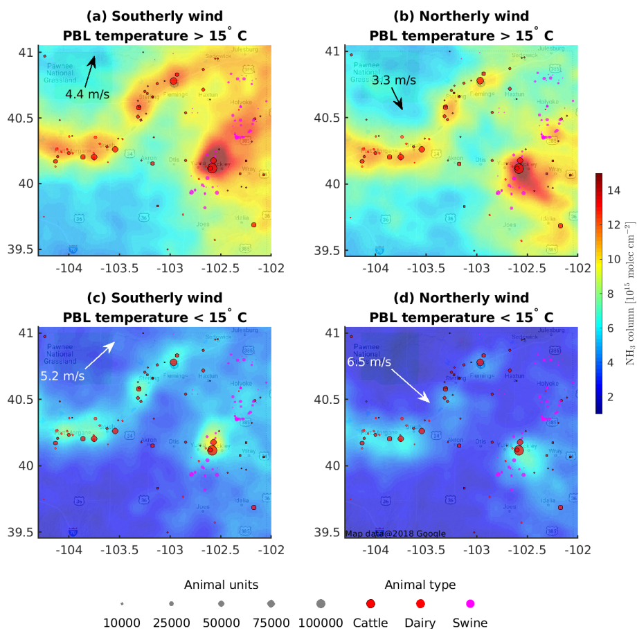
Figure 10. Physical oversampling results using IASI-A NH 3 total columns under southerly wind (a and c) and northerly wind (b and d) and high planetary boundary layer (PBL) temperature (> 15°C, a and b) and low PBL temperature (< 15°C, c and d). The text arrows show the average wind speed and wind direction at the locations/times of all IASI observations in each category. The size and location of large CAFOs are overlaid.
