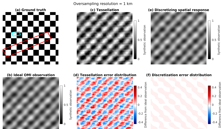
Figure 6. Oversampling a synthetic checkerboard pattern, shown in (a), at a spatial scale smaller than the OMI pixels to a grid resolution of 1 km. The ideal OMI observation in (b) is generated using spatial response function defined in Fig. 5 at very high resolution (0.05 km) and then coadded back to 1 km. (c) show the result from the tessellation method (assuming S(i, j) equals to the overlapping area between satellite pixel i and grid cell j ). (d) shows the difference between tessellation and the ideal observation. The values in (d) are equal to (c)–(b). (e–f) show the oversampling result by discretizing the spatial response function and its difference from the ideal observation. The values in (f) are equal to (e)–(b).
