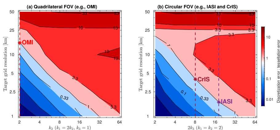
Figure 7. (a) The ratio between discretization/tessellation errors for different combinations of spatial response function shapes and target grid resolution. The unity contour line delineates the regime where tessellation error is larger than discretization error (blueish contours) and the regime where the discretization error is larger than tessellation error (reddish contours). The red vertical dashed line indicates the approximate spatial response for OMI. The red star marks the threshold resolution where the tessellation and discretization errors are equal for OMI. (b) Similar to (a) but the IASI pixel shapes and locations are used instead of OMI. The spatial response function exponents for CrIS and IASI and their intersects with the unity contour line are marked.
