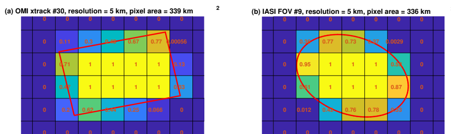
Figure 3. Tessellation process for OMI (a) and IASI (b) pixels. The IASI pixel is approximated by a 100-vertex polygon. Overlapping area ( S(i, j) ) between satellite pixel i and grid cell j is labeled at grid cell center, normalized by grid cell area ( 25 \text{ km}^2 ).
