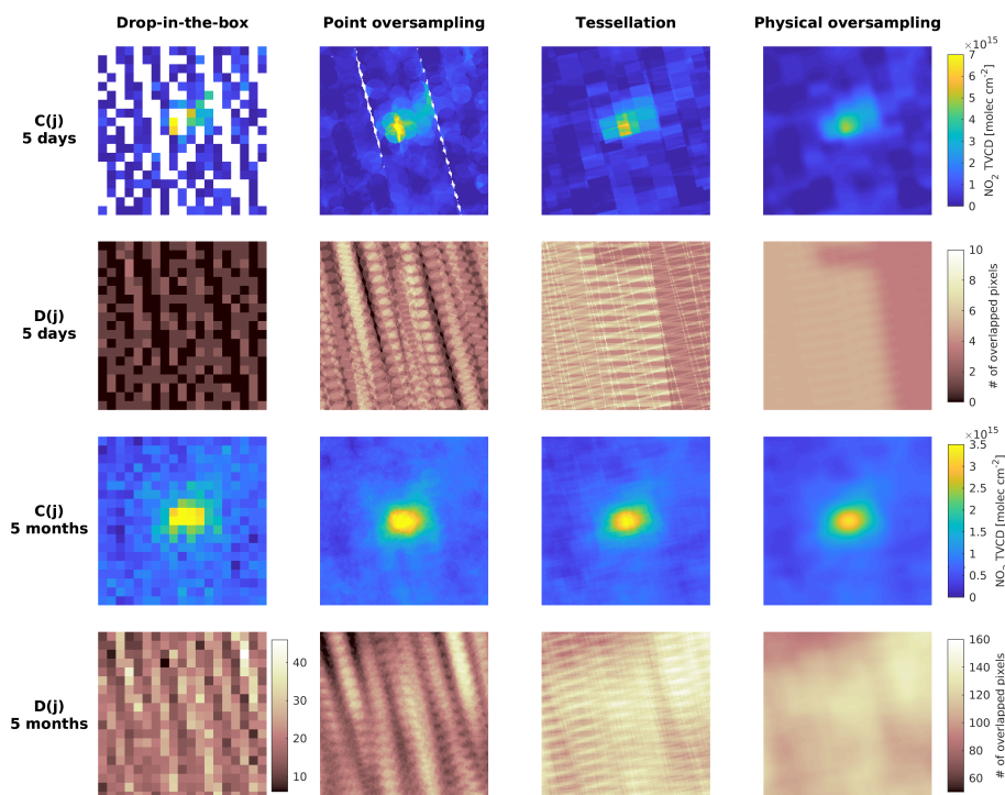
Figure 8. Level 3 results using drop-in-the-box method (10-km resolution, first column), point oversampling (averaging radius = 12 km, 1-km resolution, second column), tessellation (pixel corners from the OMPIXCOR product, 1-km resolution, third column), and physical oversampling (2-D super Gaussian with k_1 = 4 and k_2 = 2 , 1-km resolution, fourth column). The domain size is 200 \times 200 km. The first and third rows show the oversampled \text{NO}_2 TVCD for 5 days and 5 months, and the second and fourth rows show the corresponding numbers of OMI observations used in the averaging for each grid cell. Note the first panel in the fourth row is on a different color scale than the other panels in the same row.
