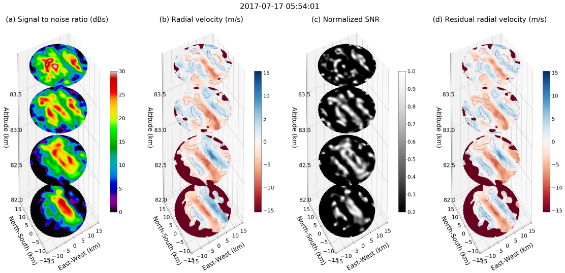
Figure 9. Same as 8, but at 05:54:01 on July 17, 2017 for altitudes: 82km, 82.7km, 83.4km, and 84km., i.e., Event 2.
