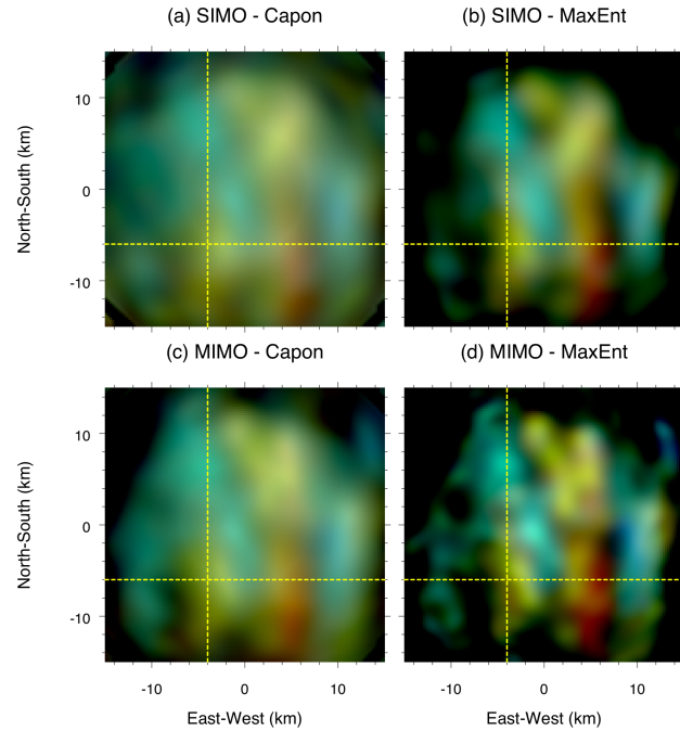
Figure 5. Same as Figure 3 but at 05:56:13 UT on July, 2017, i.e., Event 2. The yellow dashed horizontal/vertical lines represent the location of the NS/EW cuts shown in later figures for Event 2.
