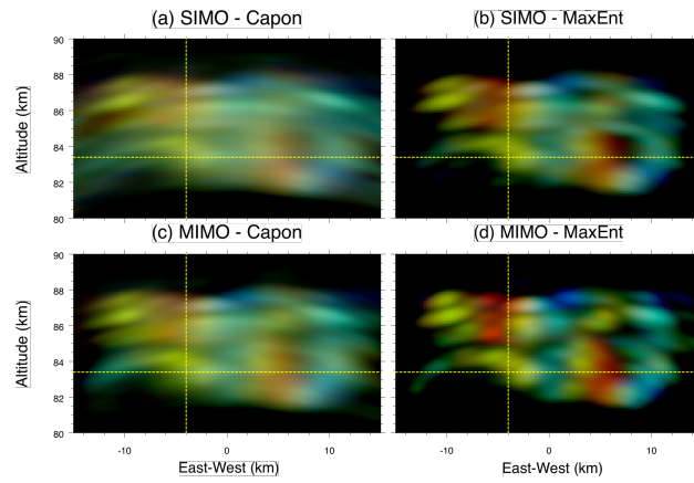
Figure 6. Same as Figure 5 but for an EW-Altitude cut at y = -6 km. The yellow dashed horizontal lines represent the location of the altitude cuts shown in previous and later figures for Event 2.
