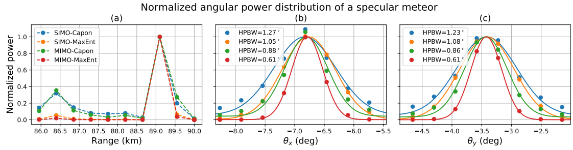
Figure 10. Normalized angular power distribution of a specular meteor echo as function of: (a) range, (b) EW angle ( \theta_x ), and NS angle ( \theta_y ). The results are shown for all four implementations, i.e., SIMO-Capon (blue), SIMO-MaxEnt (orange), MIMO-Capon (green), and MIMO-MaxEnt (red).
