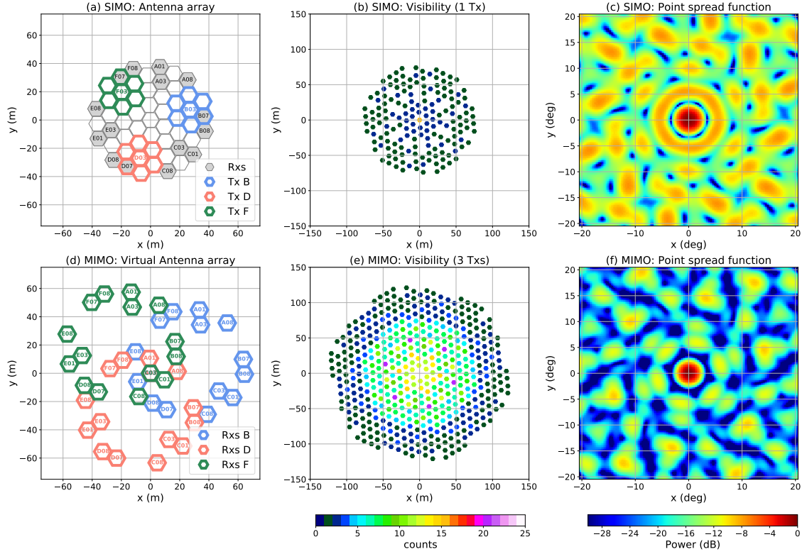
Figure 1. MAARSY antenna configuration for SIMO (first row) and MIMO (second row): (a) 16 hexagons used in reception are shown in grey and three anemones used in transmission are colored (b) visibility samples for SIMO (c) point-spread (or instrument) function for SIMO (d) the virtual position of the resulting receiving antennas by using MIMO (d) visibility samples for MIMO (e) point-spread (or instrument) function for MIMO. See text for further details.
