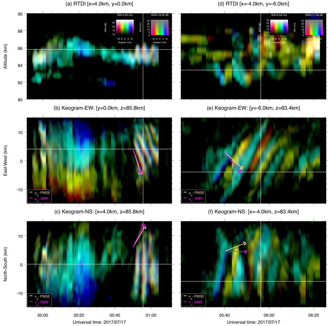
Figure 7. 24-bit time representation images of PMSE structures as function of: altitude (RTDI) (first row), EW location (Keogram) (second row), and NS location (Keogram) (third row) for selected cuts, for both Event 1 (first column) and Event 2 (second column). In the keograms, the wind components obtained with specular meteor radars (SMRs) and MAARSY PMSE are shown with pink and yellow arrows, respectively. The white dashed horizontal lines represent the location of the altitude, EW and NS cuts shown in previous figures and current keograms for Event 1 and 2. The white dashed vertical lines represent the time of the cuts shown in previous figures.
