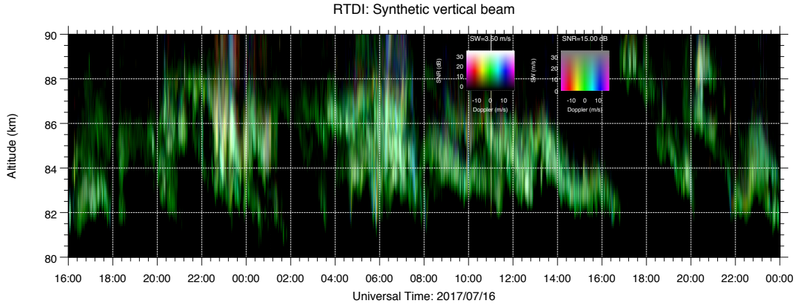
Figure 2. A 24-bit image of range-time Doppler intensity (RTDI) plot of PMSE using MIMO with time diversity conducted on July 16 and 17, 2017. The signal intensity is represented as lightness, Doppler information as hue, and spectral width as saturation. The legend on the left represent the SNR vs Doppler color map for a saturation of 90%. The legend on the right represents the spectral width vs Doppler for a lightness of 50%. Note that only the signal corresponding to the narrow region in the illuminated area is shown.
