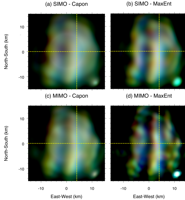
Figure 3. EW-NS images for z=85.8 km obtained from applying four different implementations (a) SIMO-Capon, (b) SIMO-MaxEnt, (c) MIMO-Capon, (d) MIMO-MaxEnt, at 00:56:55 UT on July 17, 2017, i.e., Event 1. Images are color coded as same as Figure 2. The yellow dashed horizontal/vertical lines represent the location of the NS/EW cuts shown in later figures for Event 1.
