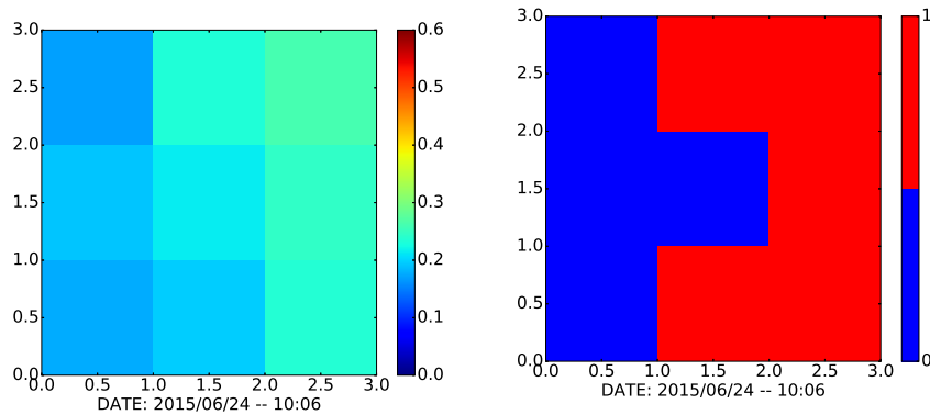
(b) Retrieved TOA BRF at 0.6 \mu\text{m} and binary cloud mask where 0 means cloud free and 1 by observation.
