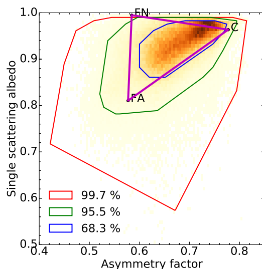
Fig. 4: Definition space for the wavelength 0.6\mu\text{m} defined by the non absorbing fine mode (FN), the absorbing fine mode (FA) and the coarse mode (C) vertices. The red, green and blue lines show respectively the 99.7%, 95% and 68% probability regions respectively, as derived from AERONET inversion product for all the observations available over all the AERONET stations.
