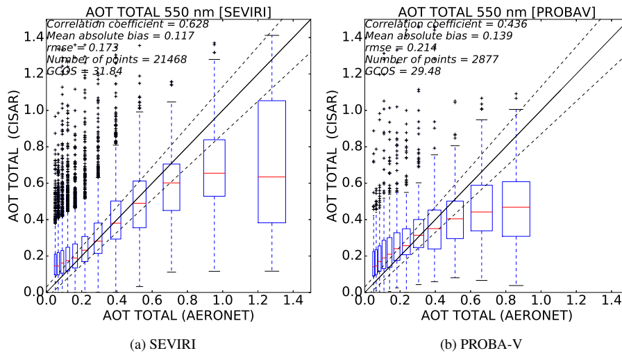
14: Boxplot between CISAR total AOT retrieval (extrapolated at 0.55 \mu\text{m} ) and the AERONET for both SEVIRI (left panel) and PROBA-V (right panel) over all the selected stations in 2015. Only retrieval with QI \geq 0.2 are considered. The blue boxes represent the interquartile range ( IQR ), the red horizontal line inside the blue boxes represents the median value, the vertical dashed bars represent the 1.5 * IQR range and the black crosses represent the outliers.
