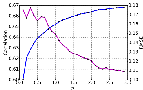
Fig. 11: Correlation (in purple) and RMSE (in blue) variations in function of the fit test p_3 . The figure refers to the CISAR AOT retrieval evaluation against AERONET data. The results are obtained from CISAR applied to SEVIRI observations.
