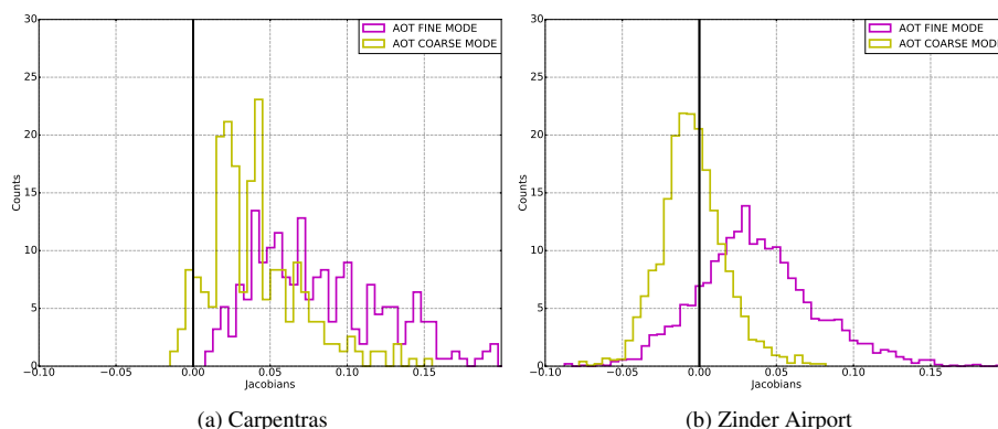
6: Distribution of the AOT Jacobian over Carpentras (dark surface) and Zinder Airport (bright surface). The histograms are obtained from PROBA-V observations (RED band) over year 2015.
