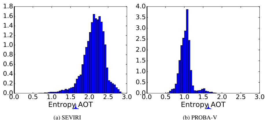
Fig. 9: Distribution of the entropy related to aerosols properties for SEVIRI (left panel) and PROBA-V (right panel) respectively.
