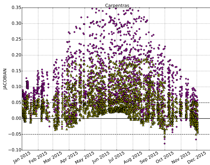
(a) SEVIRI
