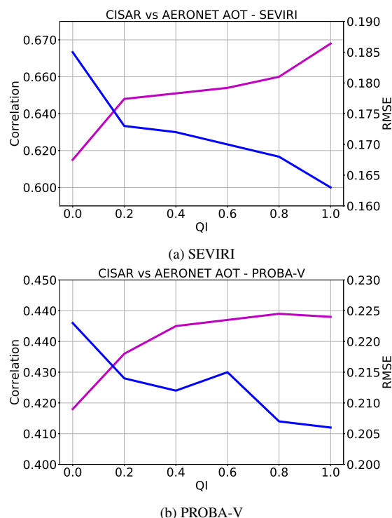
Figure 13: Correlation (in purple) and RMSE (in blue) variations in function of the QI. The figure refers to the CISAR AOT retrieval from SEVIRI (top panel) and PROBA-V (bottom panel) observations evaluated against AERONET data.
