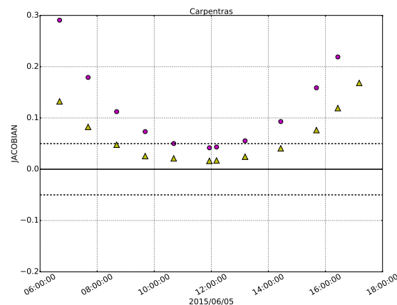
Fig. 8: AOT Jacobians associated to SEVIRI observation over Carpentras, France, for 2015/6/5. The purple dots represent the fine mode, the yellow triangles the coarse mode.
