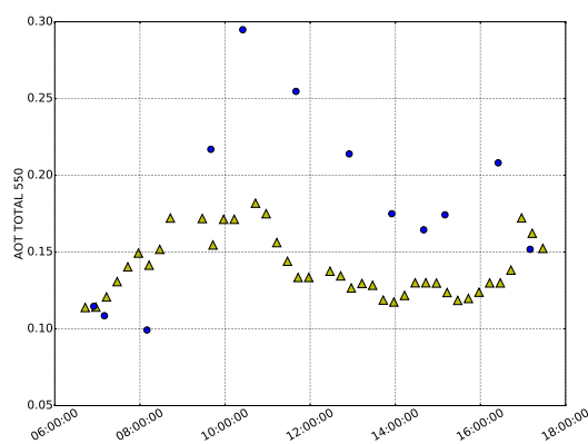
(a) CISAR (blue dots) and AERONET (yellow triangles) AOT series, showing a large overestimation of the retrieved values.
