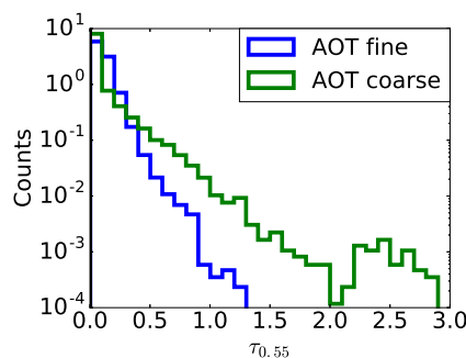
15: Fine (blue) and coarse (green) mode at 0.55 \mu\text{m} distributions from AERONET observations the selected stations (Table 1) over year 2015.
