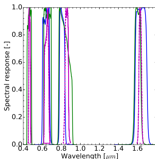
2: SEVIRI (in blue), PROBA-V (in green) and MODIS (in magenta) spectral responses.
