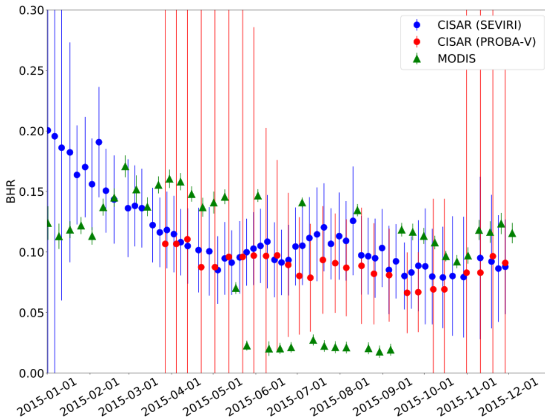
Fig. 3. BHR timeseries at 0.6 \mu m over Carpentras
